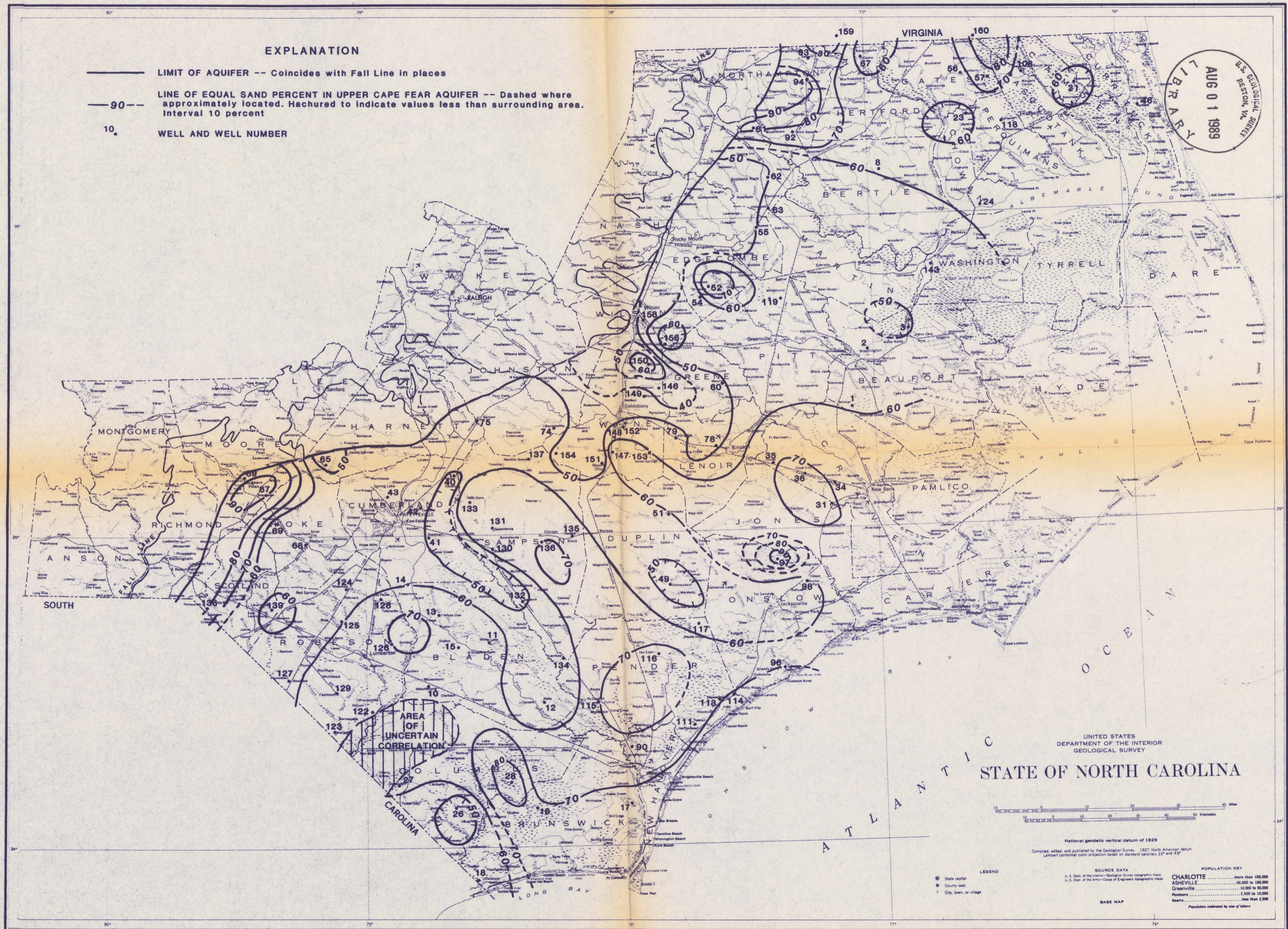
SAND PERCENTAGE IN THE UPPER CAPE FEAR AQUIFER
