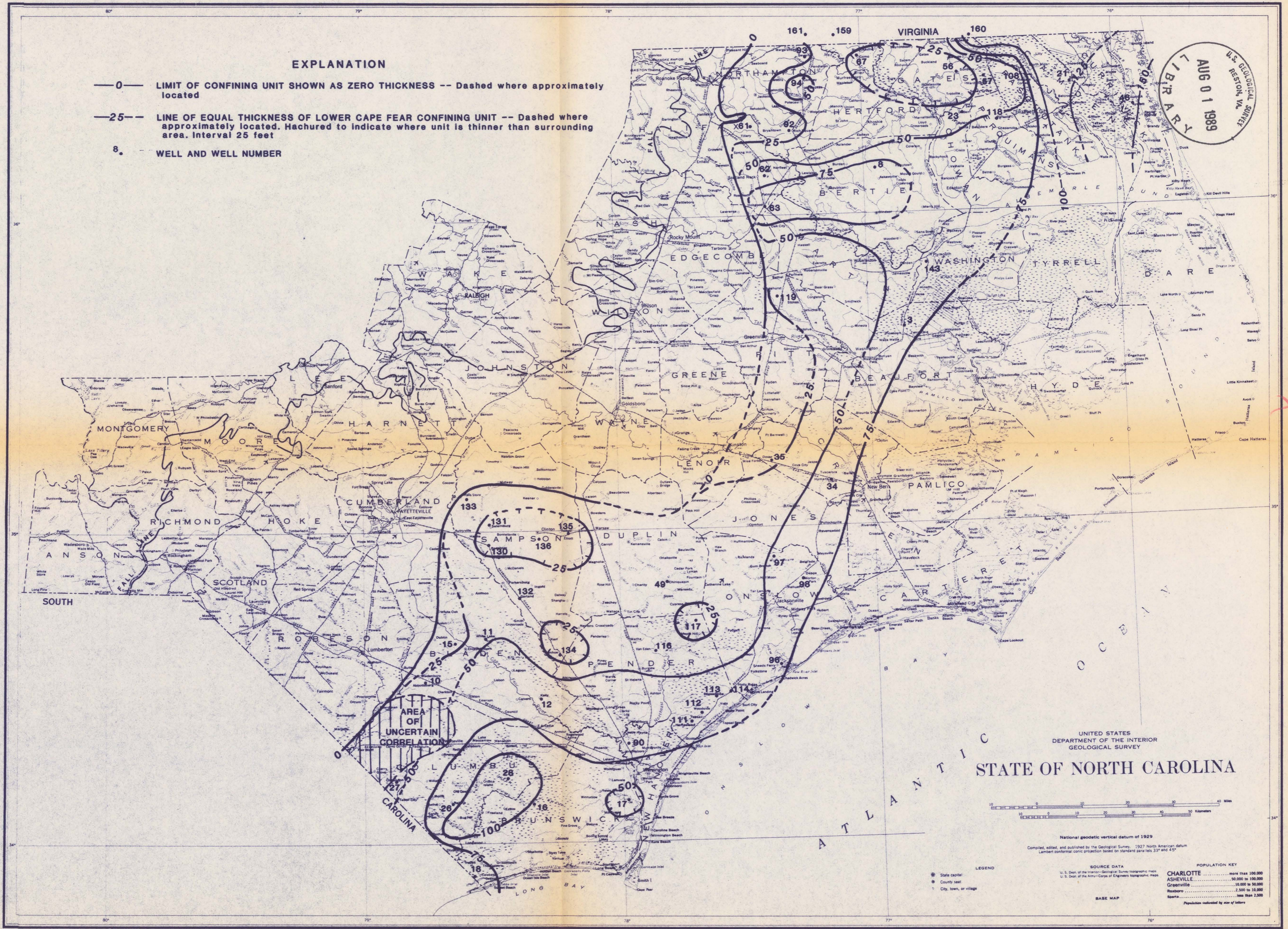
THICKNESS OF THE LOWER CAPE FEAR CONFINING UNIT
