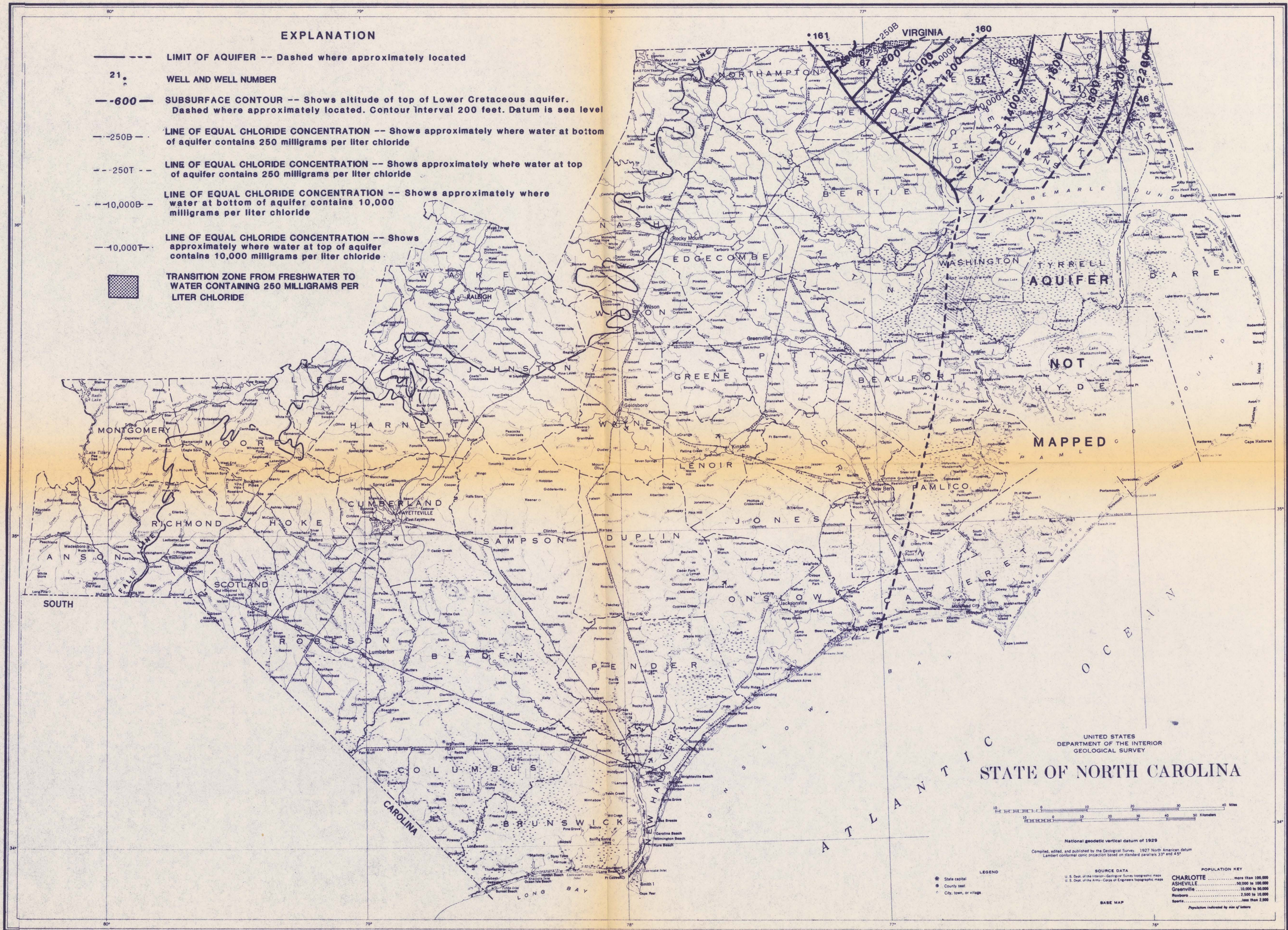
ALTITUDE OF THE TOP OF THE LOWER CRETACEOUS AQUIFER
