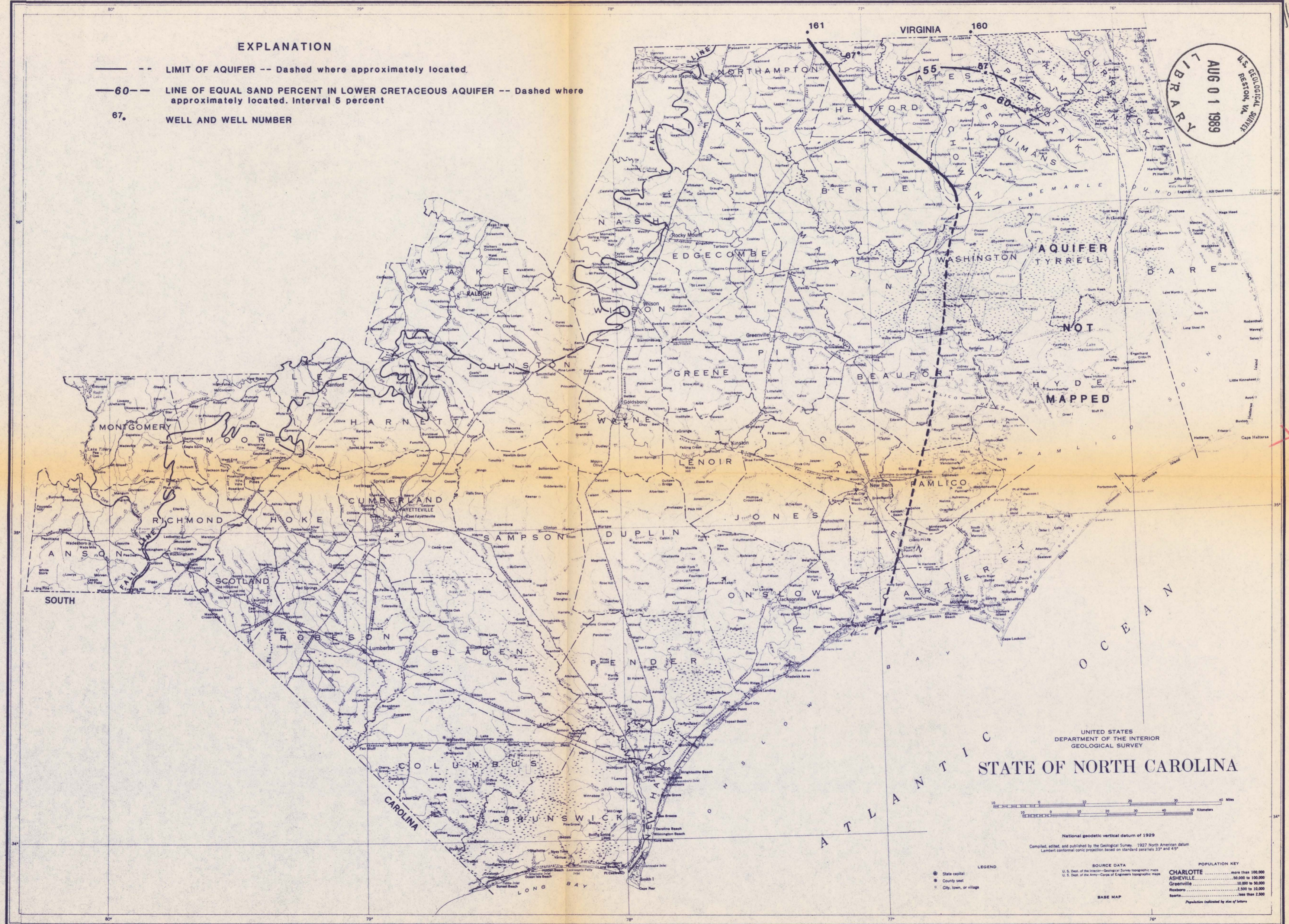
SAND PERCENTAGE IN THE LOWER CRETACEOUS AQUIFER
