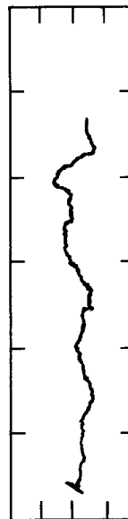
GAMMA LOG
