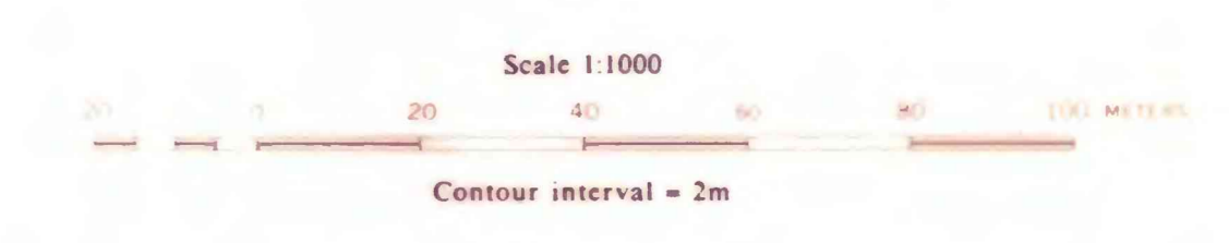
SAMPLE LOCALITY AND GOLD DISTRIBUTION MAP OF THE AR RAHAIL ANCIENT GOLD MINE, KINGDOM OF SAUDI ARABIA by Willie H. White, Rasheed M. Samster and Jeff L. Doebrich AH 1407 AD 1986
