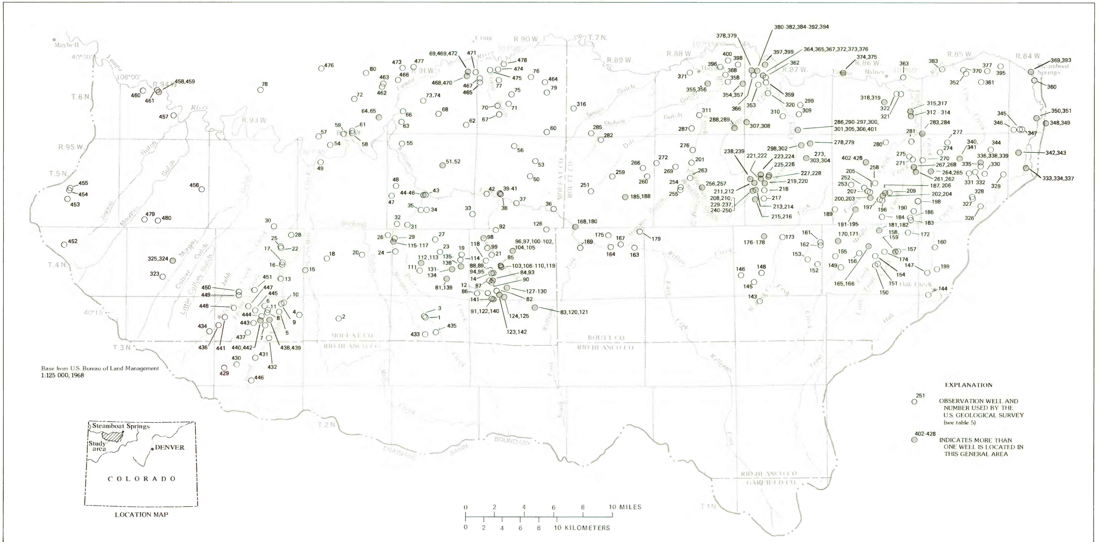
MAP SHOWING GROUND-WATER SITES FOR WHICH WATER-QUALITY, WATER-LEVEL, OR WELL-CONSTRUCTION DATA COLLECTED BY THE U.S. GEOLOGICAL SURVEY ARE AVAILABLE, NORTHWESTERN COLORADO
