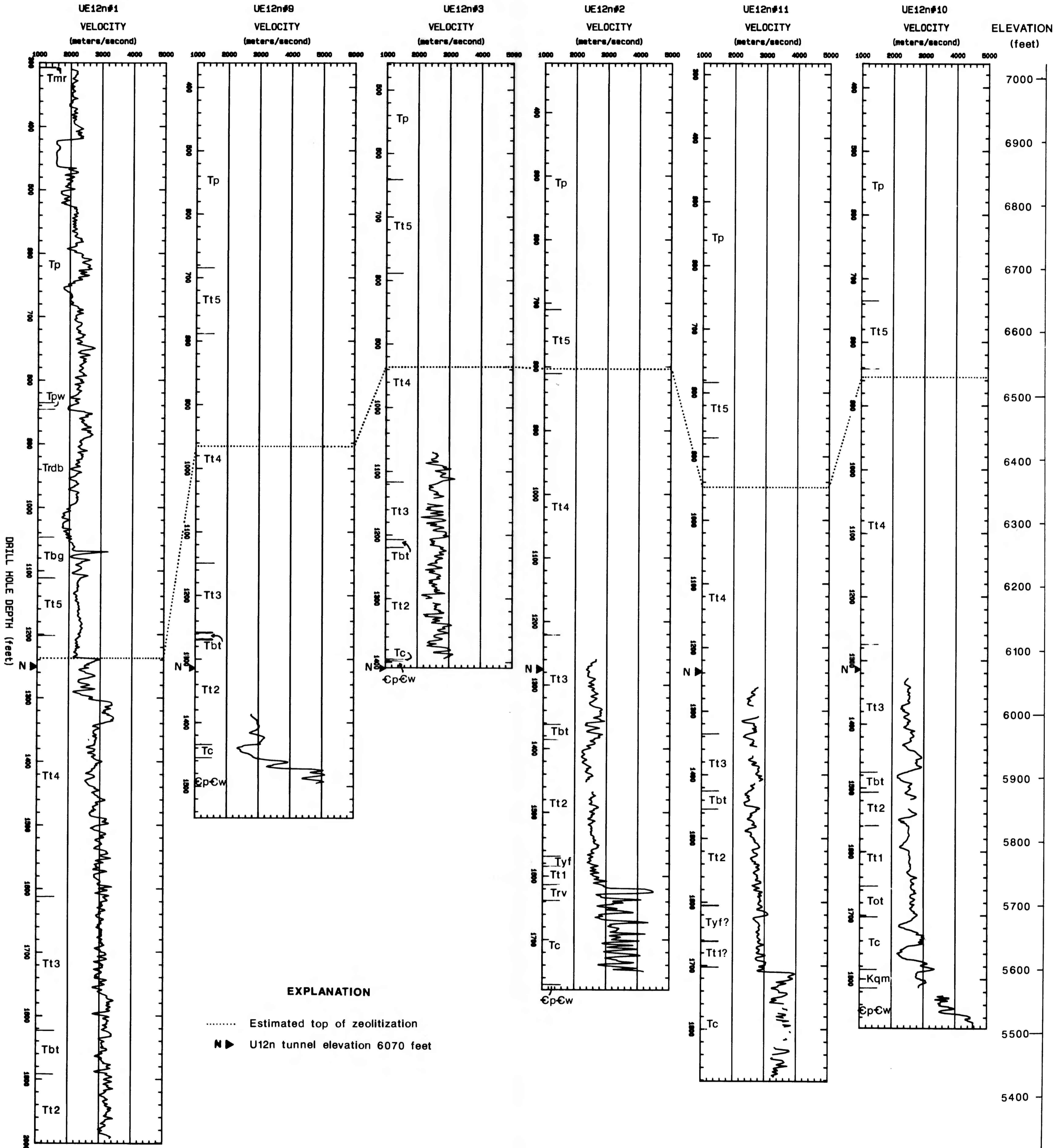
Lithologic and continuous velocity logs obtained in holes in northern N-tunnel area. (See fig. 2 for explanation of stratigraphy)
