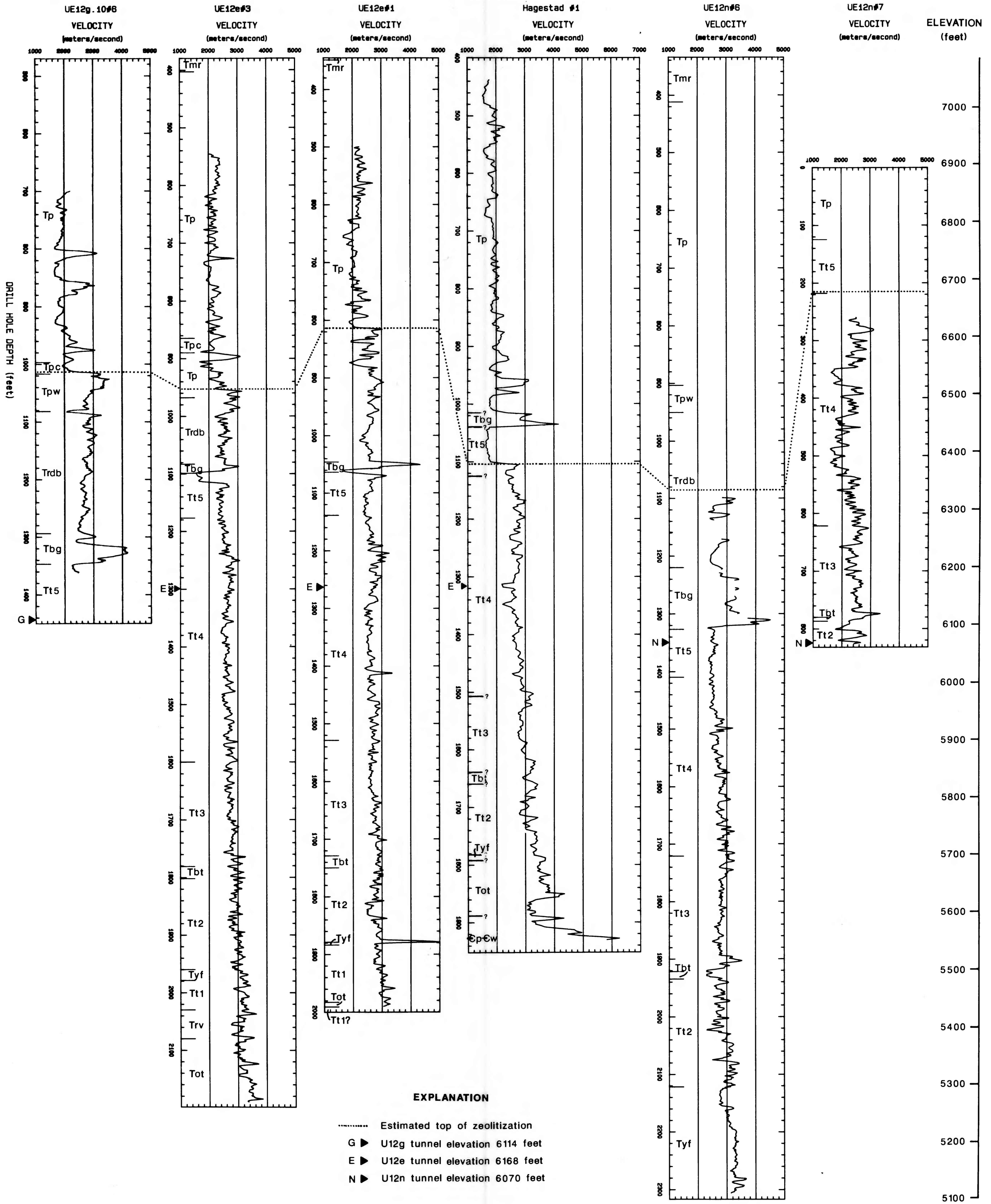
Lithologic and continuous velocity logs obtained in holes in central and southern Rainier Mesa. (See fig. 2 for explanation of stratigraphy)
