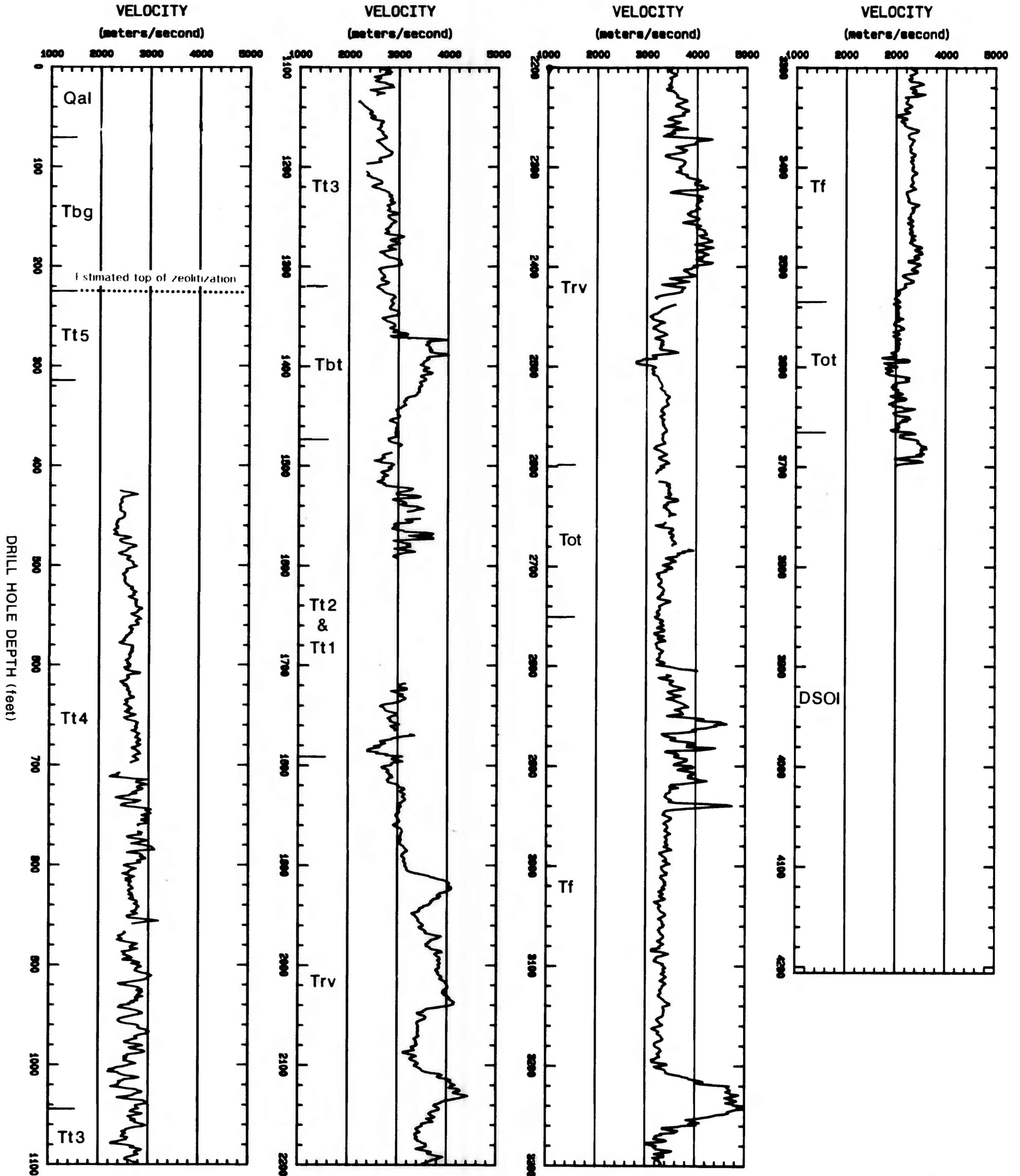
Lithologic and continuous velocity logs obtained in HTH#1 drill hole. Elevation of hole collar is 6156 feet. (See fig. 2 for explanation of stratigraphy)
