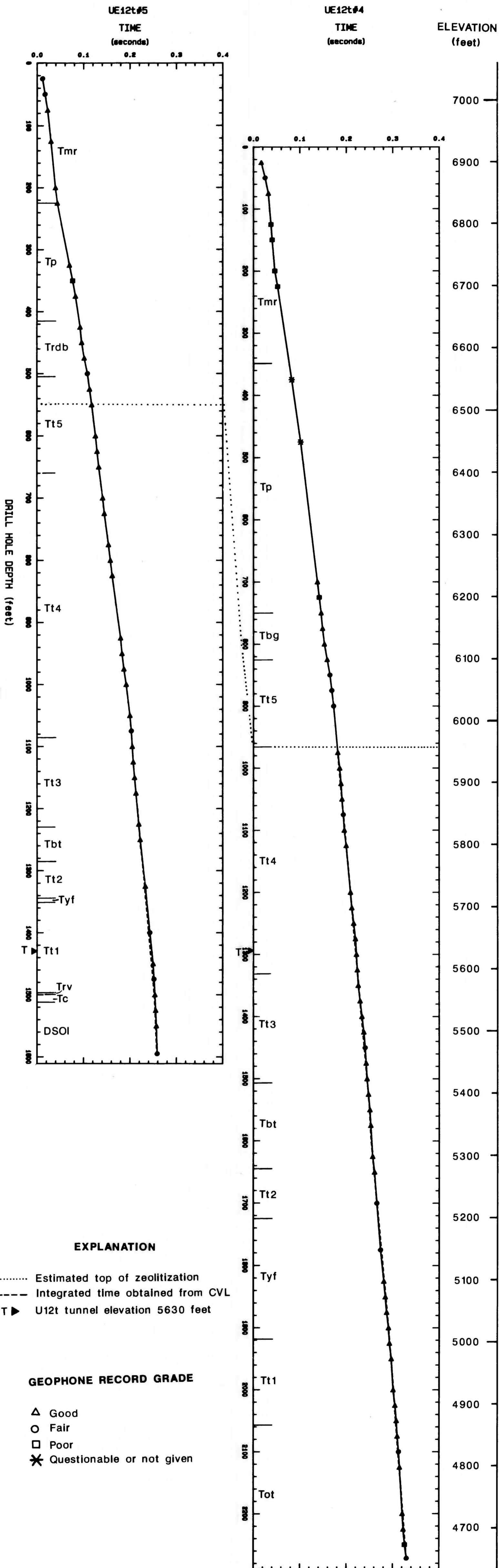
Geophone surveys obtained in holes in T-tunnel area. (See fig. 2 for explanation of stratigraphy)
