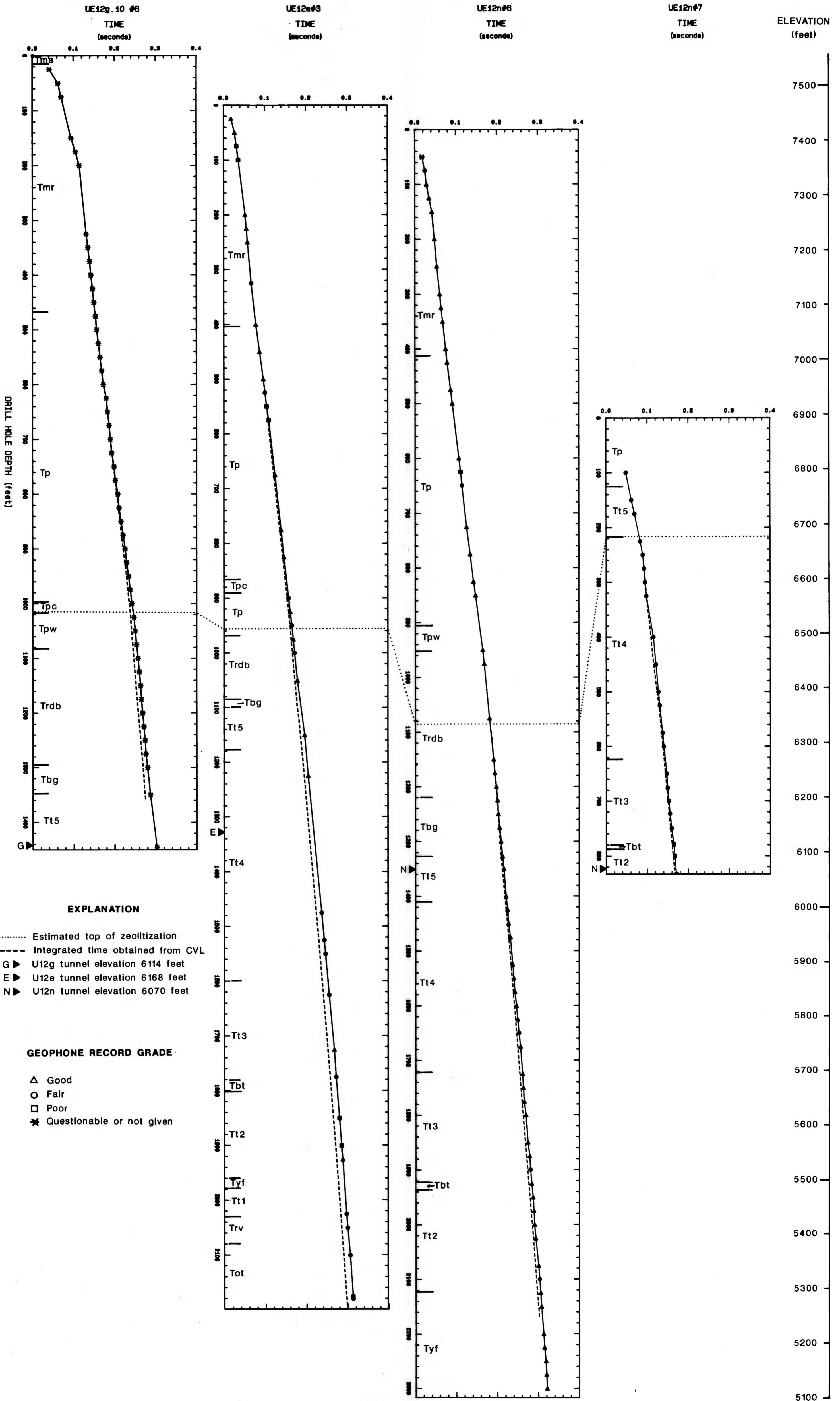
Geophone surveys obtained in holes in central and southern Rainier Mesa. (See fig. 2 for explanation of stratigraphy)
