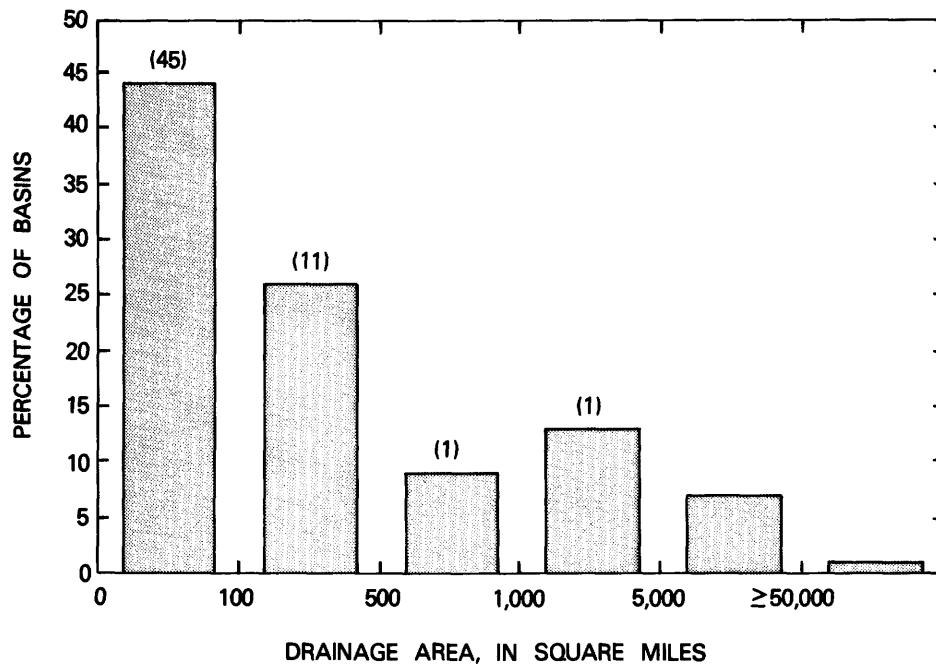
FIGURE 9. Histogram depicting the percentage of continuously operated streamgages in 1987, by drainage area. Number of Benchmark stations in each drainage area class appears in parentheses above the respective bar.
