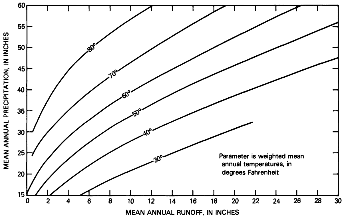
FIGURE 2. Relationship of annual runoff to precipitation and temperature. Source: Langbein and others, 1949.
