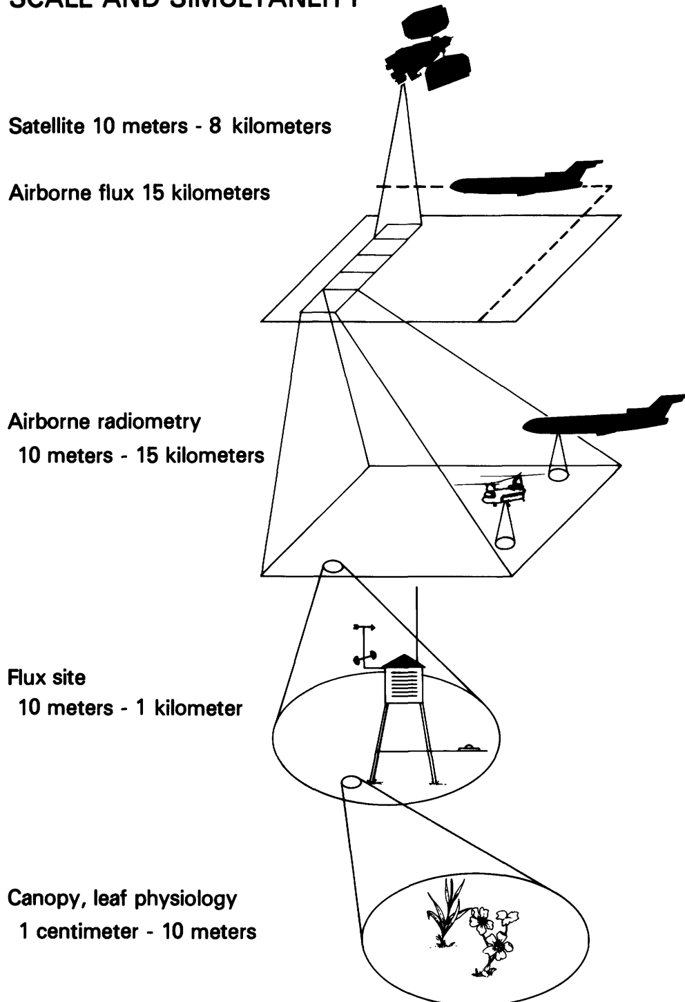
FIGURE 10. Range of scales addressed by the First International Satellite Land Surface Climatology Project field experiment. Source: Brutsaert and others, 1988.
