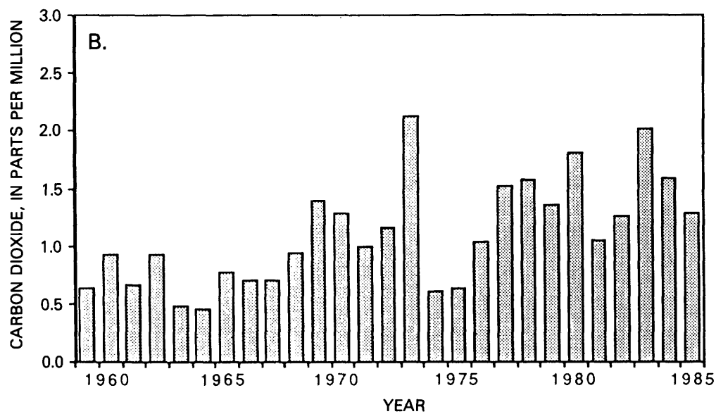
FIGURE 1. Annual mean concentrations of atmospheric carbon dioxide measured at the Mauna Loa Observatory (a), and annual changes in mean concentrations (b).
