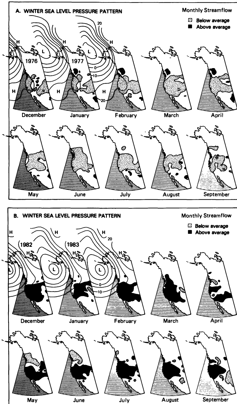
FIGURE 5. Mean sea-level pressure in "millibars - 1000" and monthly streamflow patterns: (a) winter 1976-1977 and (b) winter 1982-1983. Below average refers to the lower quartile flow and above average to the upper quartile of flow. Source: Peterson and others, 1987.
