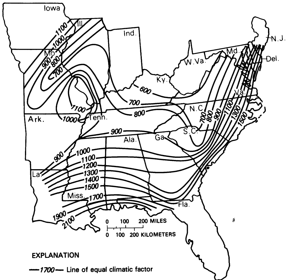
FIGURE 7. Geographic variation of the climate factor for the 100-year recurrence-interval flood. Source: Lichy and Liscum, 1978.
