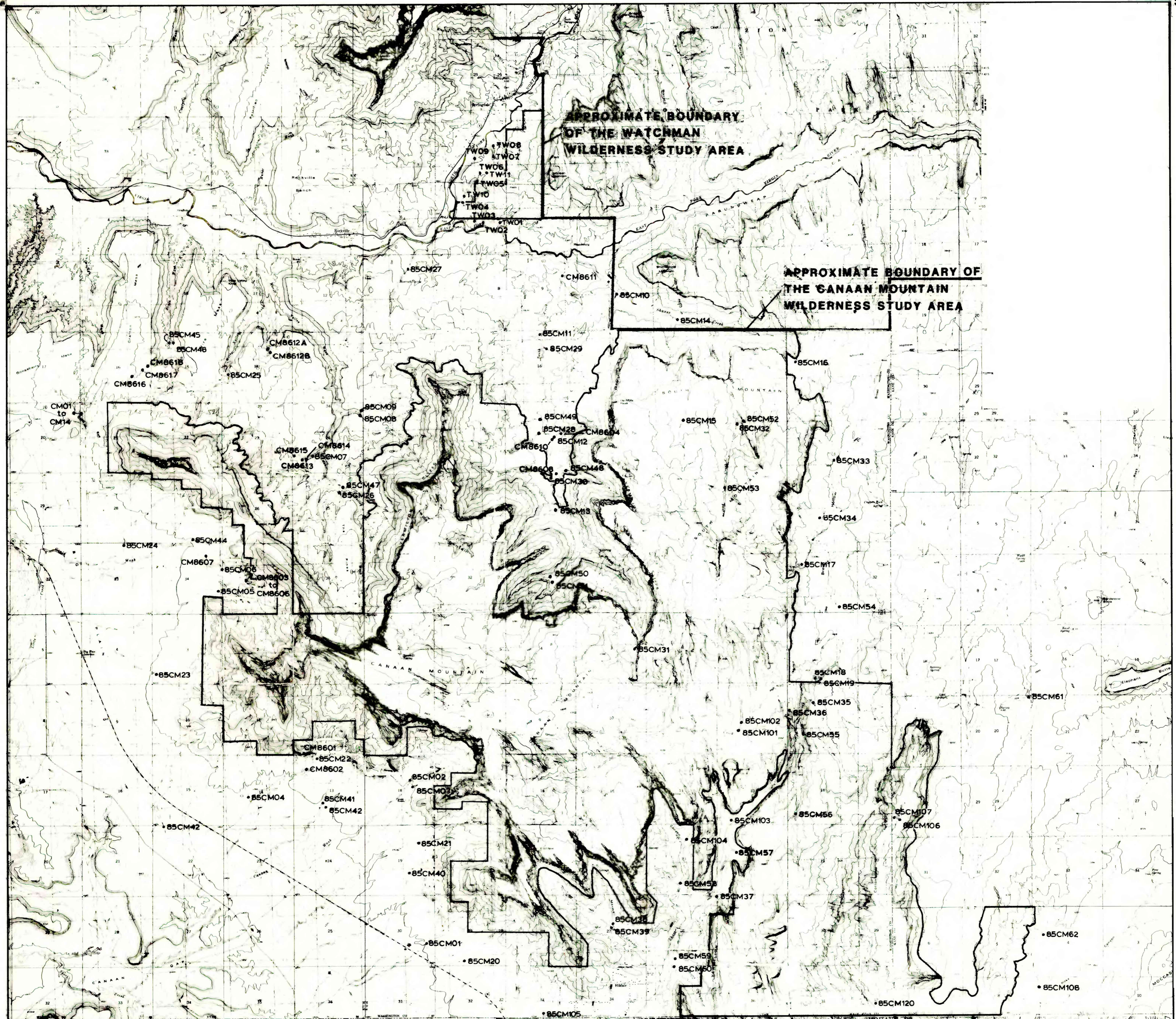
PLATE 1. LOCALITIES OF STREAM-SEDIMENT, HEAVY-MINERAL-CONCENTRATE, AND ROCK SAMPLES FROM THE CANAAN MOUNTAIN (UT-040-143) AND THE WATCHMAN (UT-040-149) WILDERNESS STUDY AREAS, KANE AND WASHINGTON COUNTIES, UTAH
