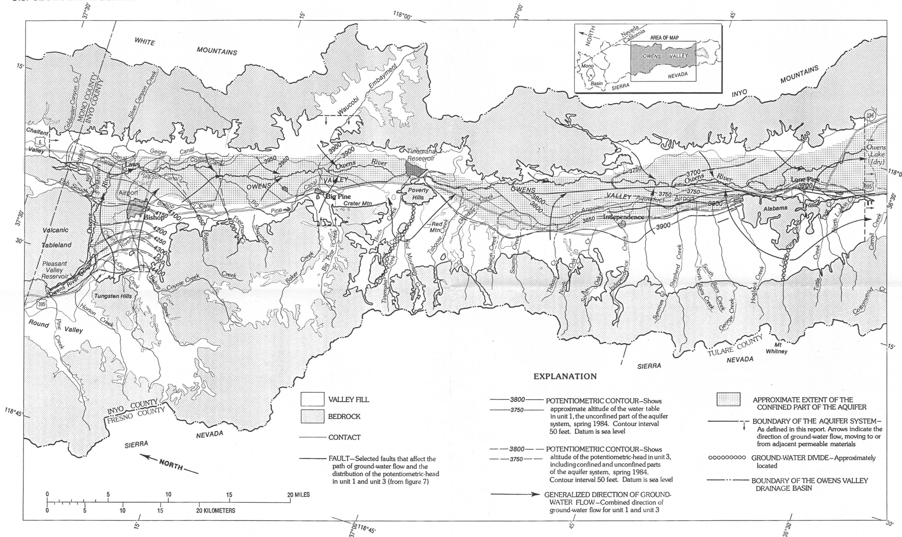
Figure 17. Areal extent of defined aquifer system, occurrence of unconfined and confined conditions, boundary conditions, configuration of potentiometric surface in hydrogeologic units 1 and 3, and direction of ground-water flow, spring 1984.
