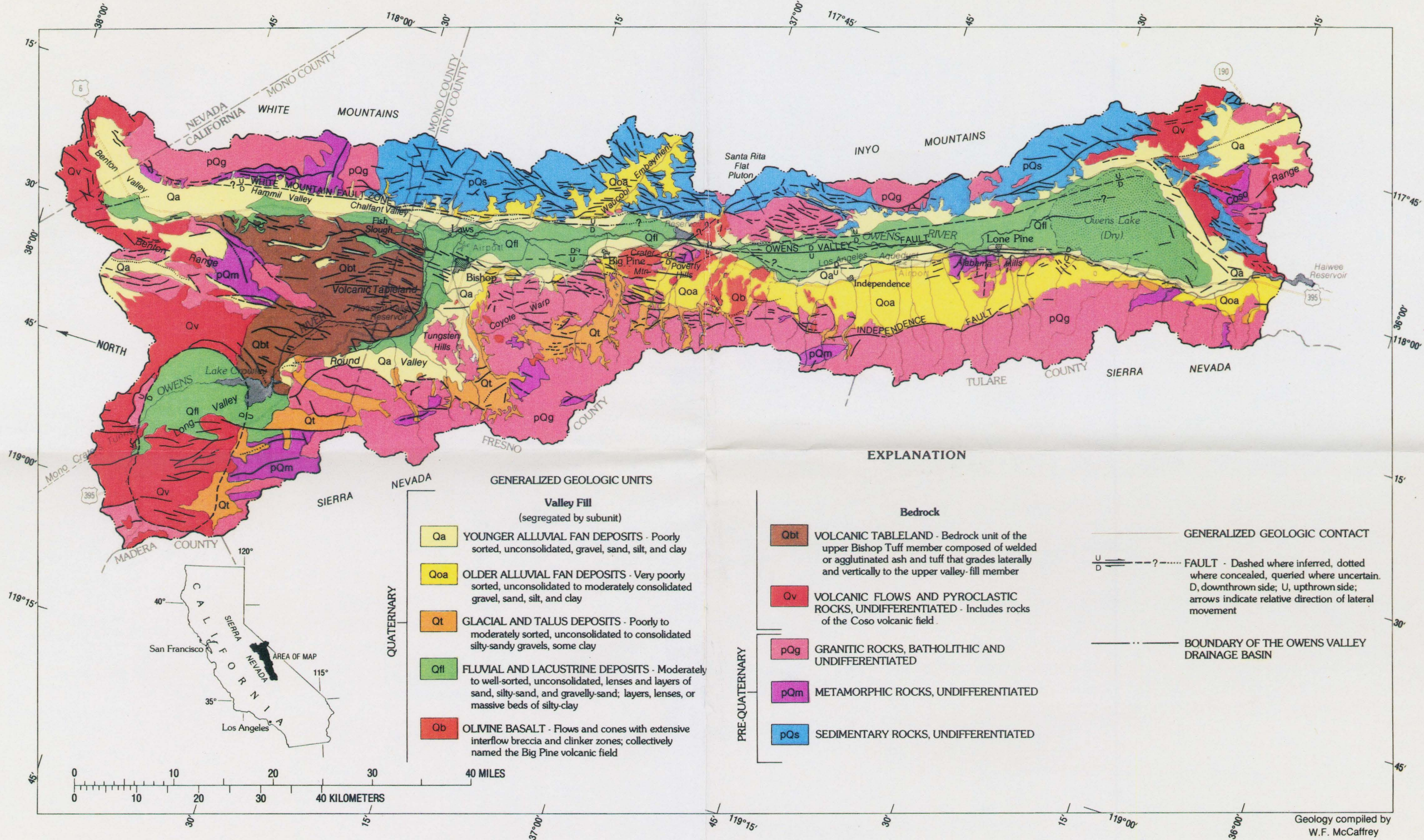
Figure 7. Generalized geologic map of the Owens Valley drainage basin (geology compiled from sources shown in fig. 6 and this study).
