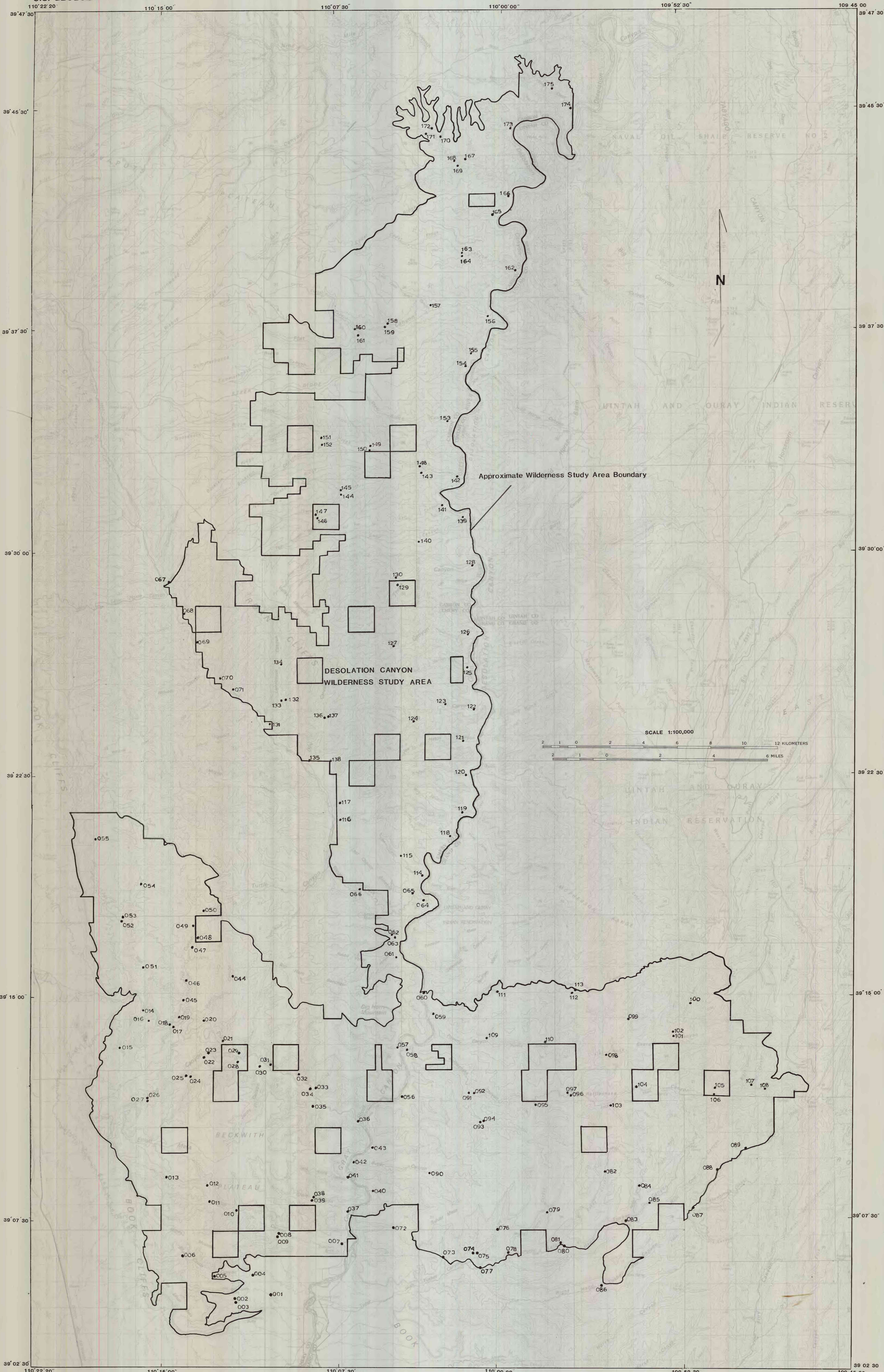
LOCALITIES OF STREAM-SEDIMENT AND HEAVY-MINERAL CONCENTRATE SAMPLES COLLECTED FROM THE DESOLATION CANYON WILDERNESS STUDY AREA, EMERY AND CARBON COUNTIES, UTAH
