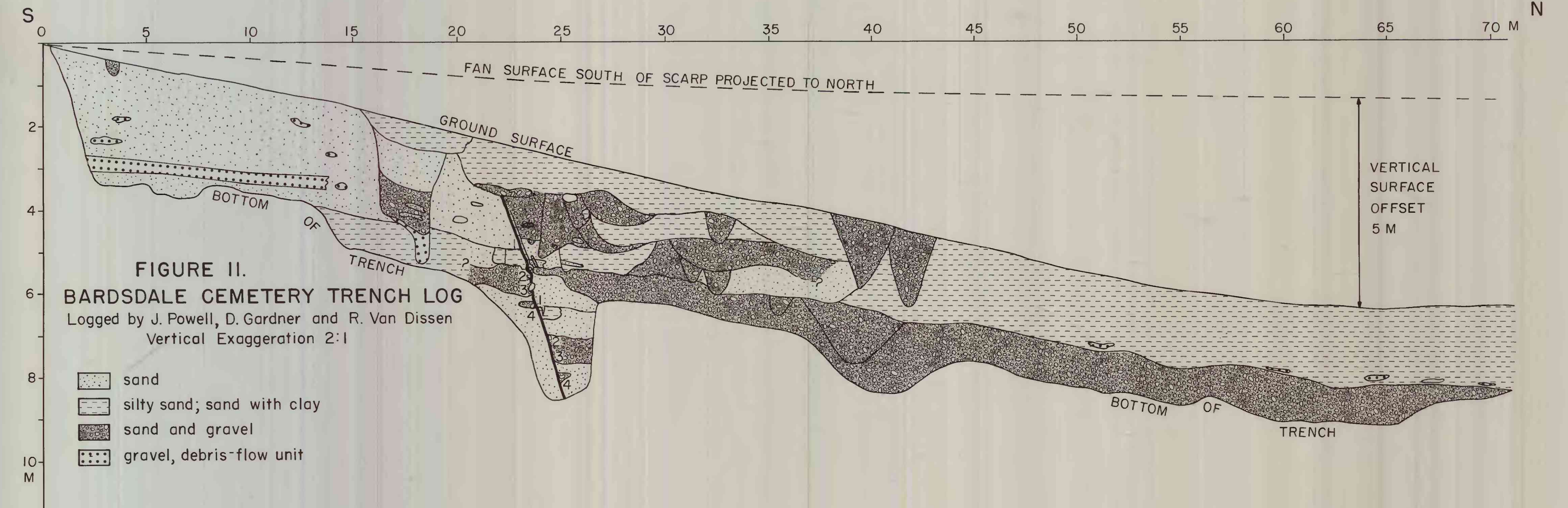
FIGURE 11. BARSDALE CEMETERY TRENCH LOG Logged by J. Powell, D. Gardner and R. Van Disen Vertical Exaggeration 2:1
