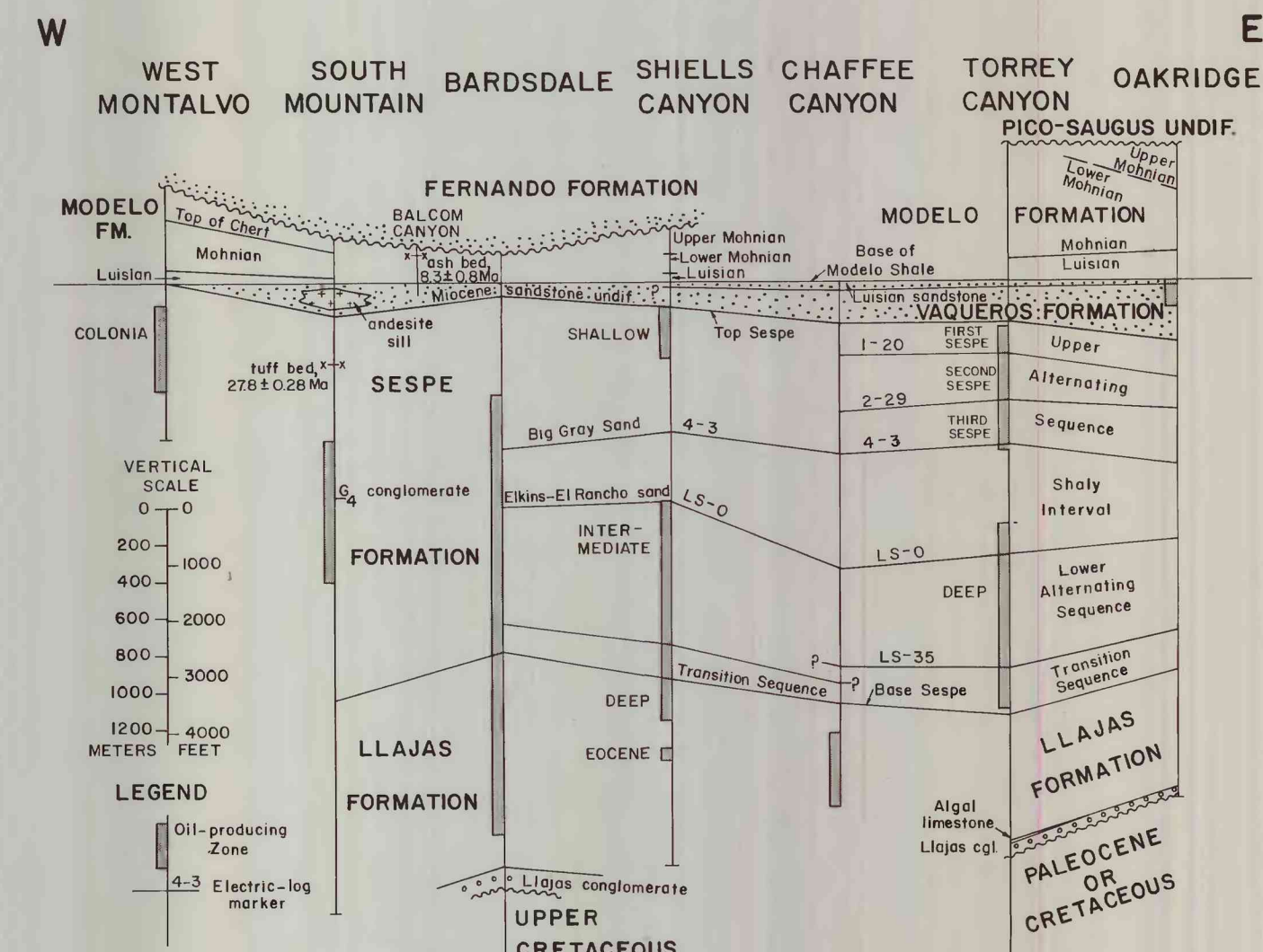
Figure 2. STRATIGRAPHIC CORRELATION SECTION, HANGING WALL OF OAK RIDGE FAULT.
