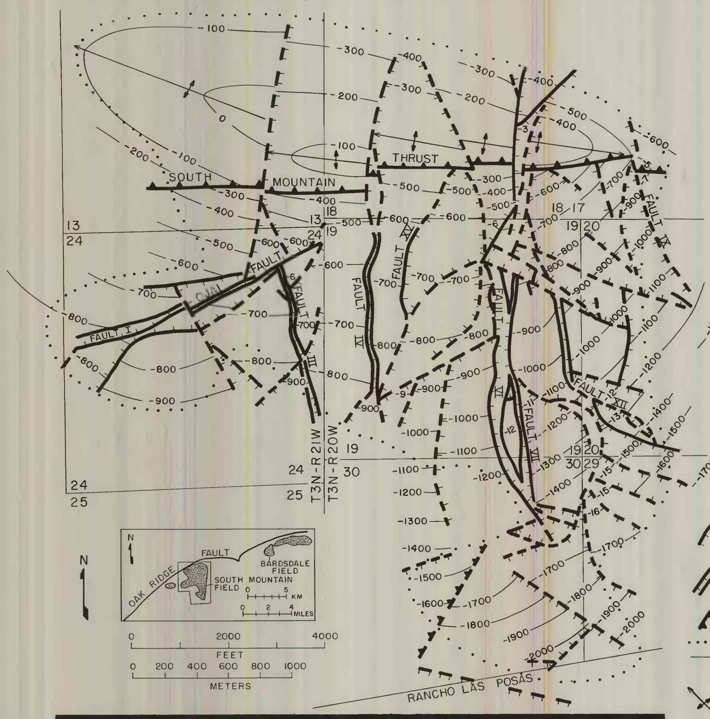
FIGURE 5. SOUTH MOUNTAIN FIELD A. STRUCTURE CONTOURS ON G 4 CONGLOMERATE HORIZON, SESPE FORMATION
