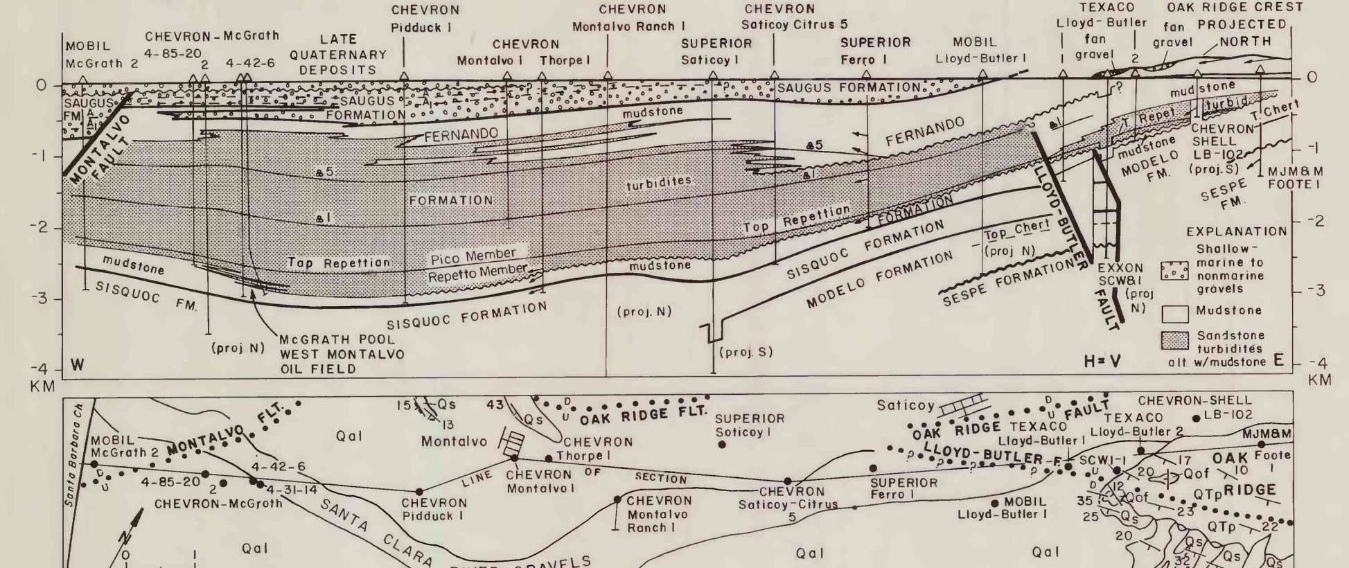
Figure 4. CROSS SECTION OF HANGING WALL OF OAK RIDGE FAULT, PACIFIC COAST TO OAK RIDGE.
