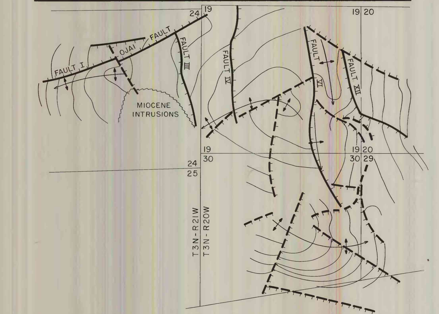
B. STRUCTURE CONTOUR FORM LINES ON G 4 CONGLOMERATE HORIZON AS IT WOULD APPEAR IF BAILEY ASH HORIZON WERE HORIZONTAL.
