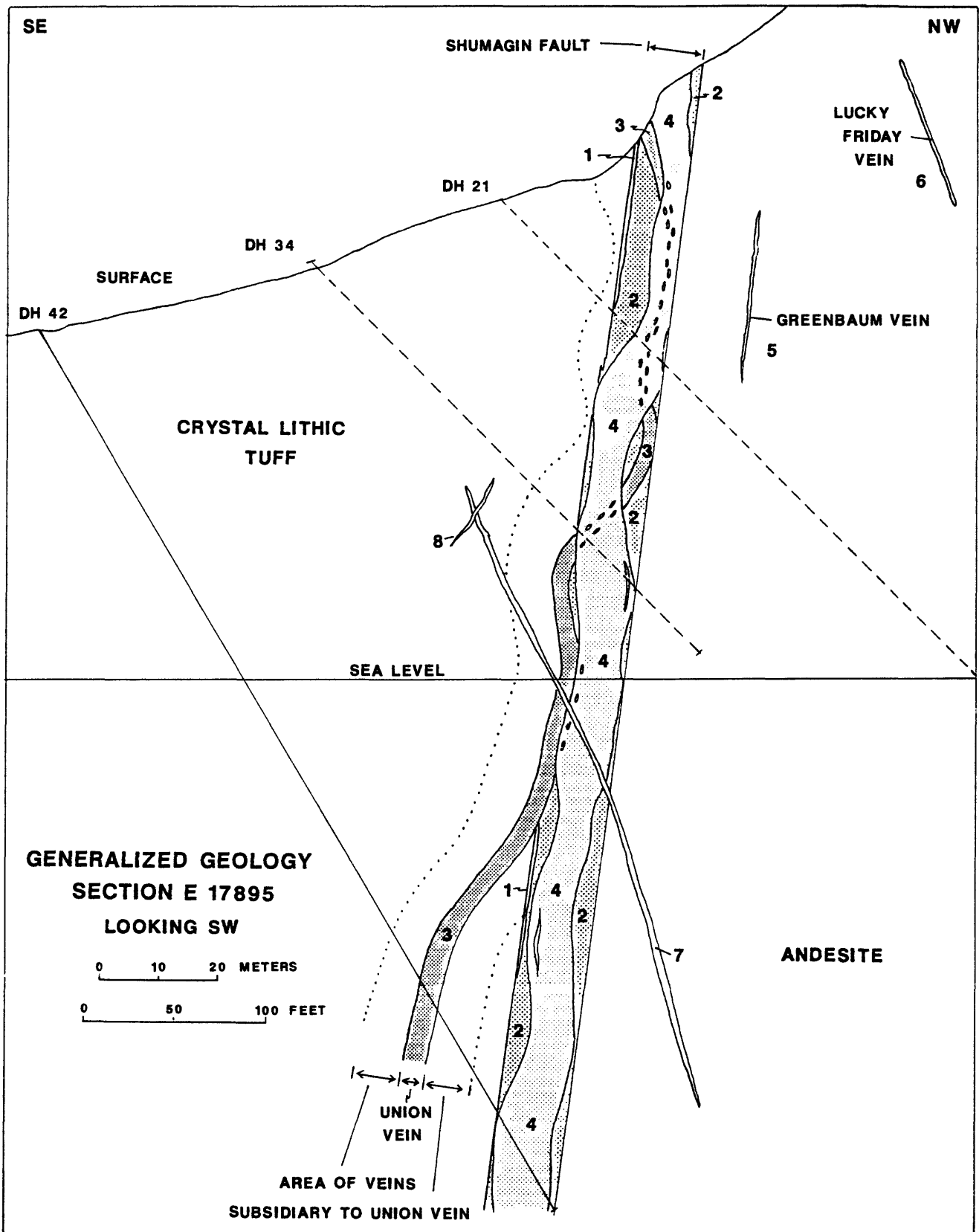
Figure 3. Generalized geology of Section E 17895, looking southwest. Drill hole 34 is projected 49 m to section and aligned with the footwall of the Shumagin fault. Numbers refer to relative ages of units described in text.
