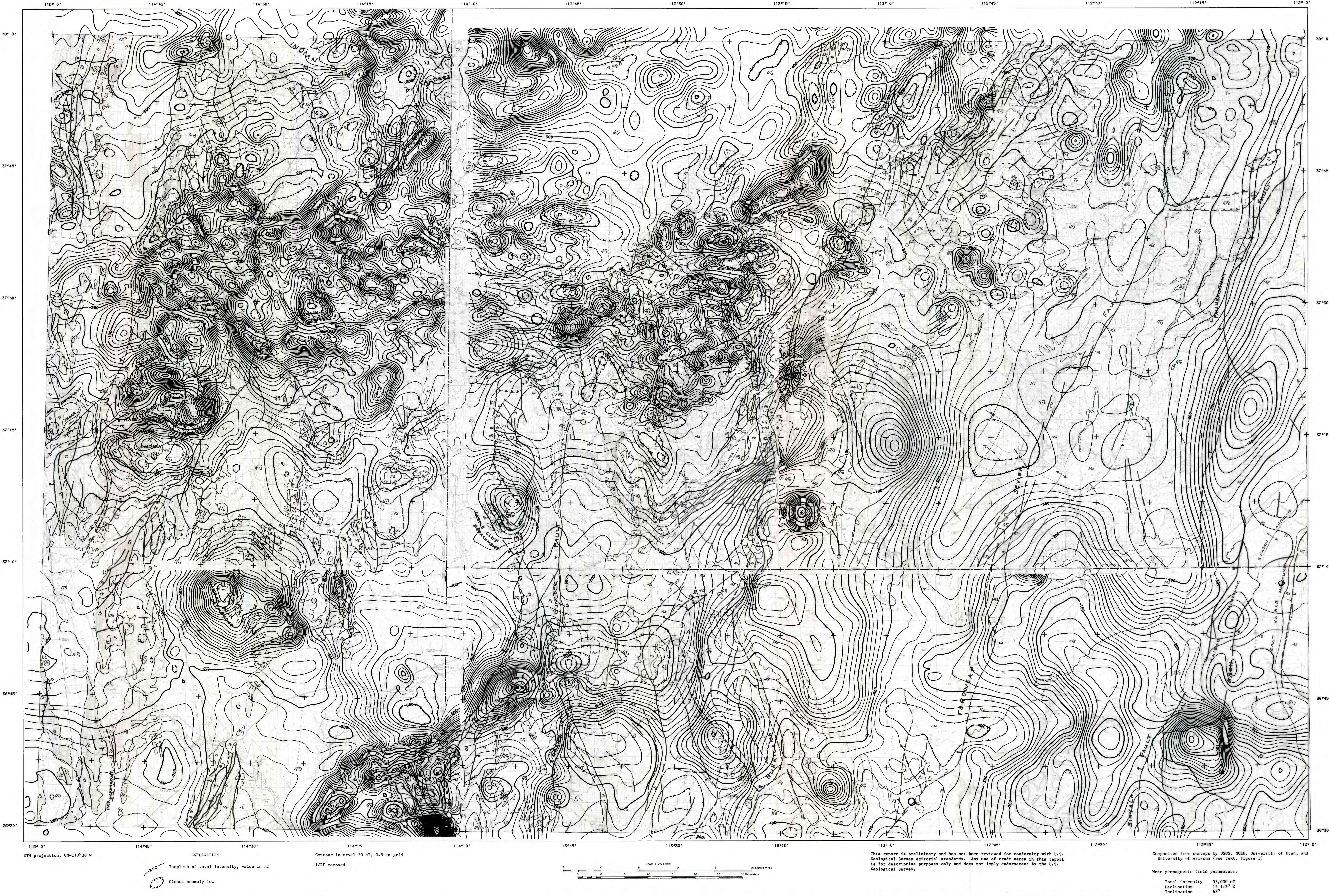
RESIDUAL TOTAL-INTENSITY AEROMAGNETIC ANOMALY MAP OF THE USGS "BARCO" PROJECT AREA, SOUTHWESTERN UTAH, SOUTHEASTERN NEVADA, AND NORTHWESTERN ARIZONA
