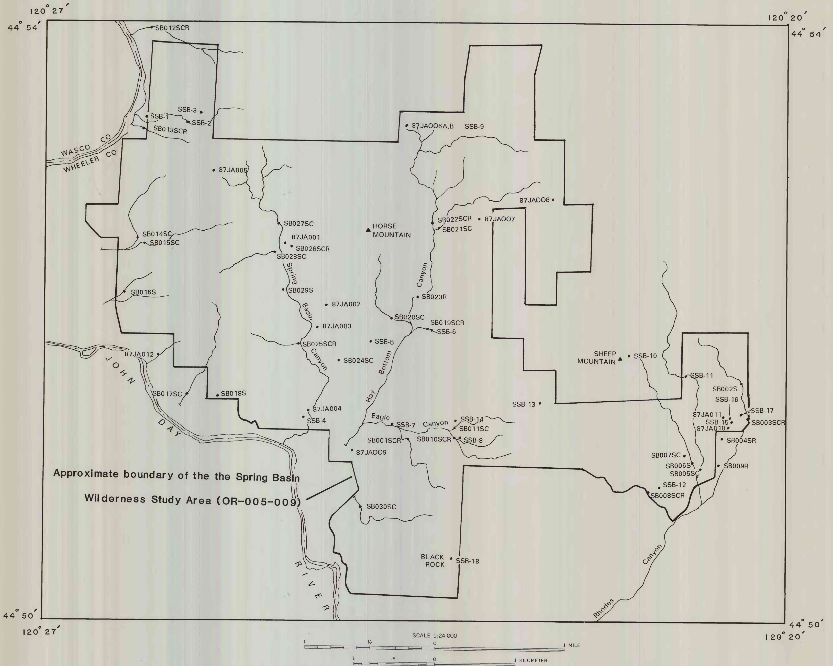
PLATE 1- LOCALITIES OF HEAVY-MINERAL CONCENTRATES, STREAM SEDIMENTS, AND ROCKS FROM THE SPRING BASIN WILDERNESS STUDY AREA (OR-005-009), WHEELER COUNTY, OREGON
