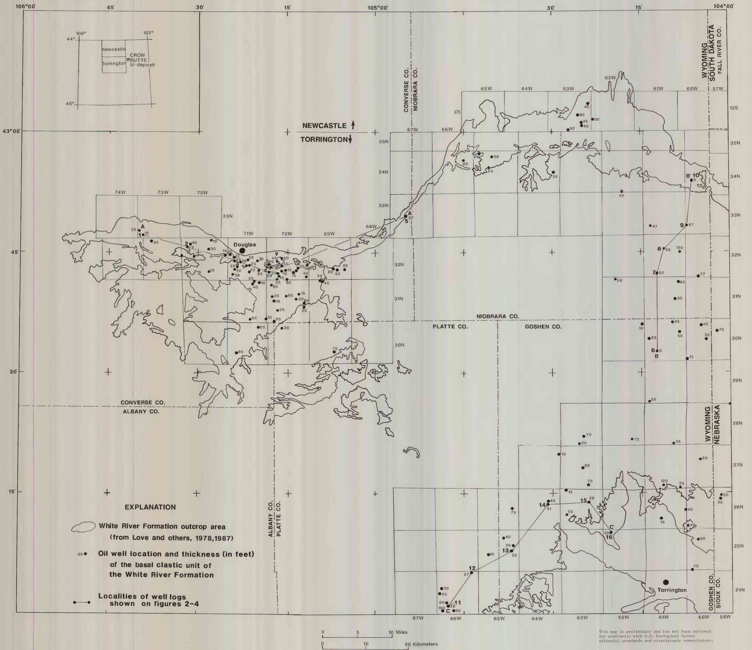
Figure 1.-- Thickness of the basal clastic unit of the white River Formation
