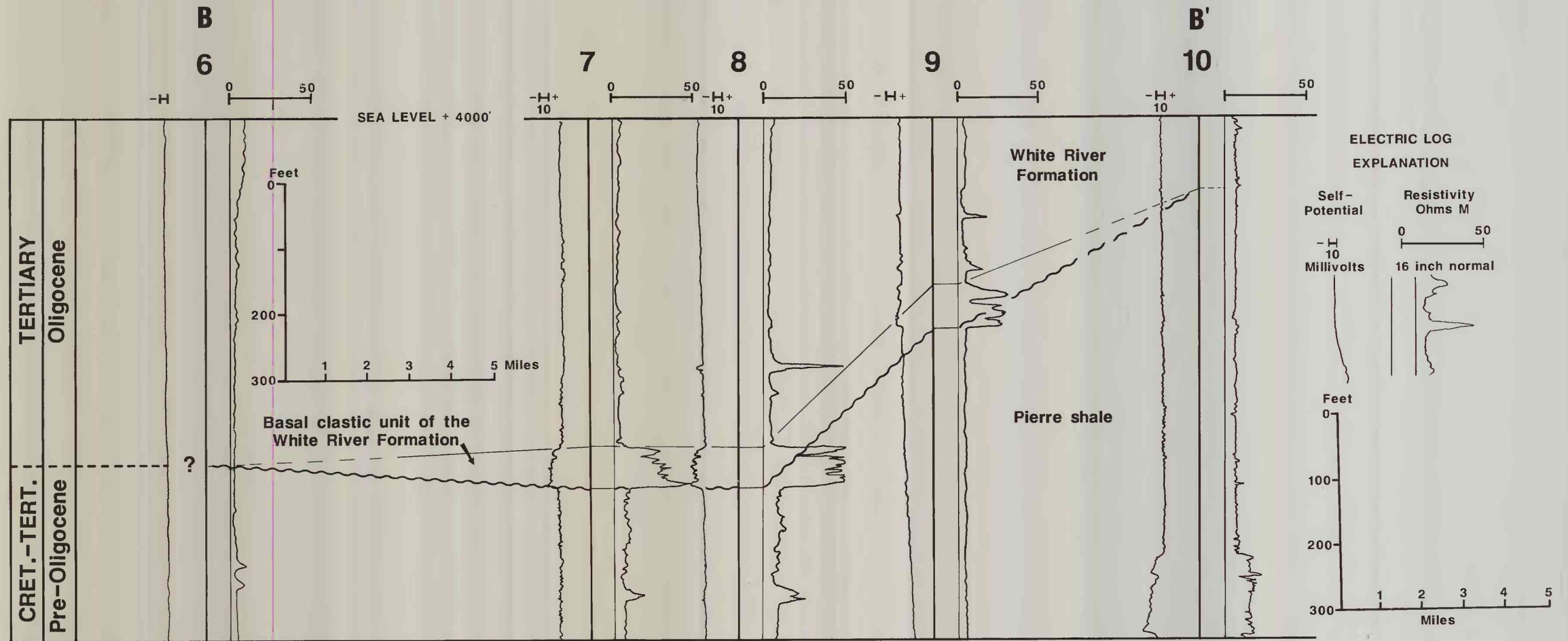
Figure 3.-- Line of electric log sections showing correlation of basal clastic unit of the White River Formation.
