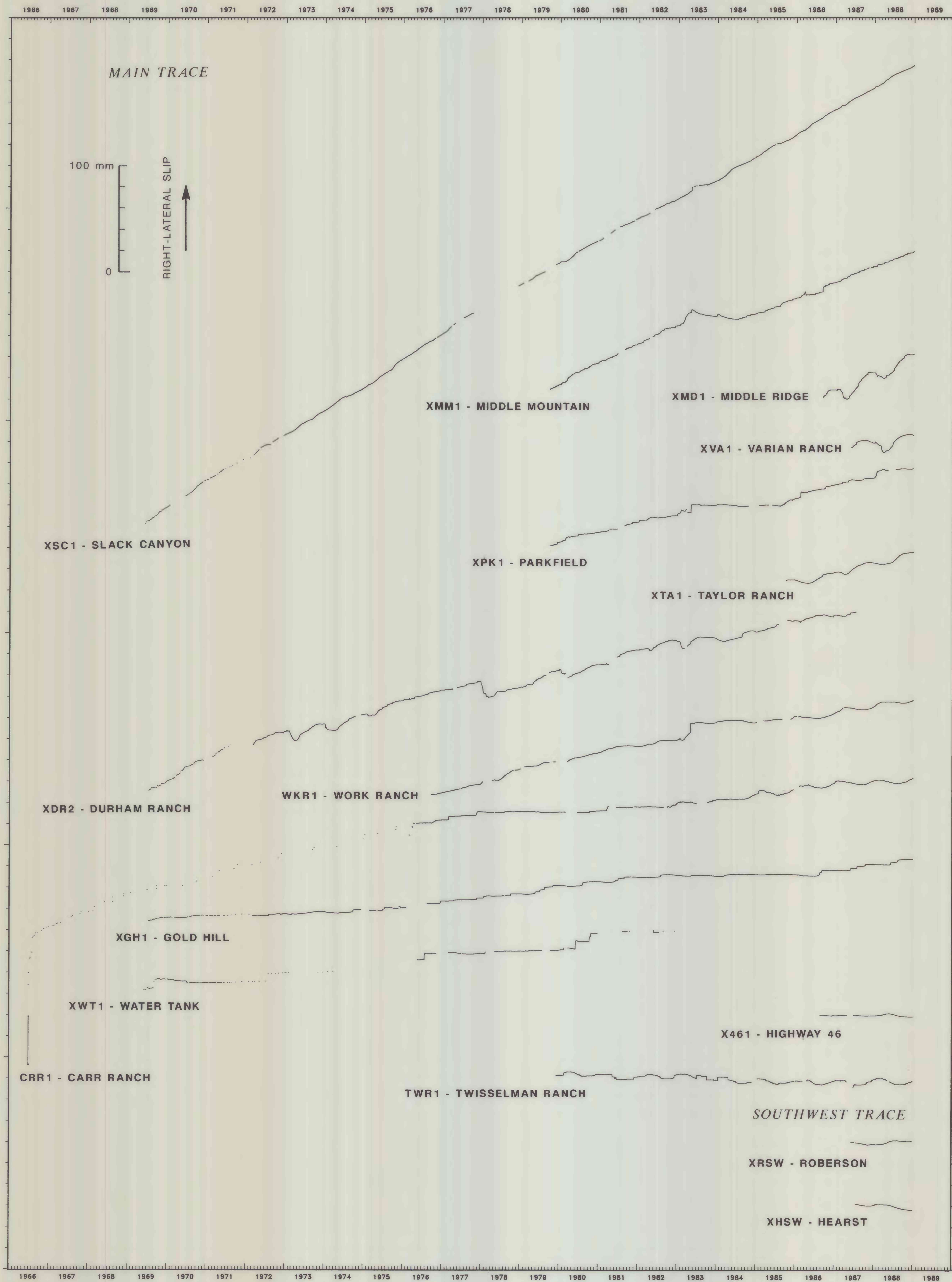
CUMULATIVE CREEP RECORDED BY U.S.G.S. CREEPMETERS ON THE SAN ANDREAS FAULT AT PARKFIELD, CALIFORNIA, BETWEEN 1966 AND 1988
