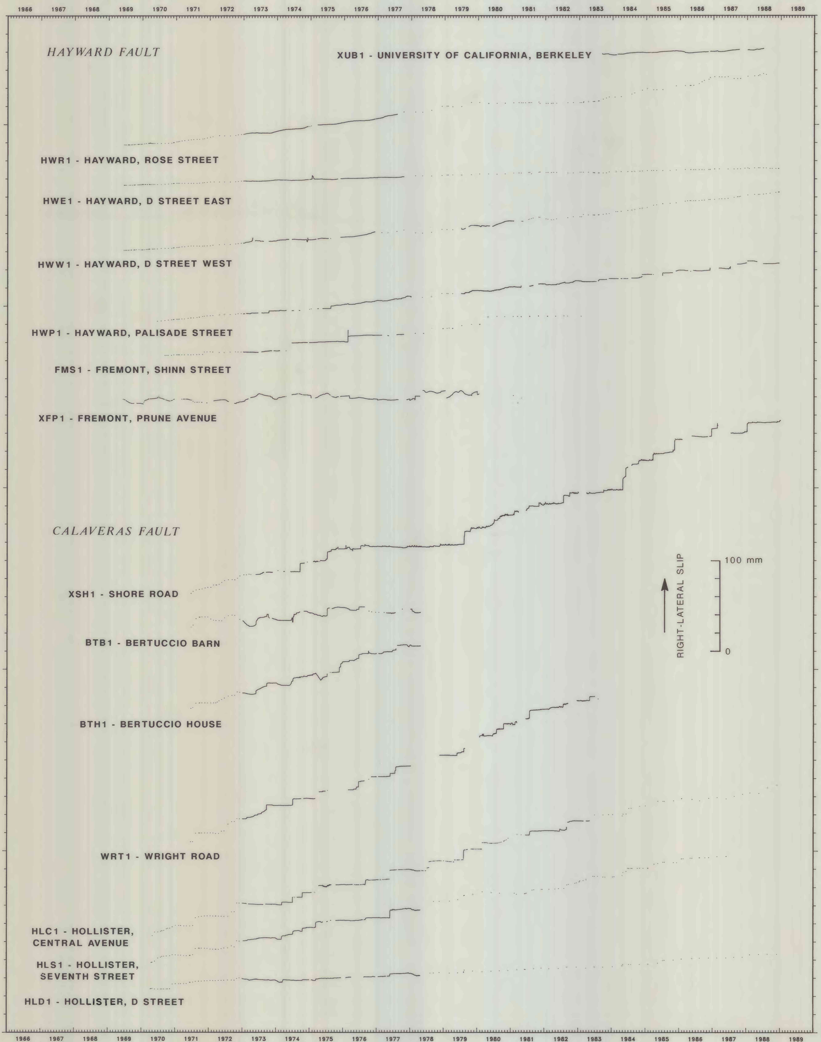
CUMULATIVE CREEP RECORDED BY U.S.G.S. CREEPMETERS ON THE HAYWARD AND CALAVERAS FAULTS BETWEEN 1966 AND 1988
