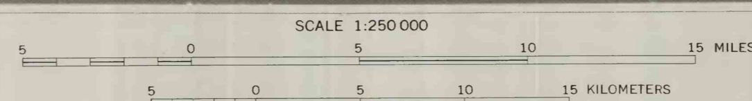
MAP SHOWING LOCATION OF ROCK SAMPLES FROM THE LIME HILLS QUADRANGLE, ALASKA
