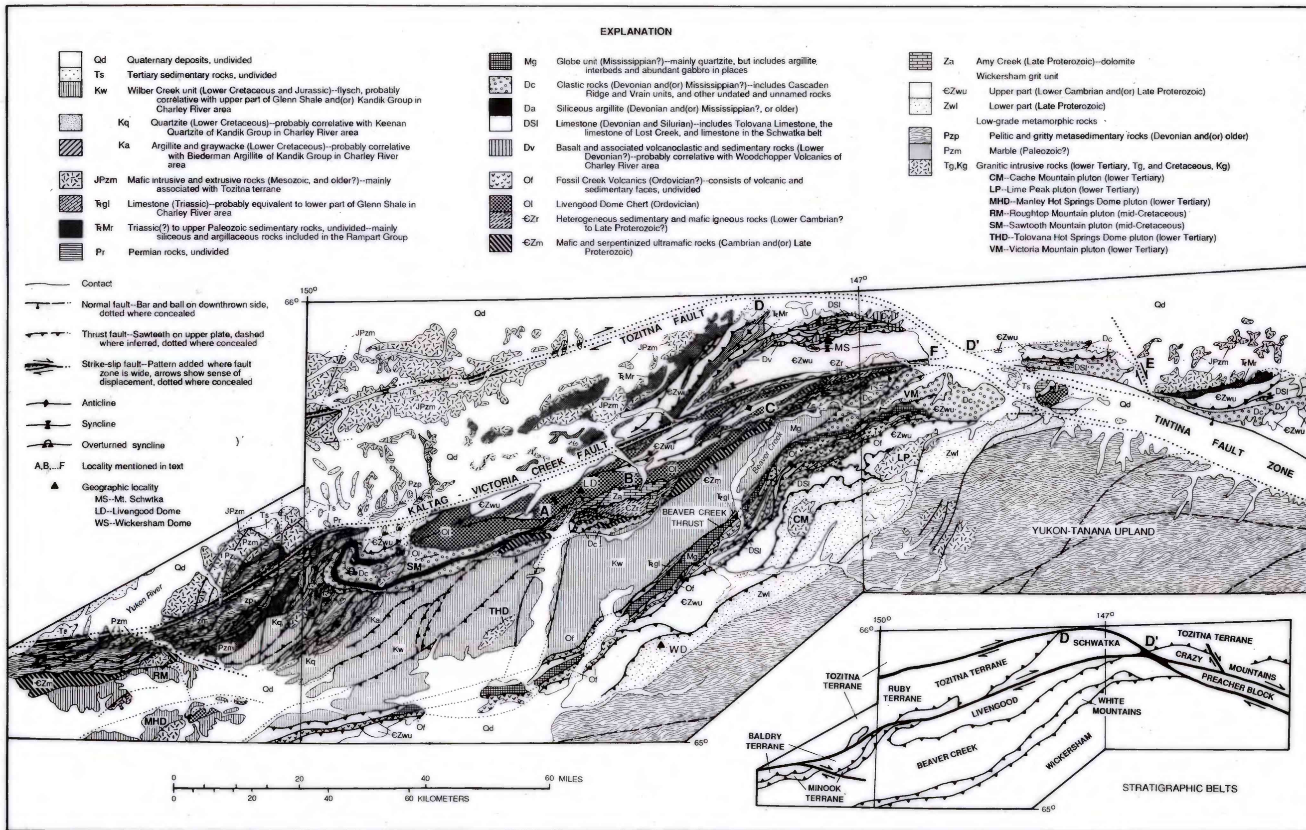
Figure 8. Geologic map of the Livengood area. See figure 3 for area location.
