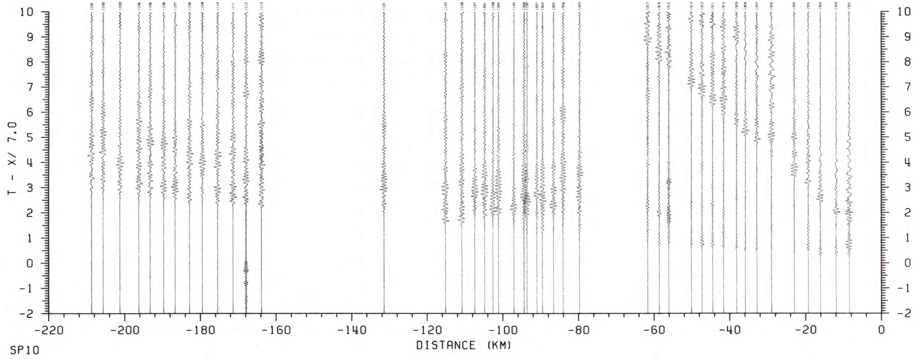
RECORD SECTIONS FROM SHOTPOINTS 10-14 THE 1988 GRENVILLE-APPALACHIAN SEISMIC REFRACTION EXPERIMENT IN ONTARIO, NEW YORK, AND NEW ENGLAND by J. Luetgert, S. Hughes, J. Cipar, S. Mangino, D. Forsyth and I. Asudeh 1990
