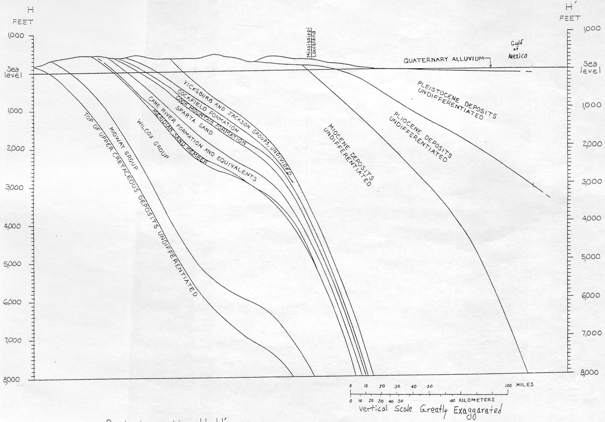
Figure 10.-- Geologic section H-H'.
