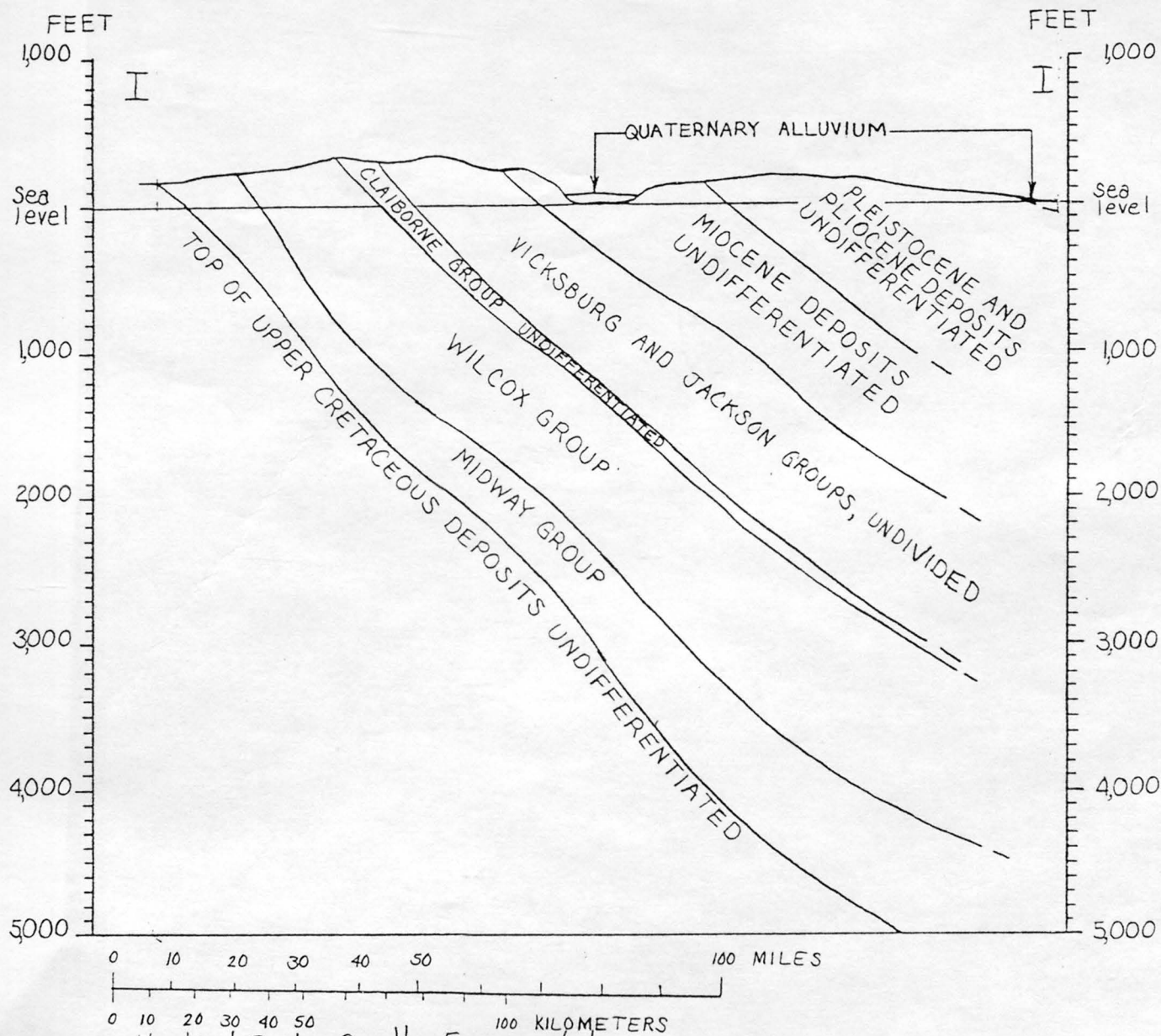
Figure 11.-- Geologic section I-I'.
