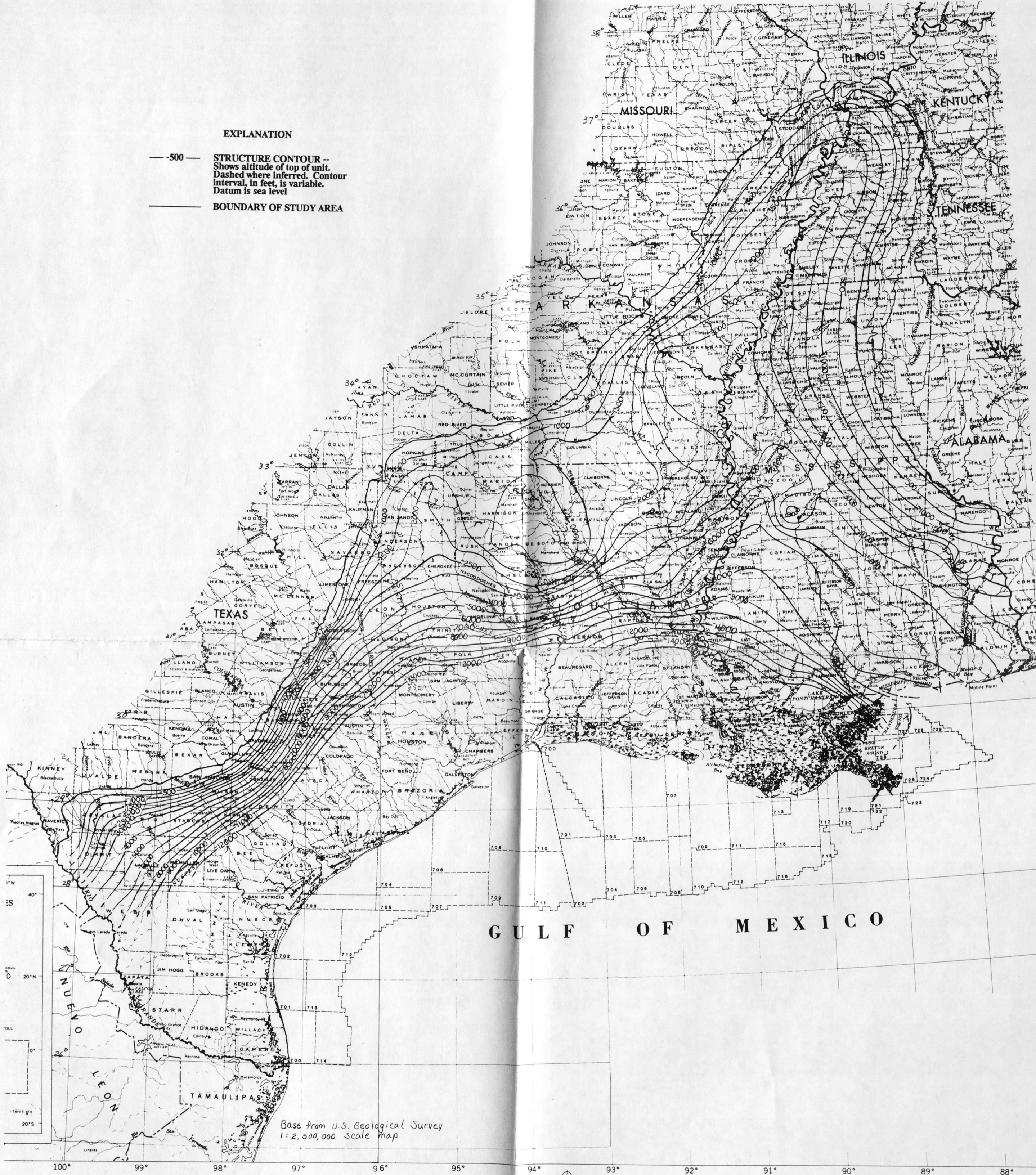
Figure 15. -- Altitude and configuration of the top of Upper Cretaceous deposits.
