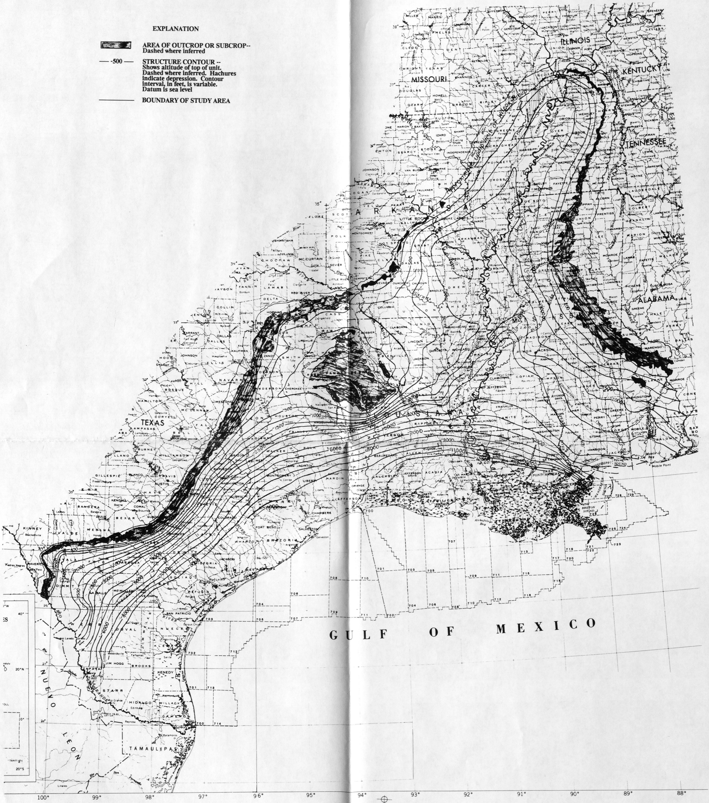
Figure 18. -- Altitude and configuration of the top of the Wilcox Group.
