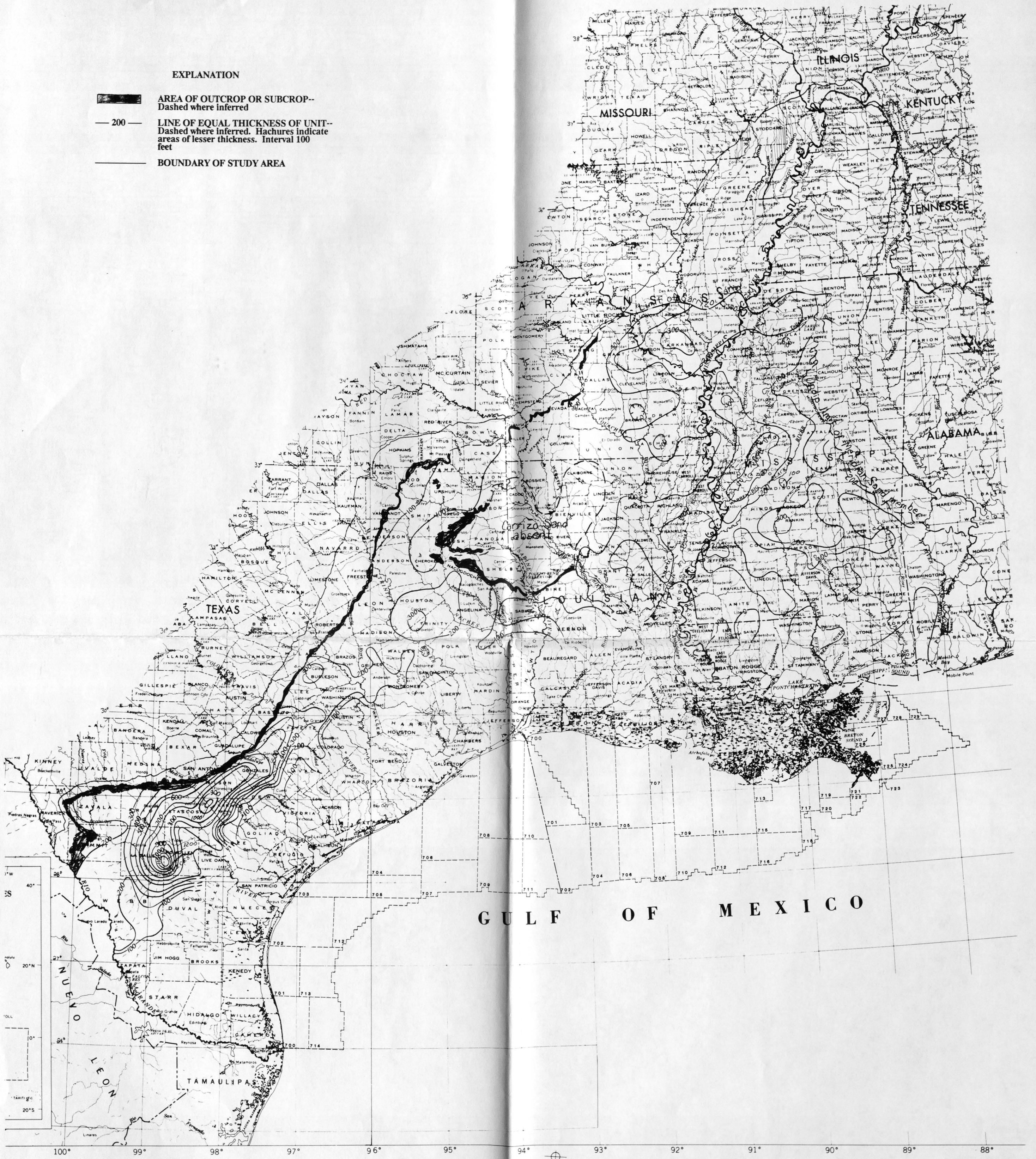
Figure 21. -- Thickness of the Carrizo Sand and Meridian Sand Member.
