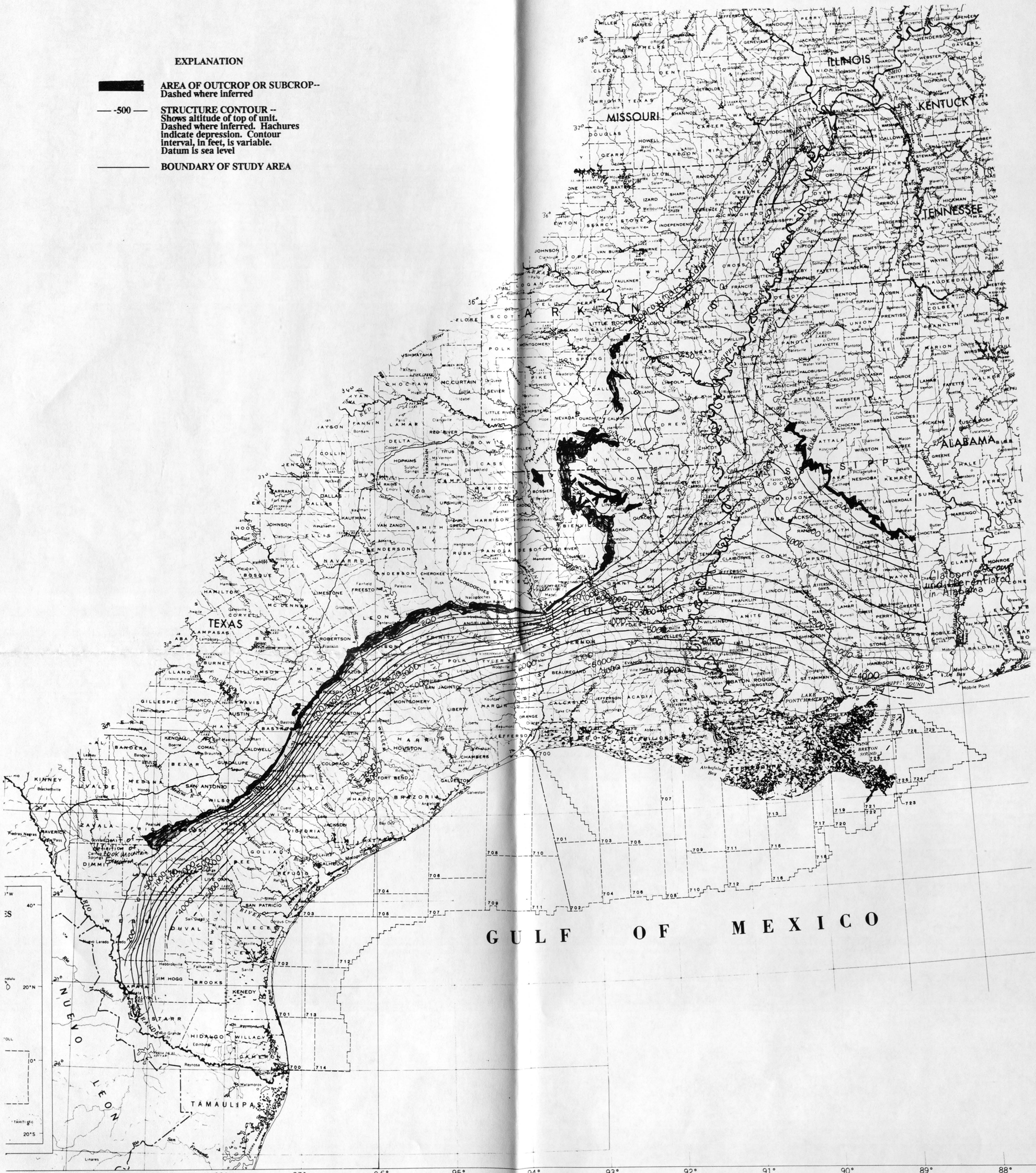
Figure 26.-- Altitude and configuration of the top of the Cook Mountain Formation.
