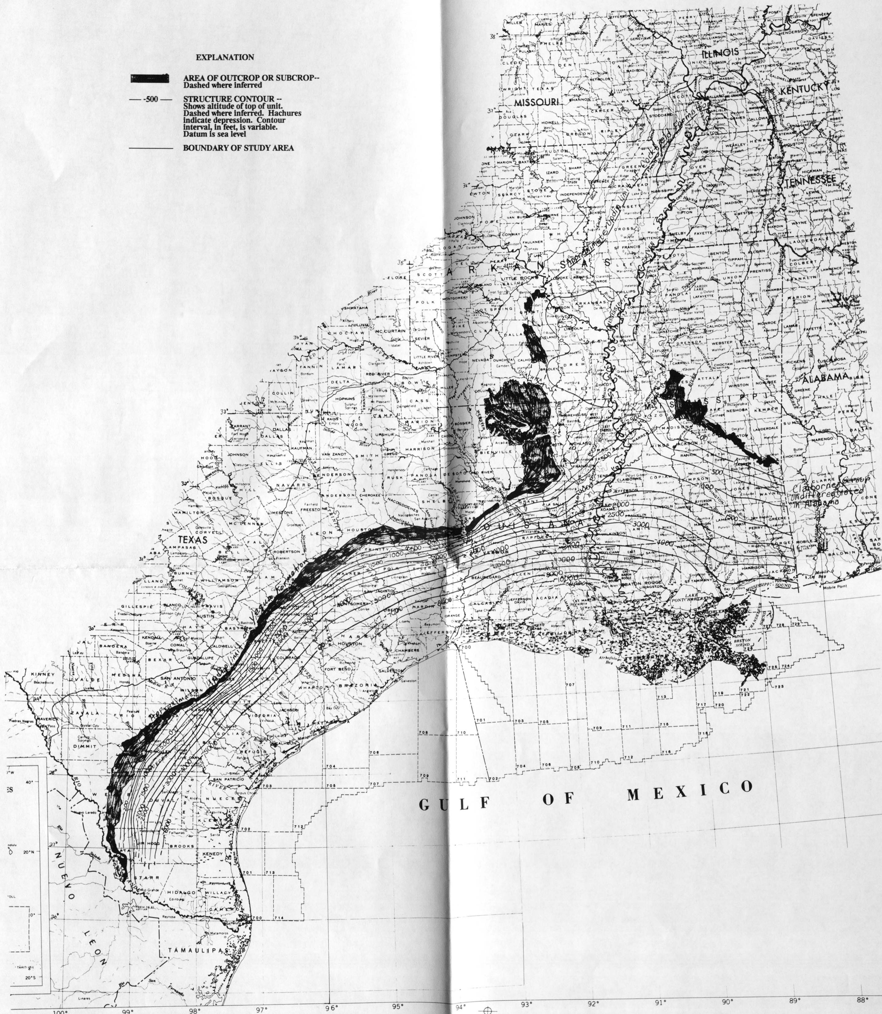
Figure 28. -- Altitude and configuration of the top of the Cockfield and Yegua Formations.
