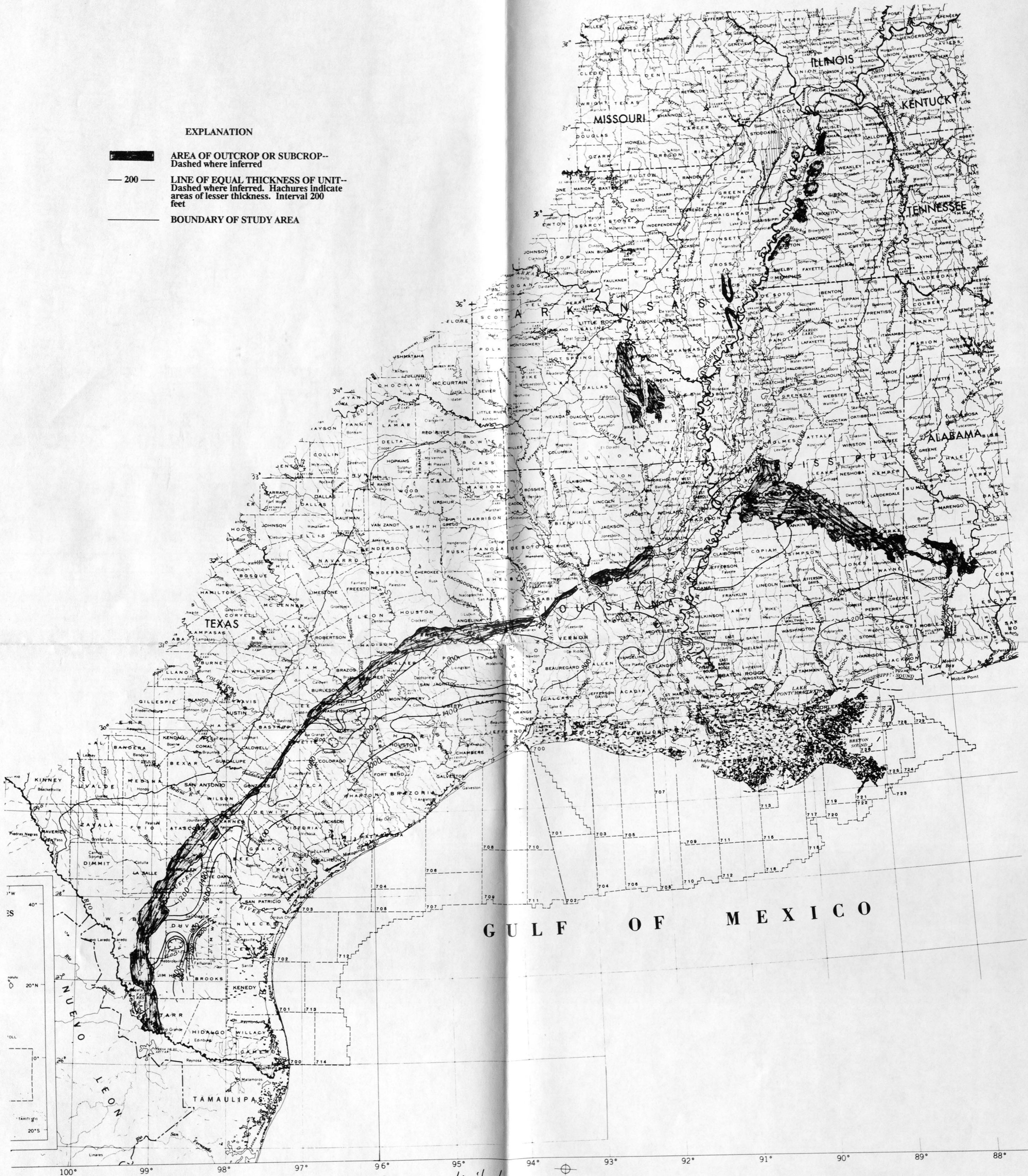
Figure 31. -- Thickness of the Vicksburg and Jackson Groups undivided.
