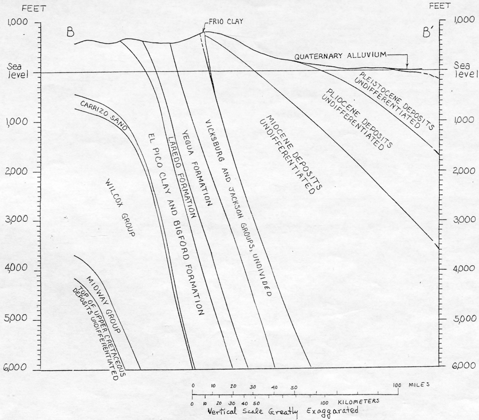
Figure 4.-- Geologic section B-B'.
