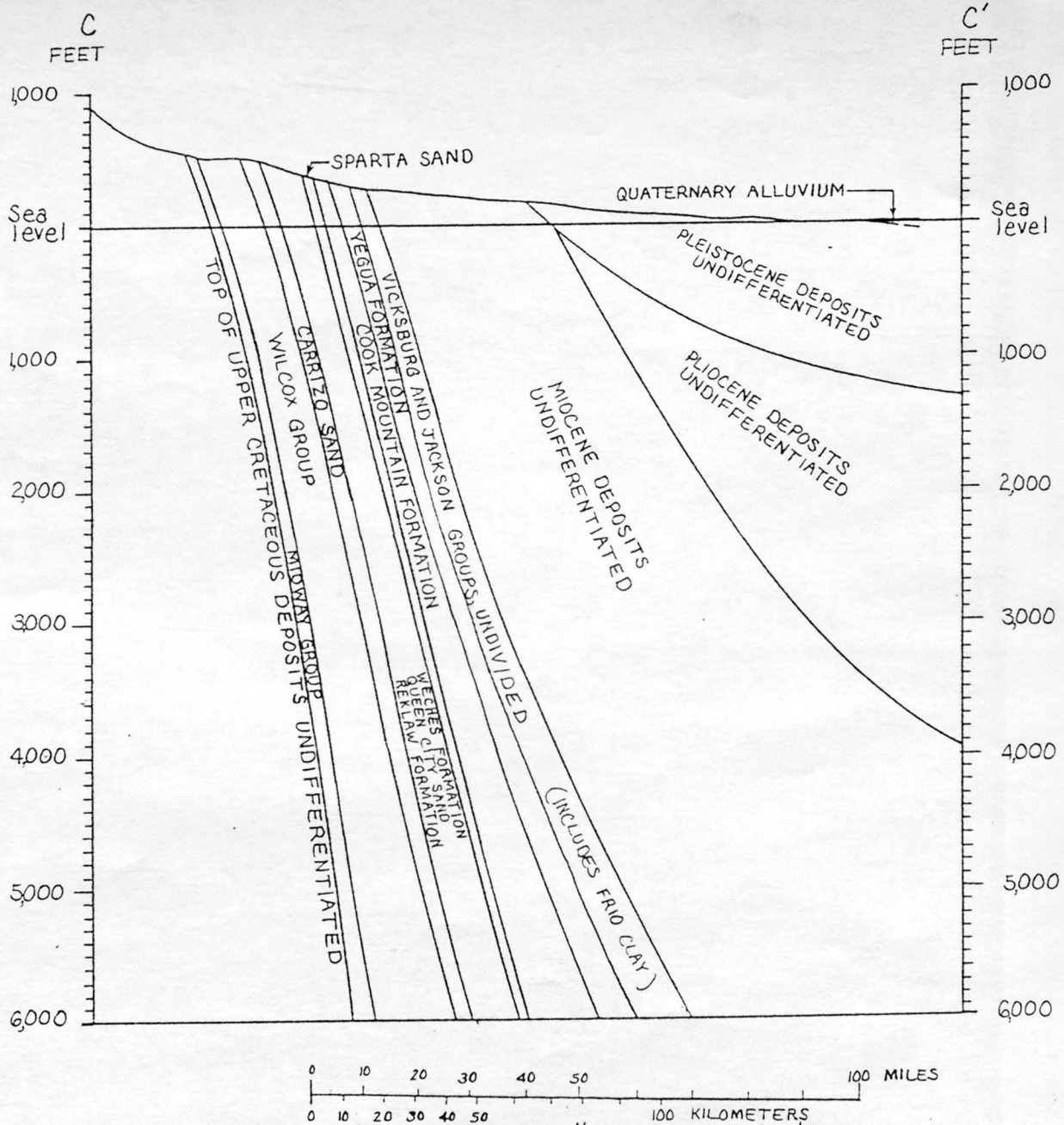
Vertical Scale Greatly Exaggerated Figure 5. -- Geologic section C-C'.
