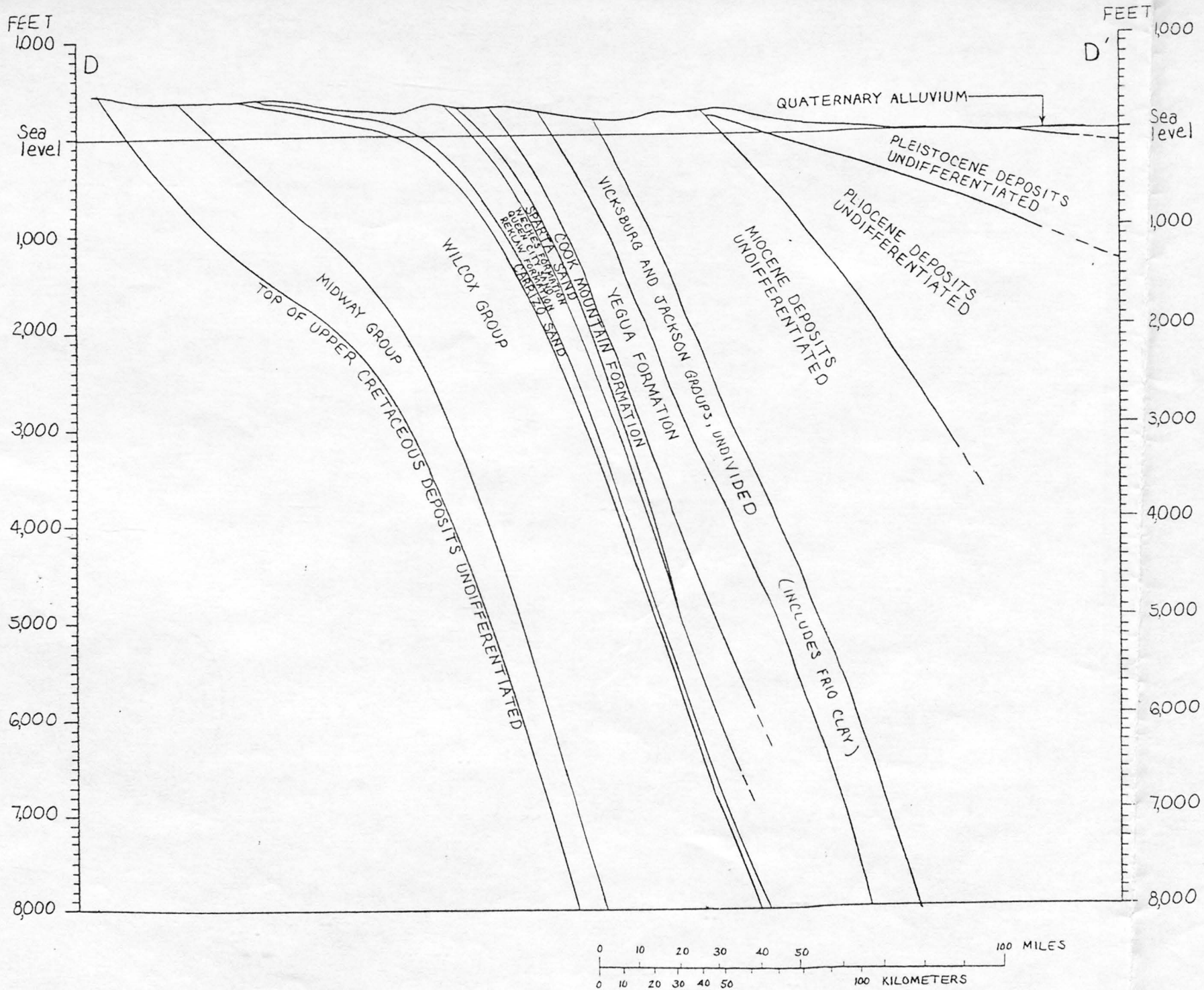
Figure 6.-- Geologic section D-D'.
