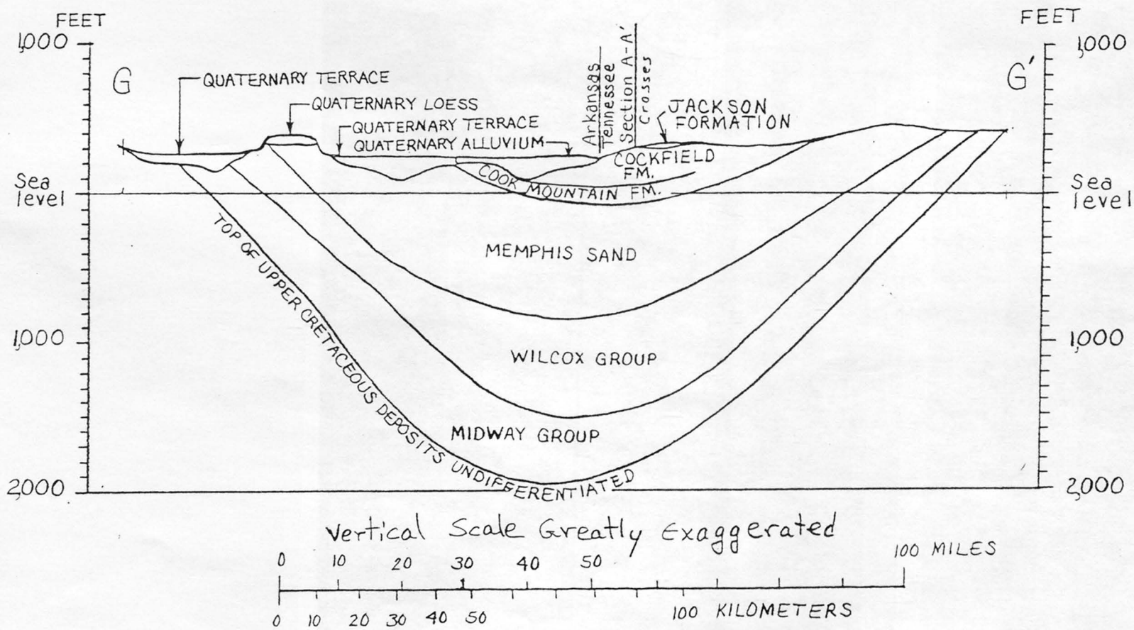
Figure 9.-- Geologic section G-G'.
