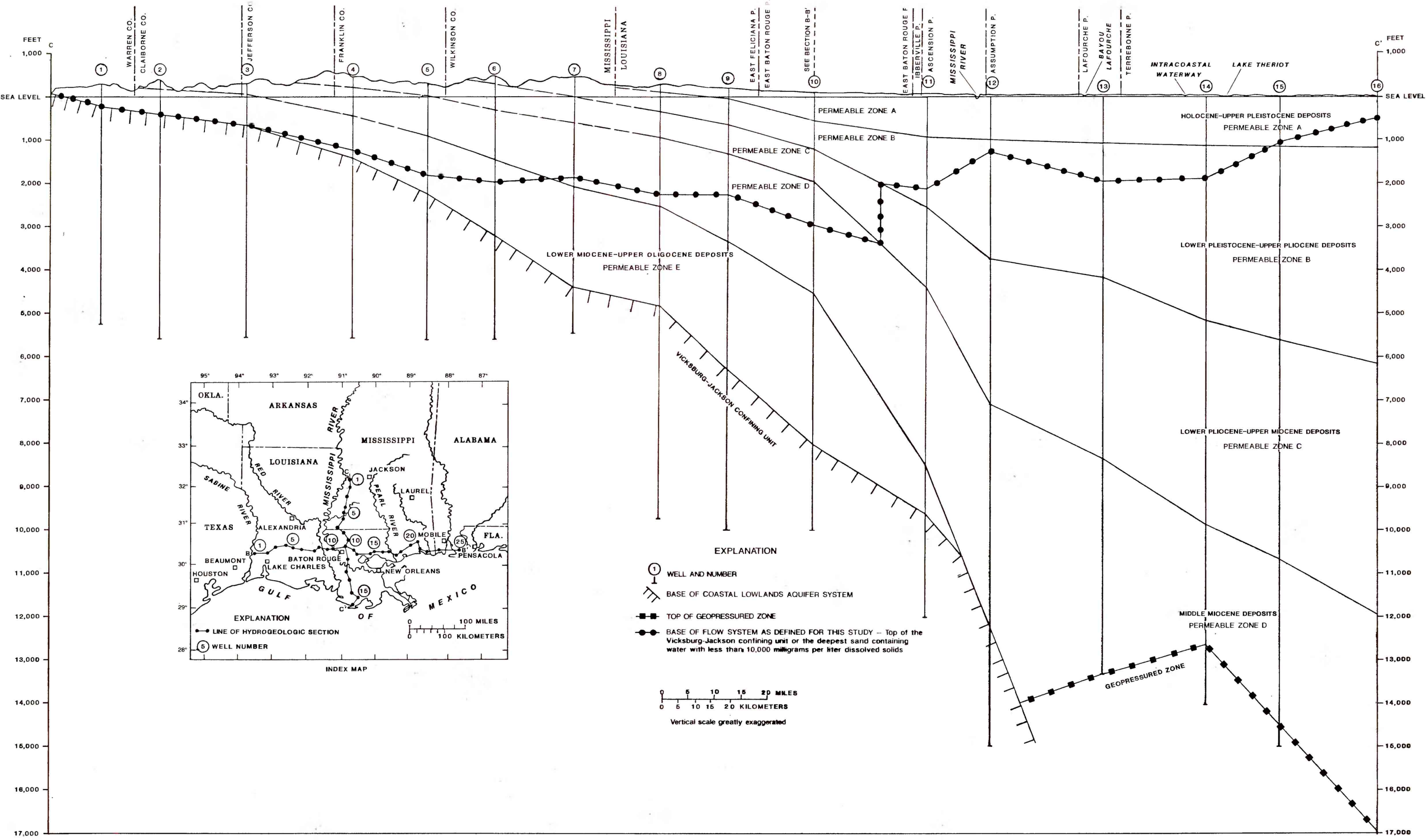
PLATE 2 NORTH-SOUTH HYDROGEOLOGIC SECTION C-C' OF THE COASTAL LOWLANDS AQUIFER SYSTEM SHOWING THE PERMEABLE ZONES AND LIMITS OF THE FLOW SYSTEM IN MISSISSIPPI AND LOUISIANA
