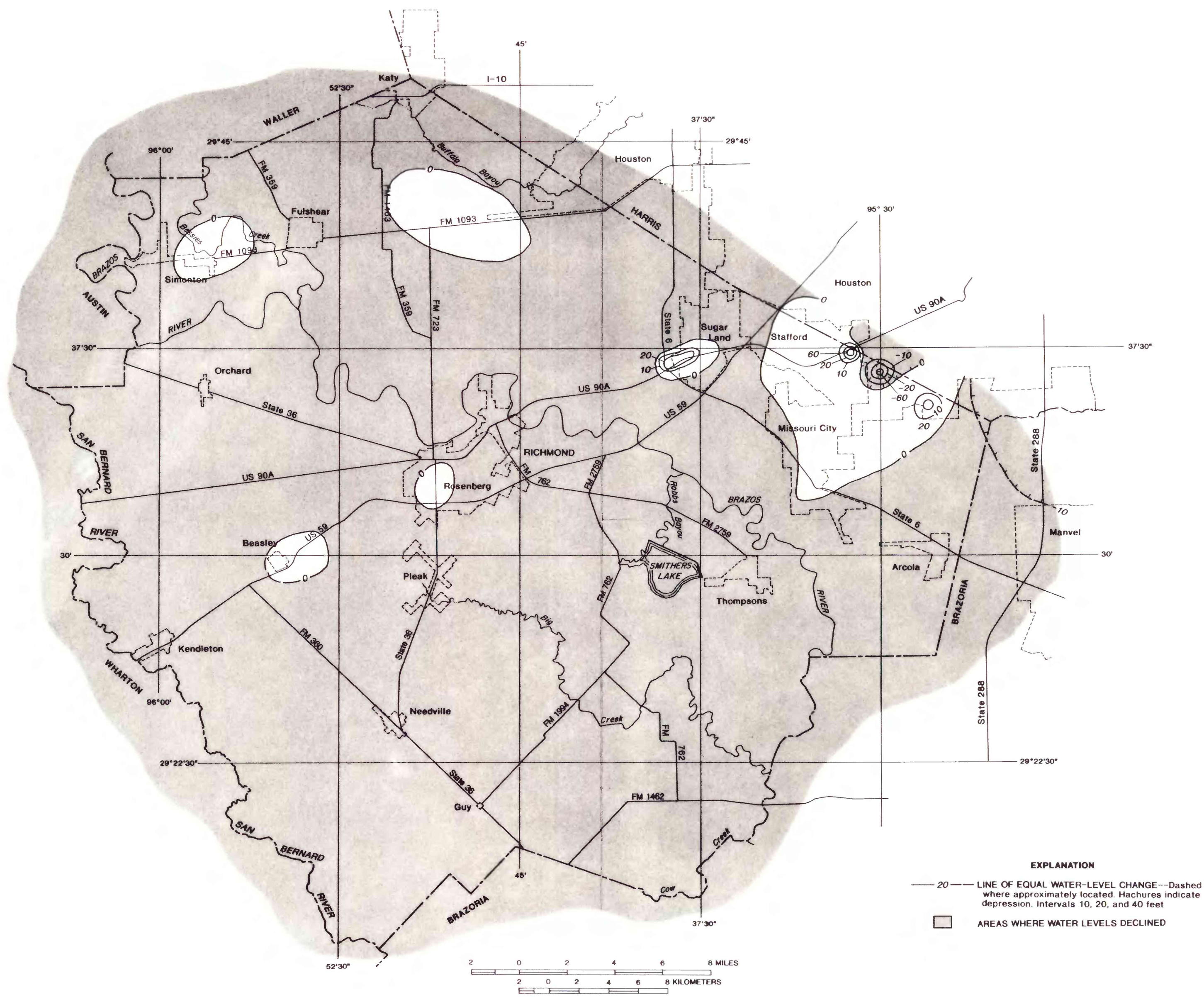
Figure 2.--Map showing approximate change in water levels in wells completed in the Evangeline aquifer, 1990-91
