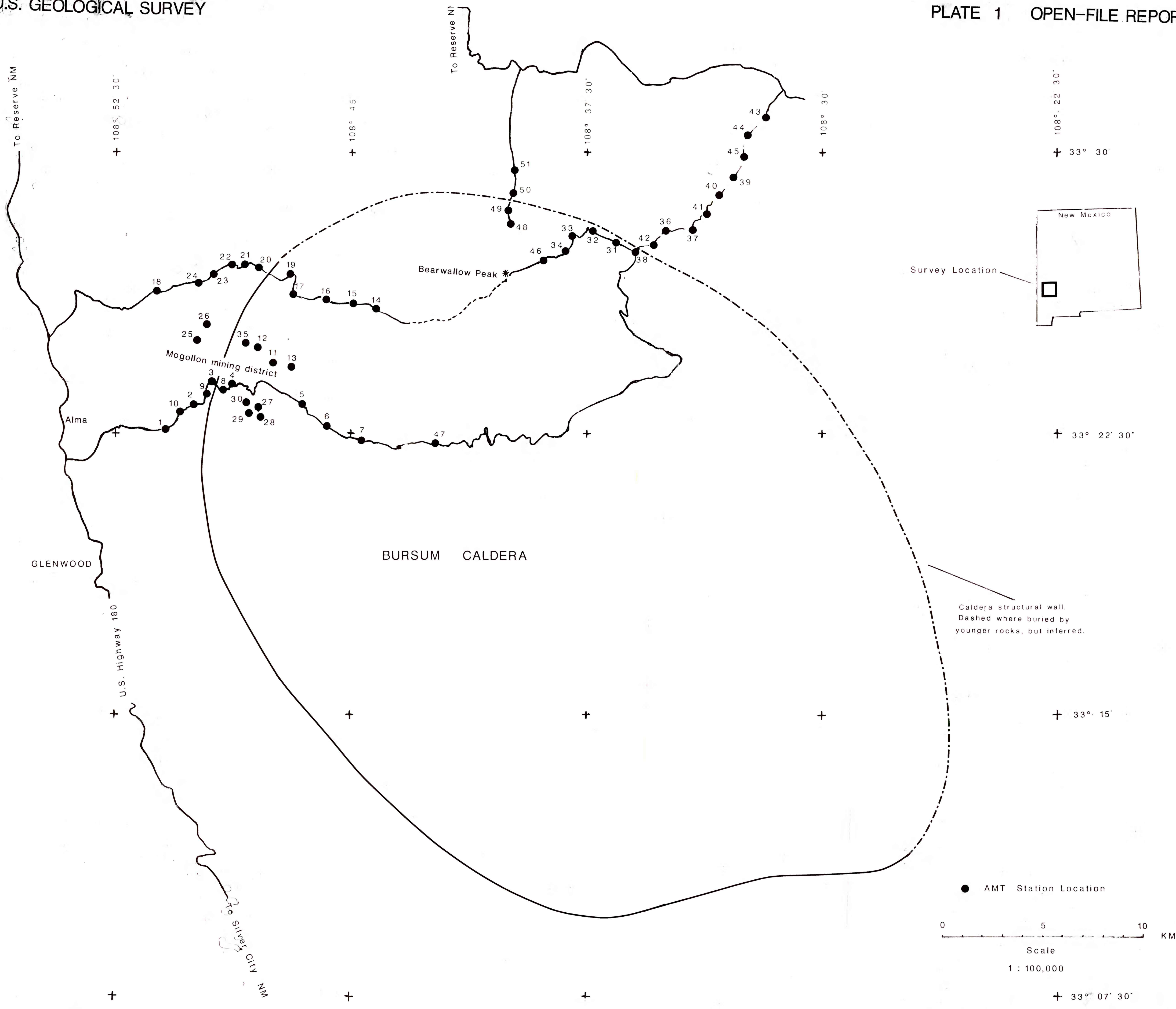
Plate 1--Map showing location of audio-magnetotelluric (AMT) stations, Mogollon mining district, west central New Mexico
