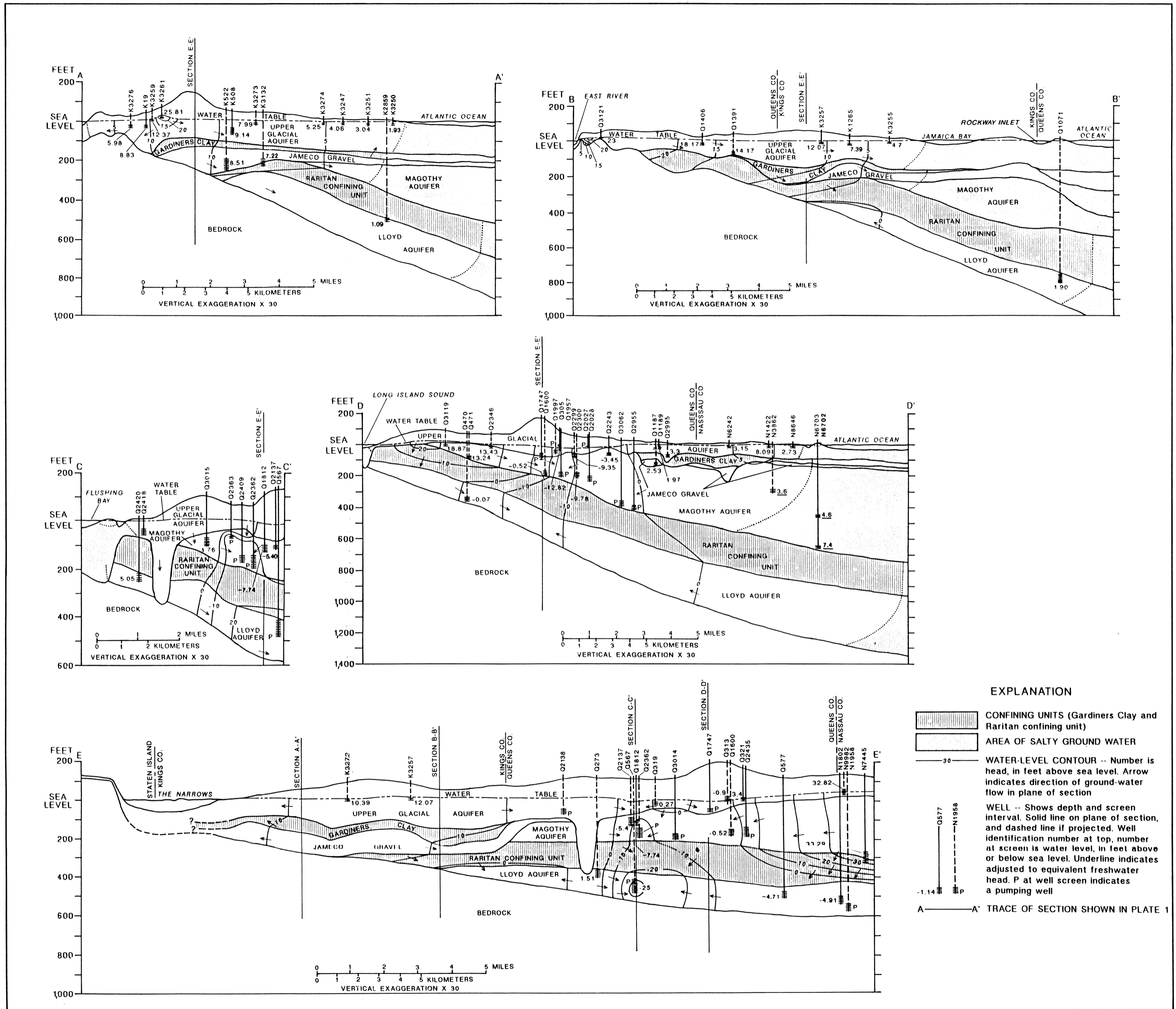
HEAD DISTRIBUTION WITHIN MAJOR HYDROGEOLOGIC SECTION
