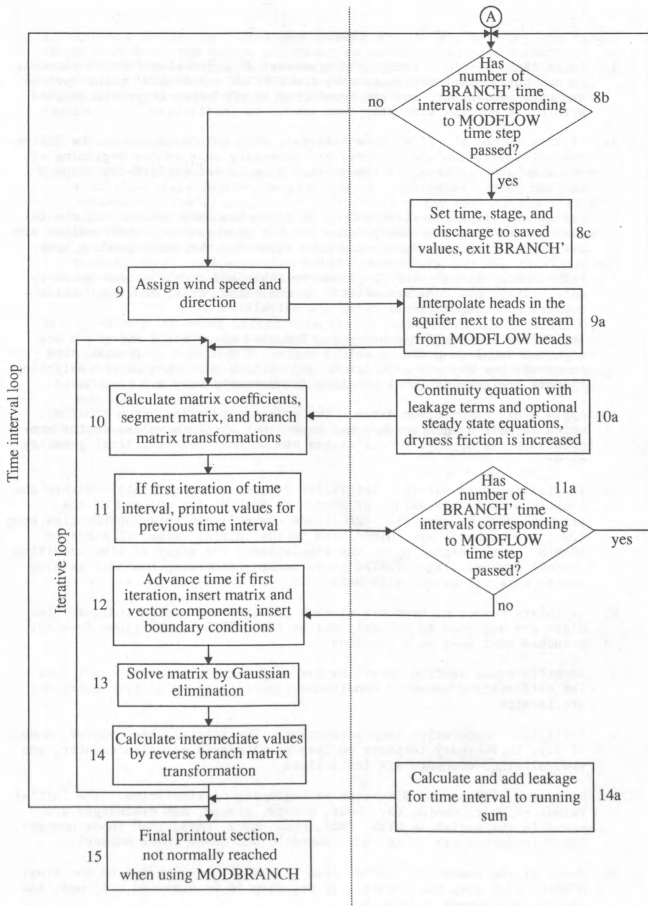
Figure 10. Flowchart of modified BRANCH'--Continued.
