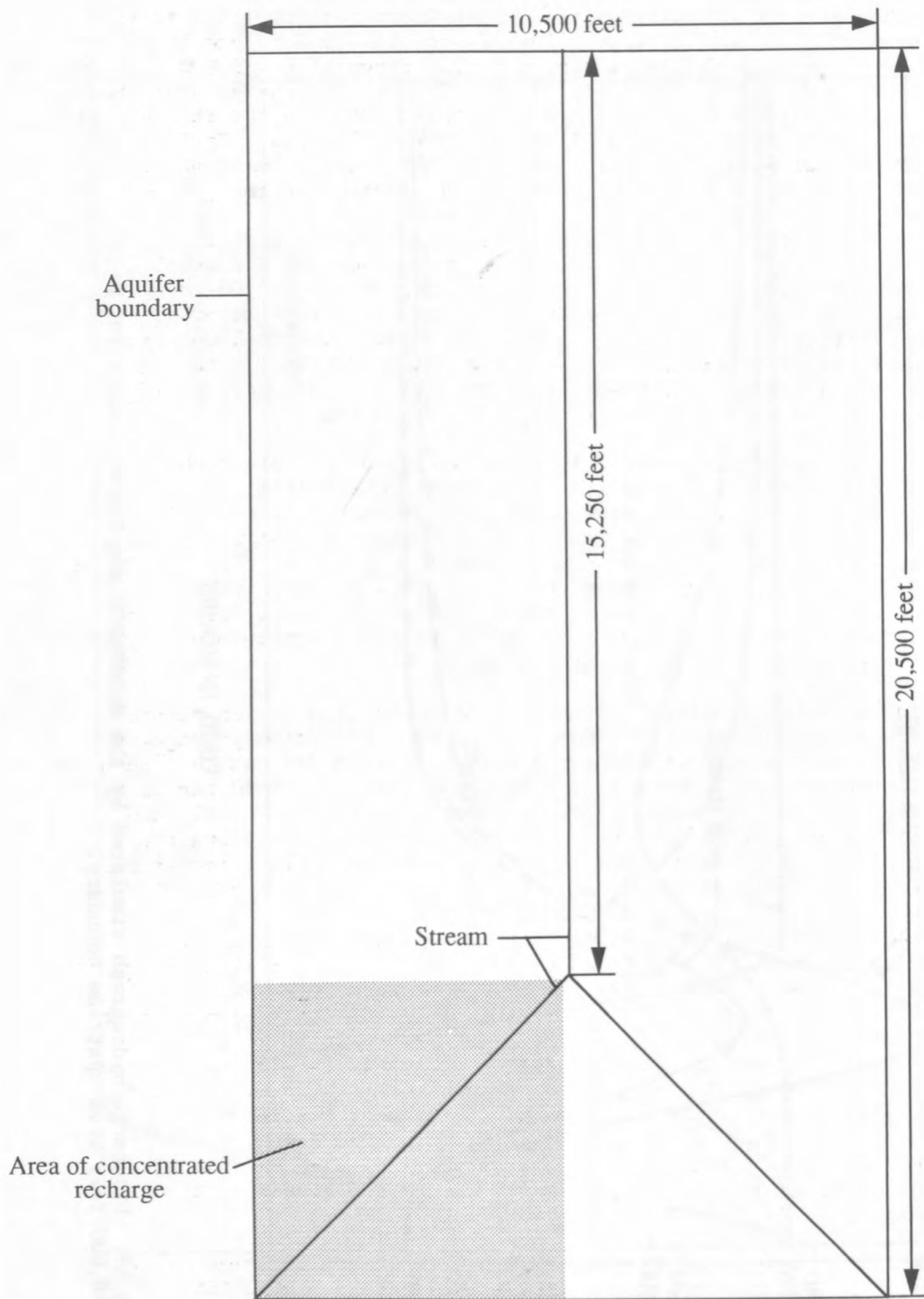
Figure 14. Aquifer and river layout for steady-state problem.
