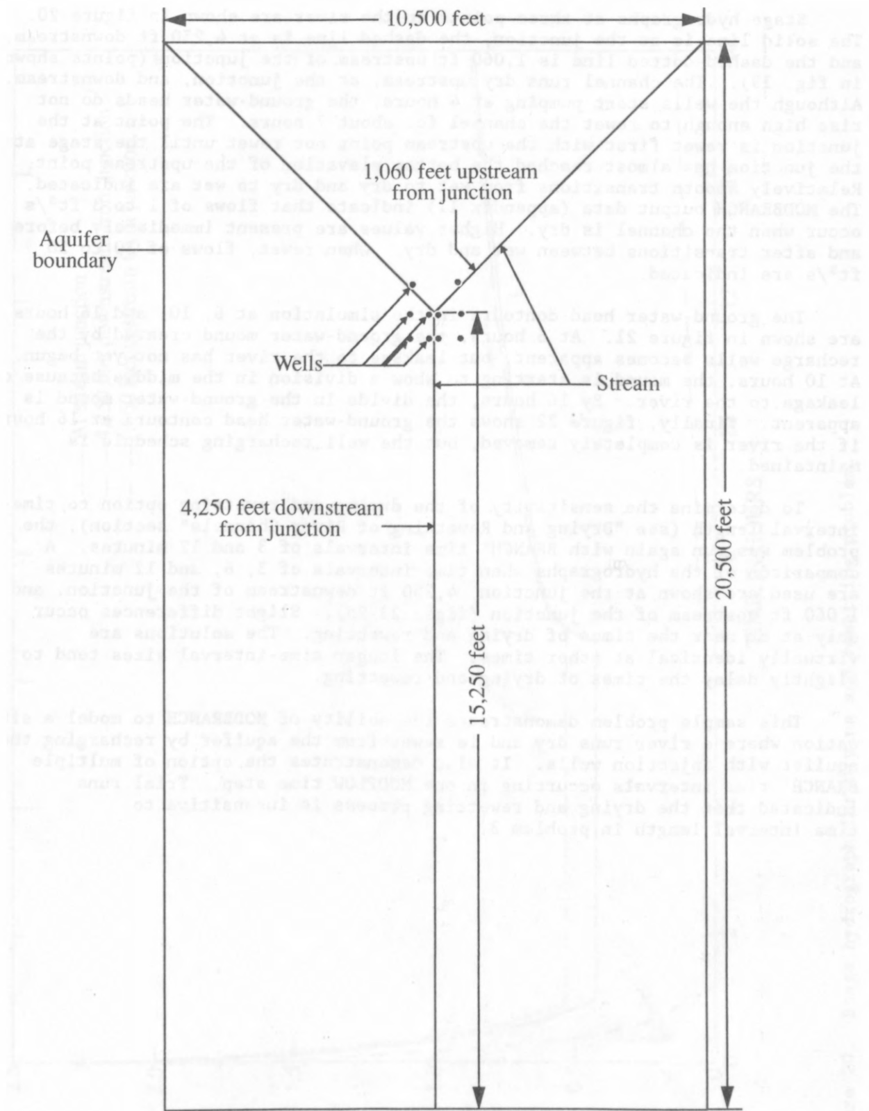
Figure 19. Aquifer, river, and well layout for drying and rewetting problem.
