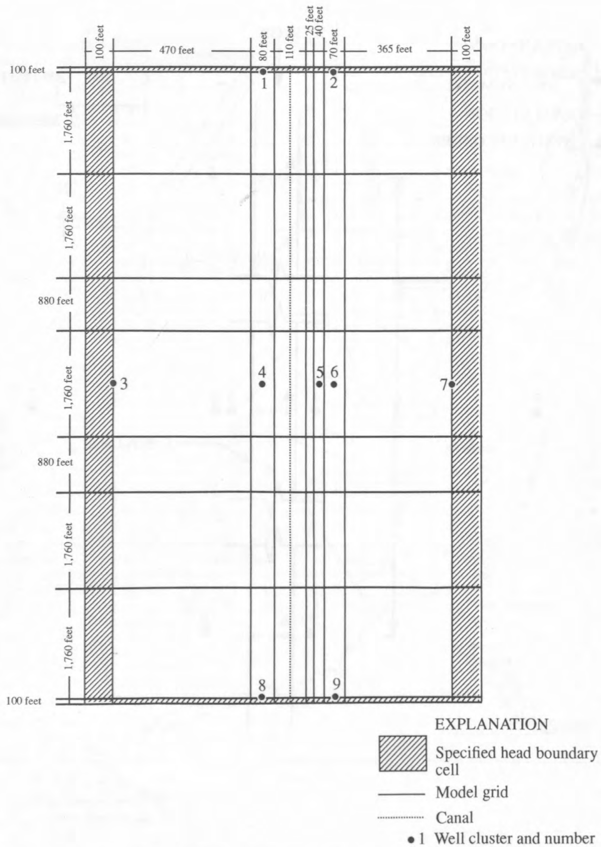
Figure 28. Model aquifer grid for the L-31N Canal field problem.
