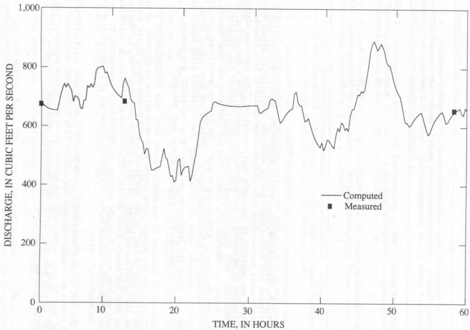
Figure 30. Hydrograph showing measured and computed discharge at L-31N Canal.
