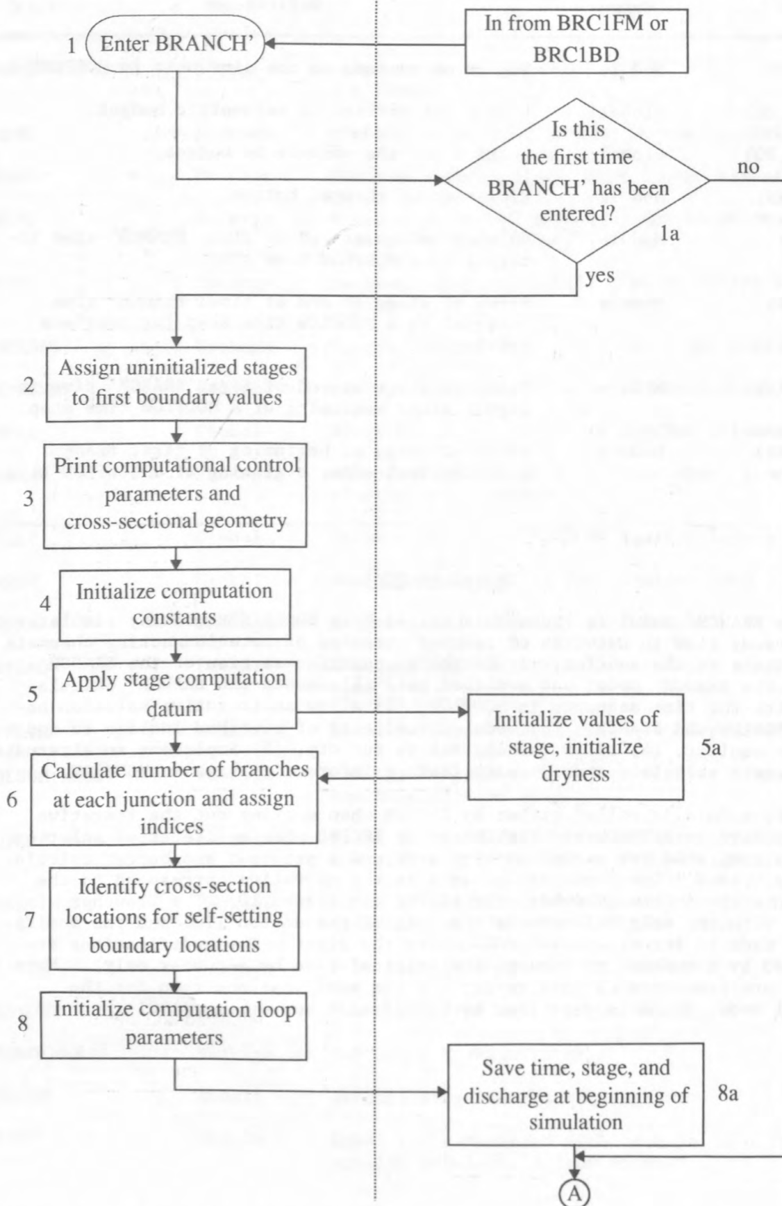
Figure 10. Flowchart of modified BRANCH'.
