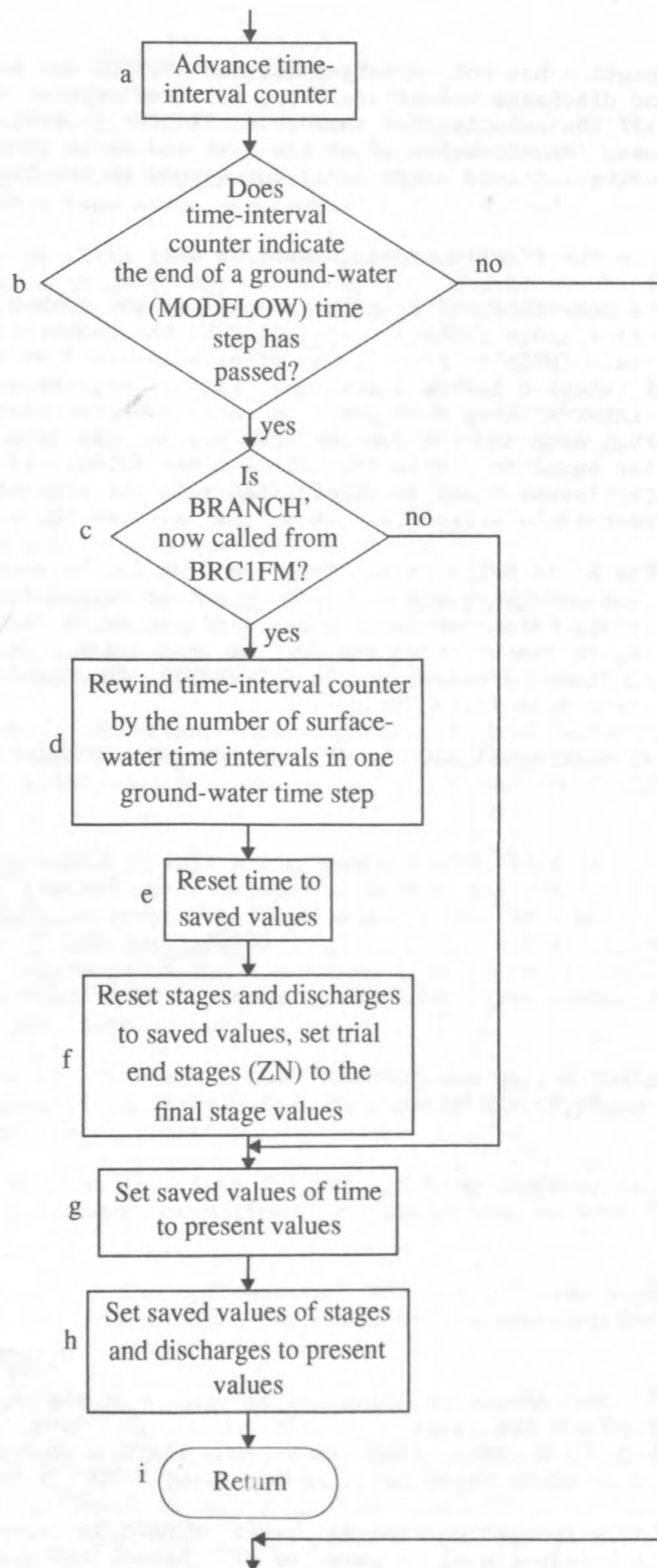
Figure 11. Expanded flowchart of step 8B in Branch'.
