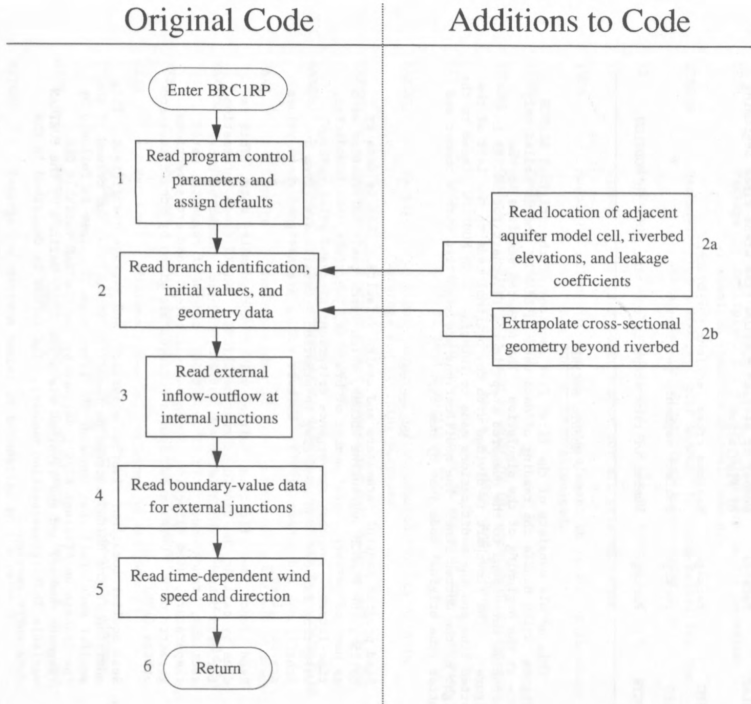
Figure 7. Flowchart of data entry module (BRC1RP).
