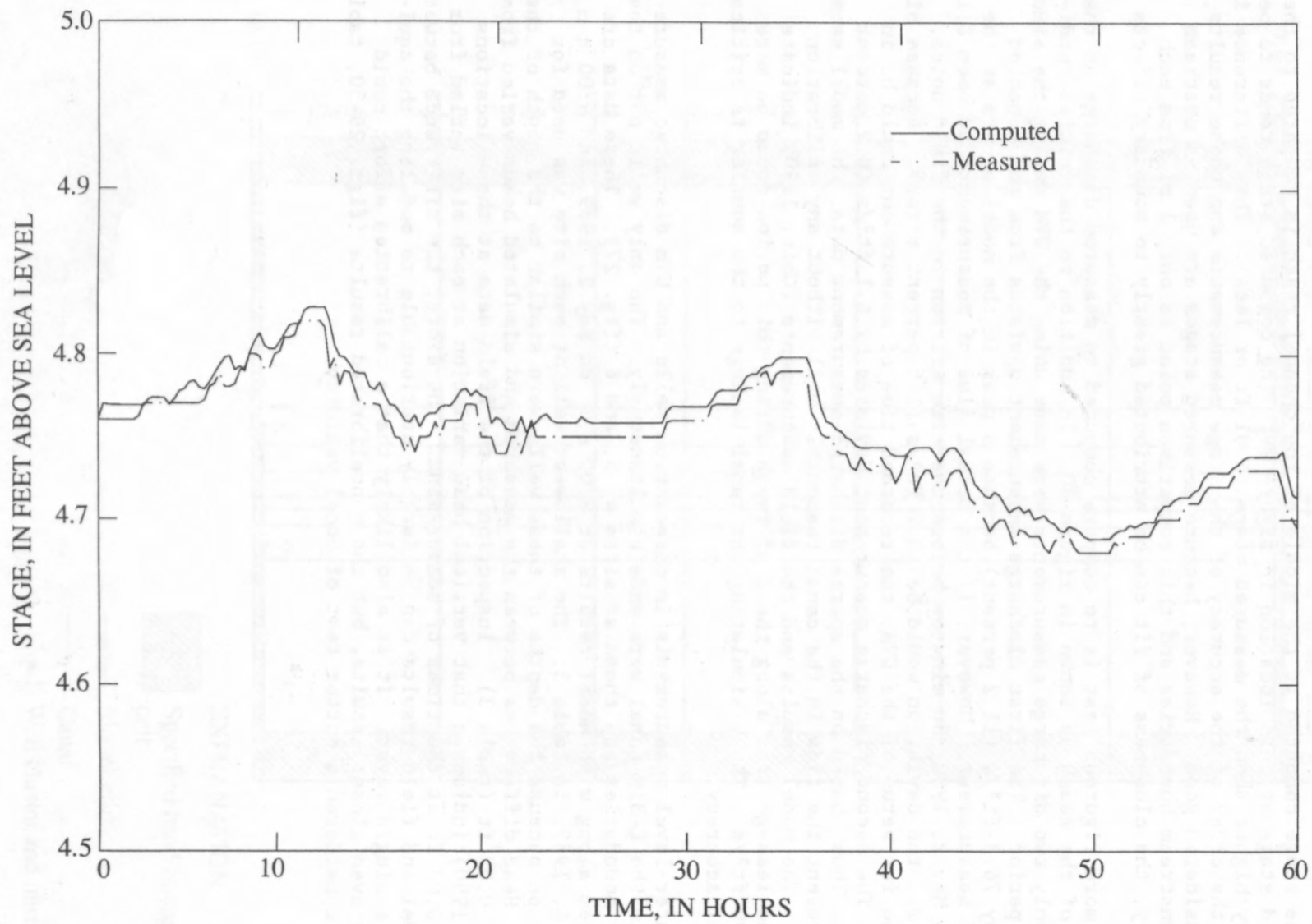
Figure 29. Hydrograph showing measured and computed stage at L-31N Canal at mile 1.
