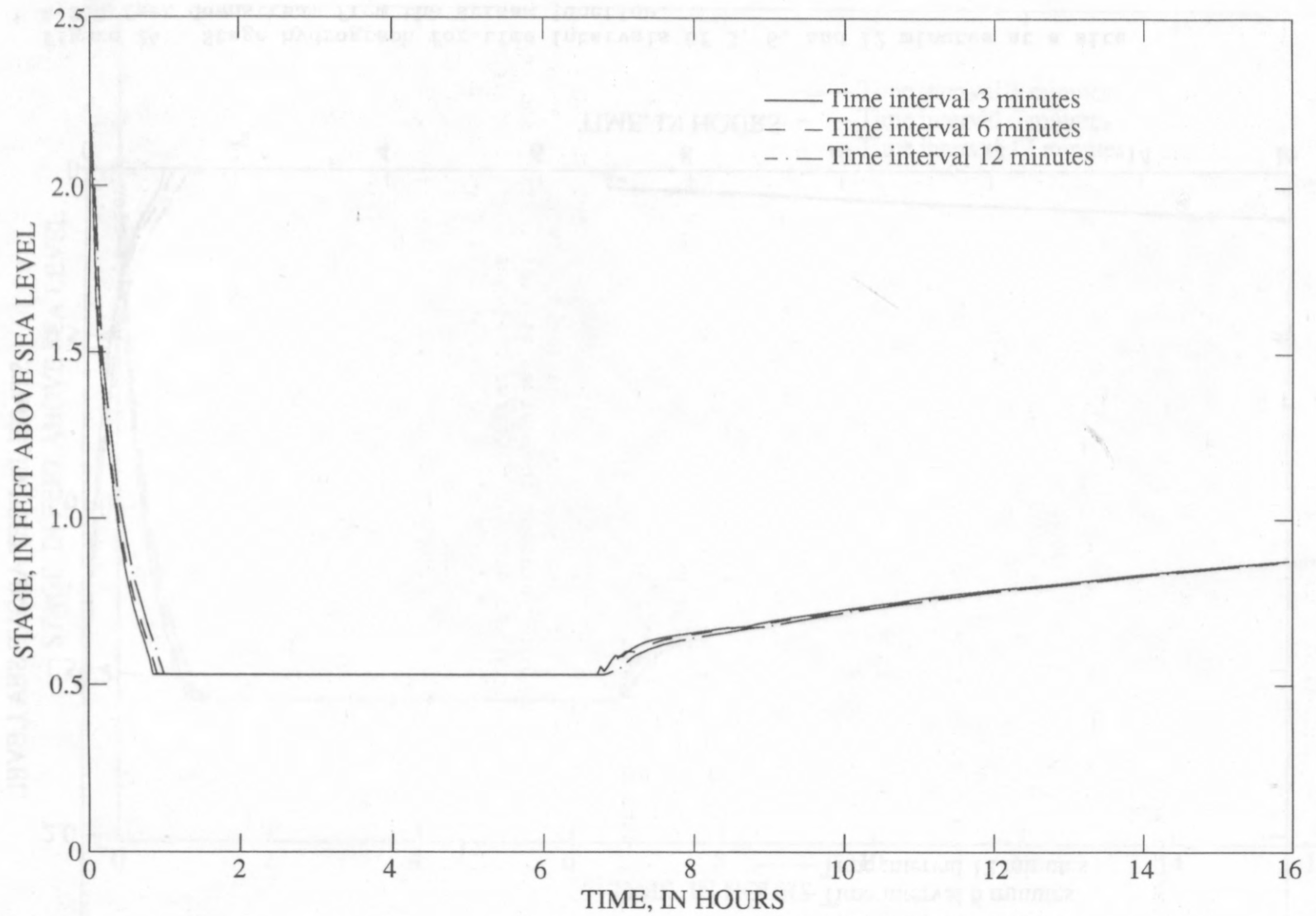
Figure 25. Stage hydrograph for time intervals of 3, 6, and 12 minutes at a site
