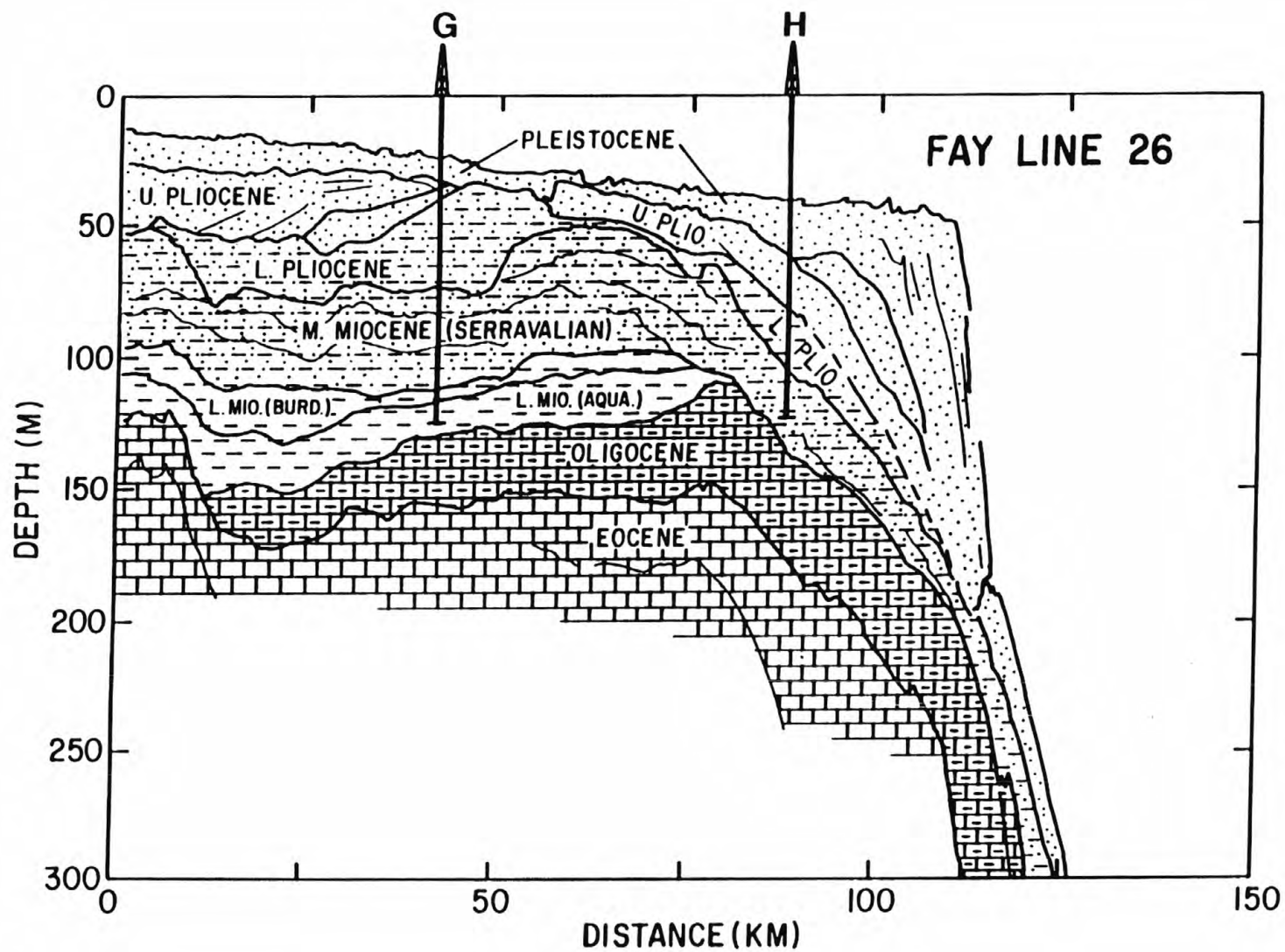
Fig. III-15. W to E section across shelf and slope. (Fay Line 26). Modified from data in Popenoe (1991).
