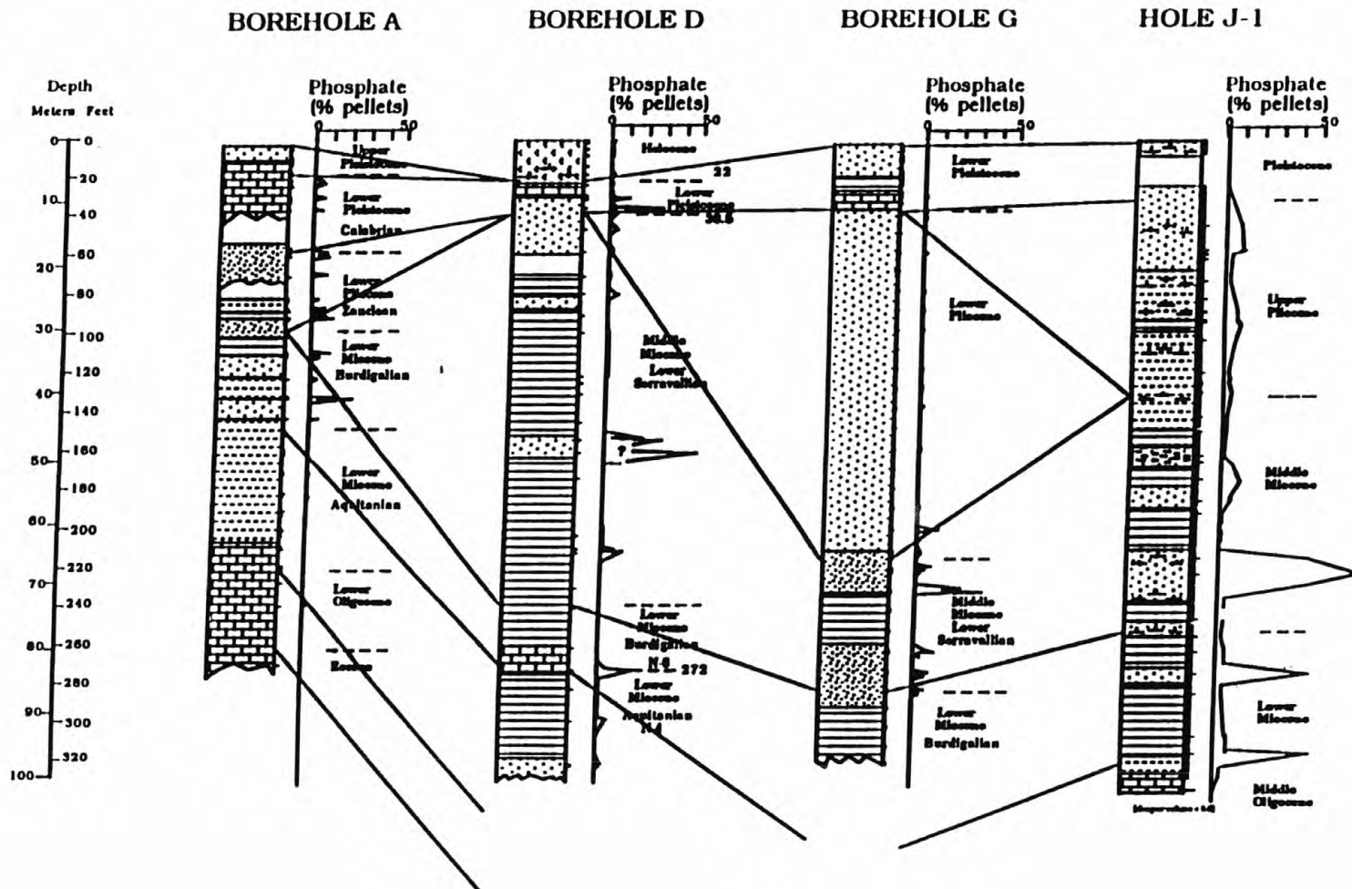
Fig. III-13. North to South stratigraphic profile
