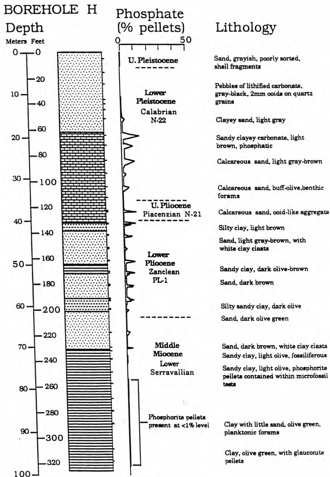
Fig. III-8. Core log, Borehole H
