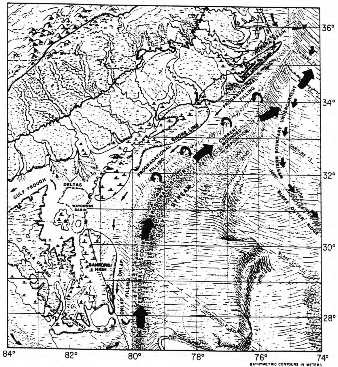
Figure VI-4. Paleogeographic reconstruction of the southeastern Atlantic margin early Burdigalian time (from Popenoe, 1990).
