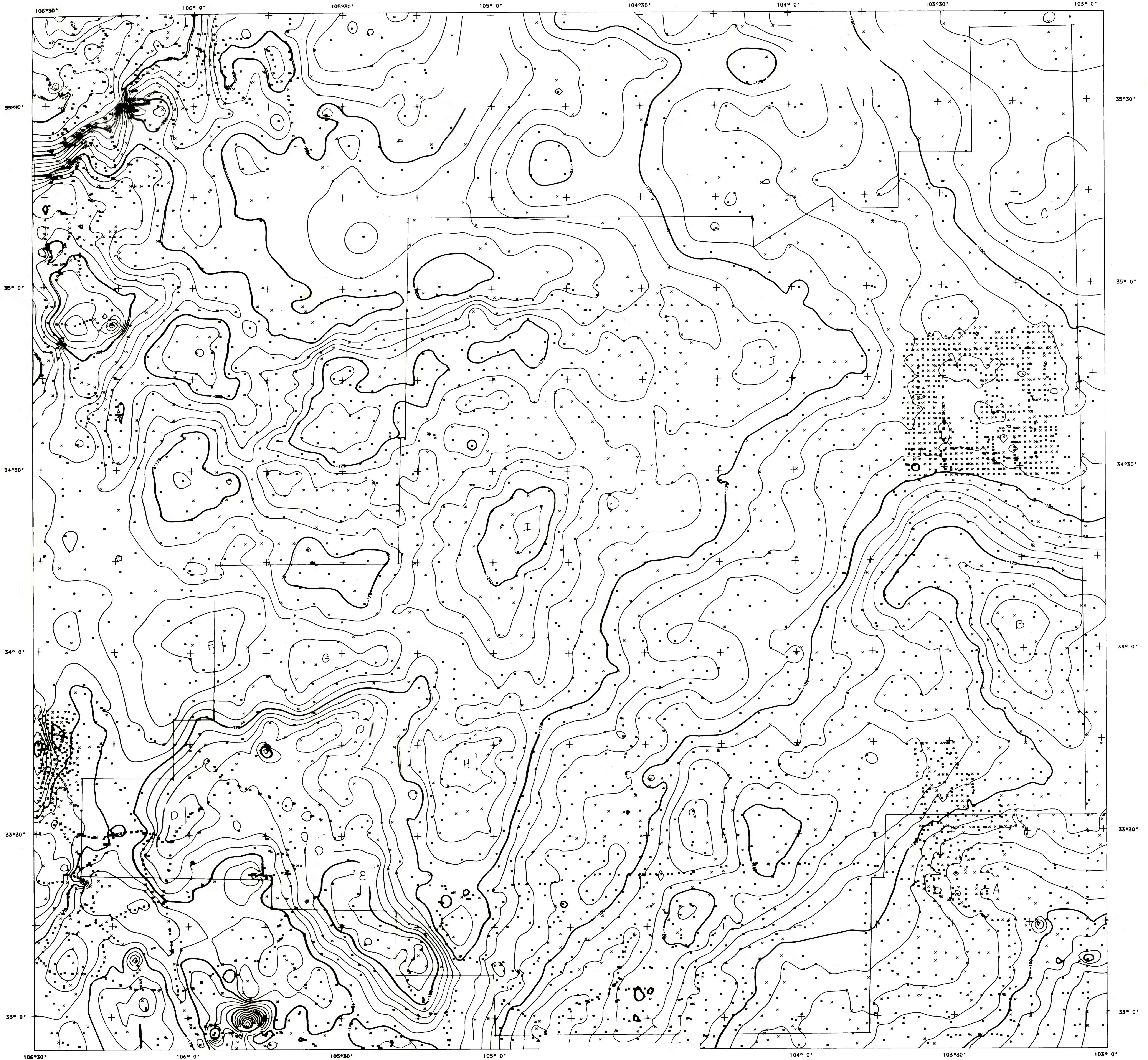
MAP F.--Complete Bouguer gravity anomaly map of the Roswell Resource Area (scale 1:500,000; Contour Interval (CI) = 5mGal)
