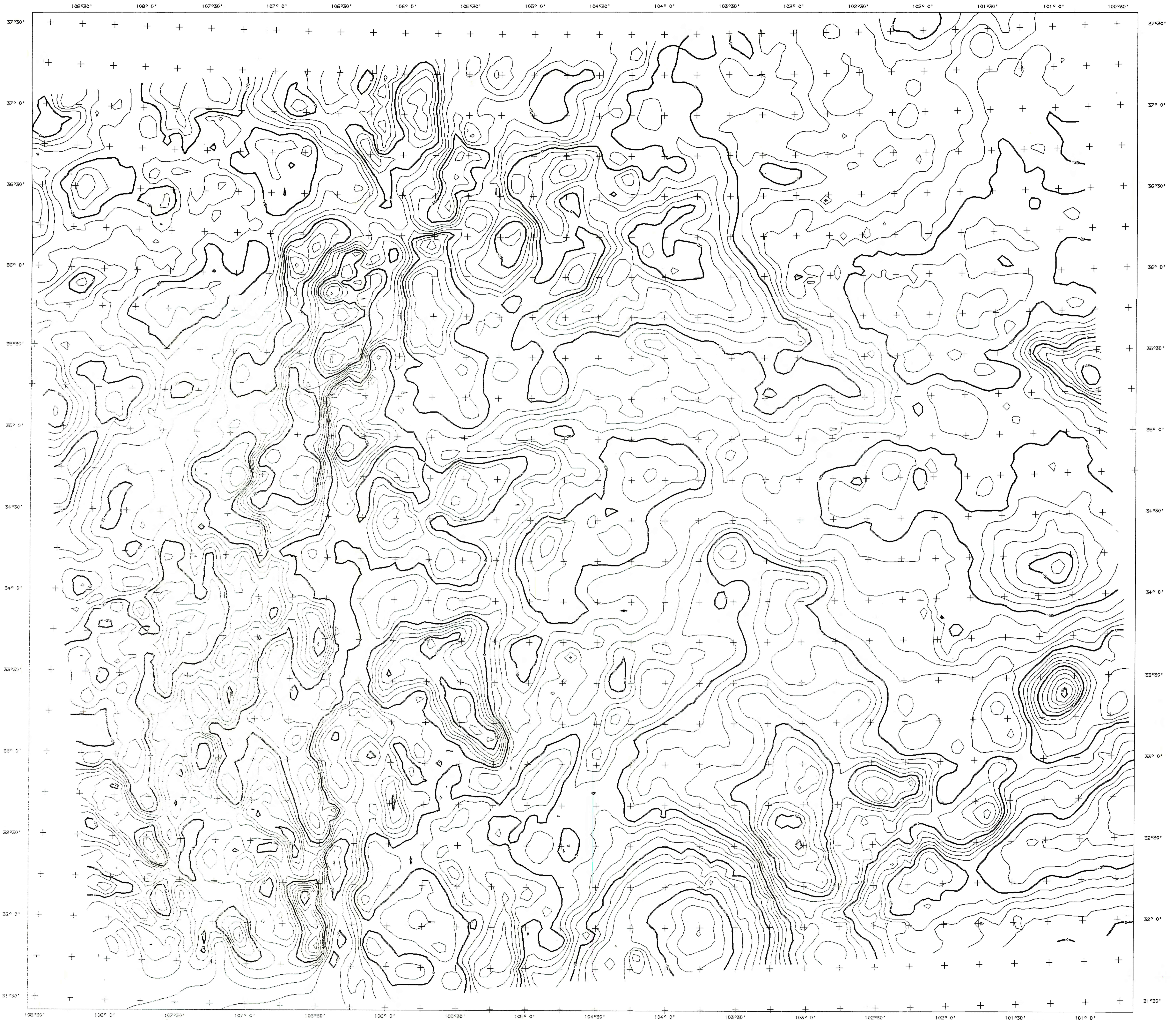
MAP H.-- Isostatic gravity map of the Roswell Resource Area By Dolores M. Kulik 1992
