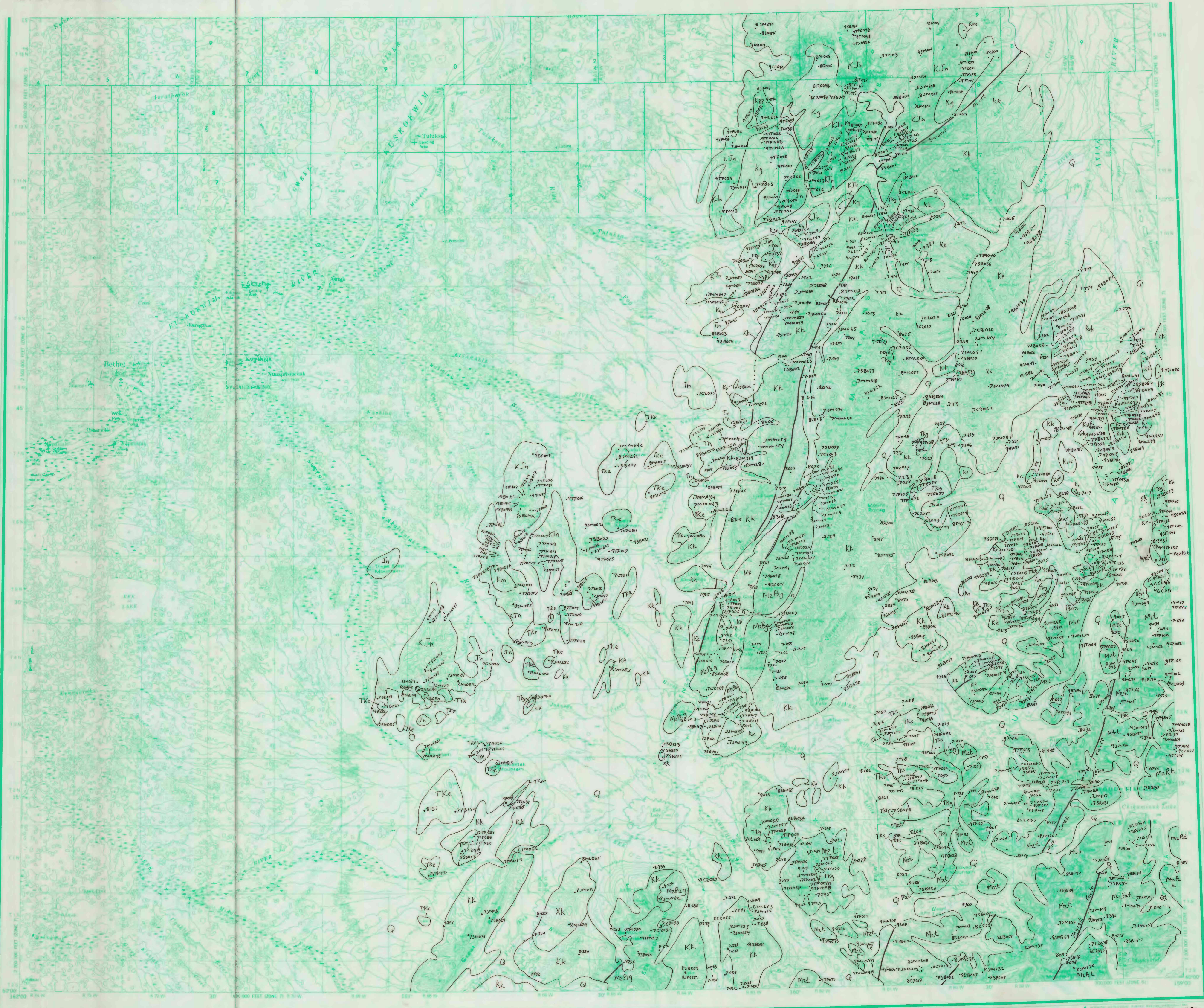
GEOLOGY SIMPLIFIED FROM BOX AND OTHERS, 1972
