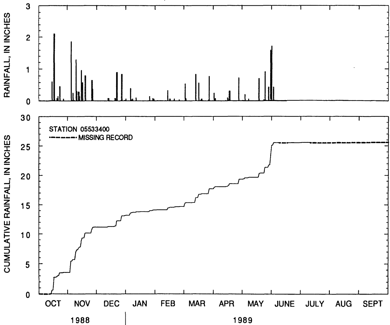
Figure 9.--Daily rainfall totals and cumulative rainfall at Sawmill Creek near Lemont, Illinois, water year 1989.
