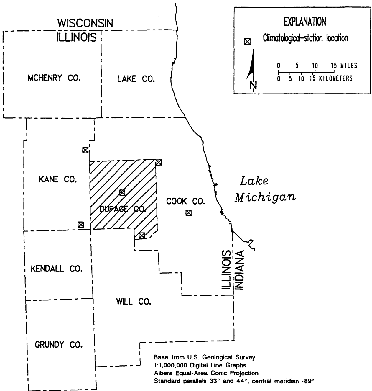
Figure 2.--Locations of climatological stations in and near Du Page County, Illinois.
