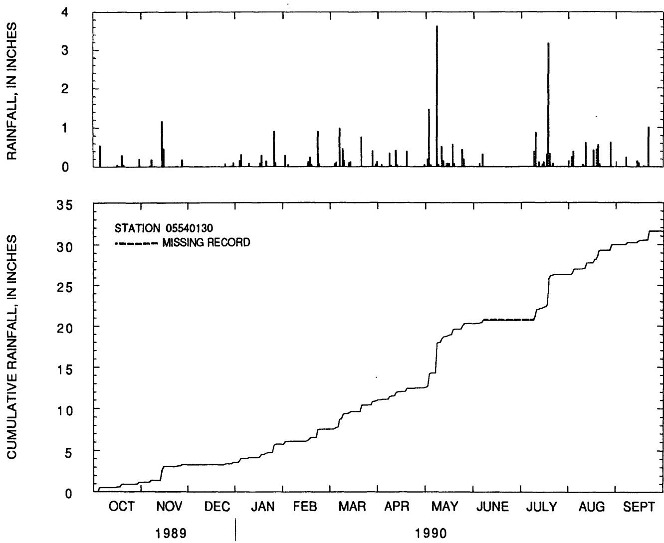
Figure 19.--Daily rainfall totals and cumulative rainfall at West Branch Du Page River near Naperville, Illinois, water year 1990.
