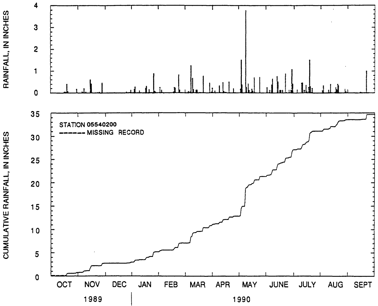
Figure 28.--Daily rainfall totals and cumulative rainfall at St. Joseph Creek at Lisle, Illinois, water year 1990.
