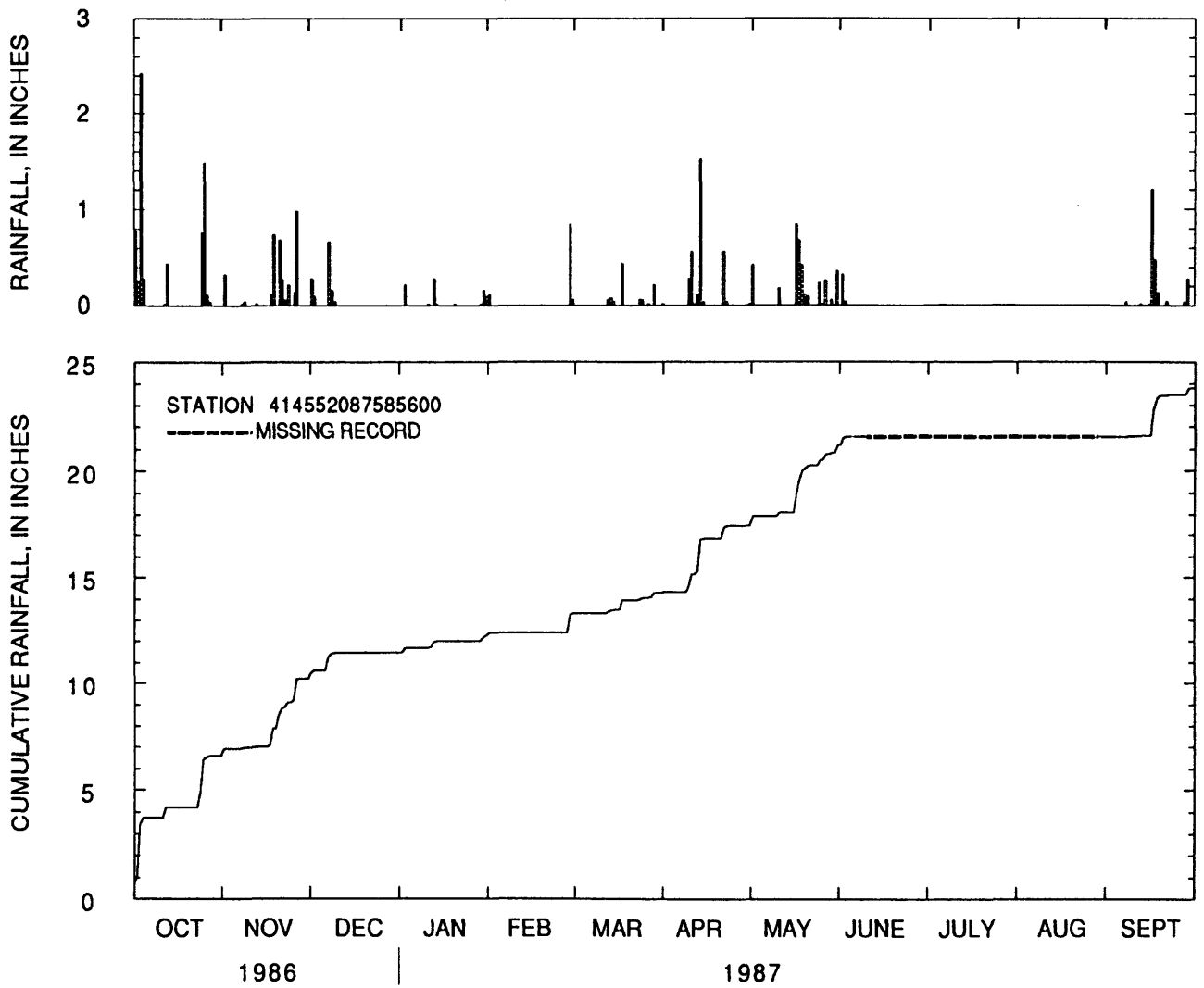
Figure 35.--Daily rainfall totals and cumulative rainfall at Clarendon Hills Cemetery at Darien, Illinois, water year 1987.
