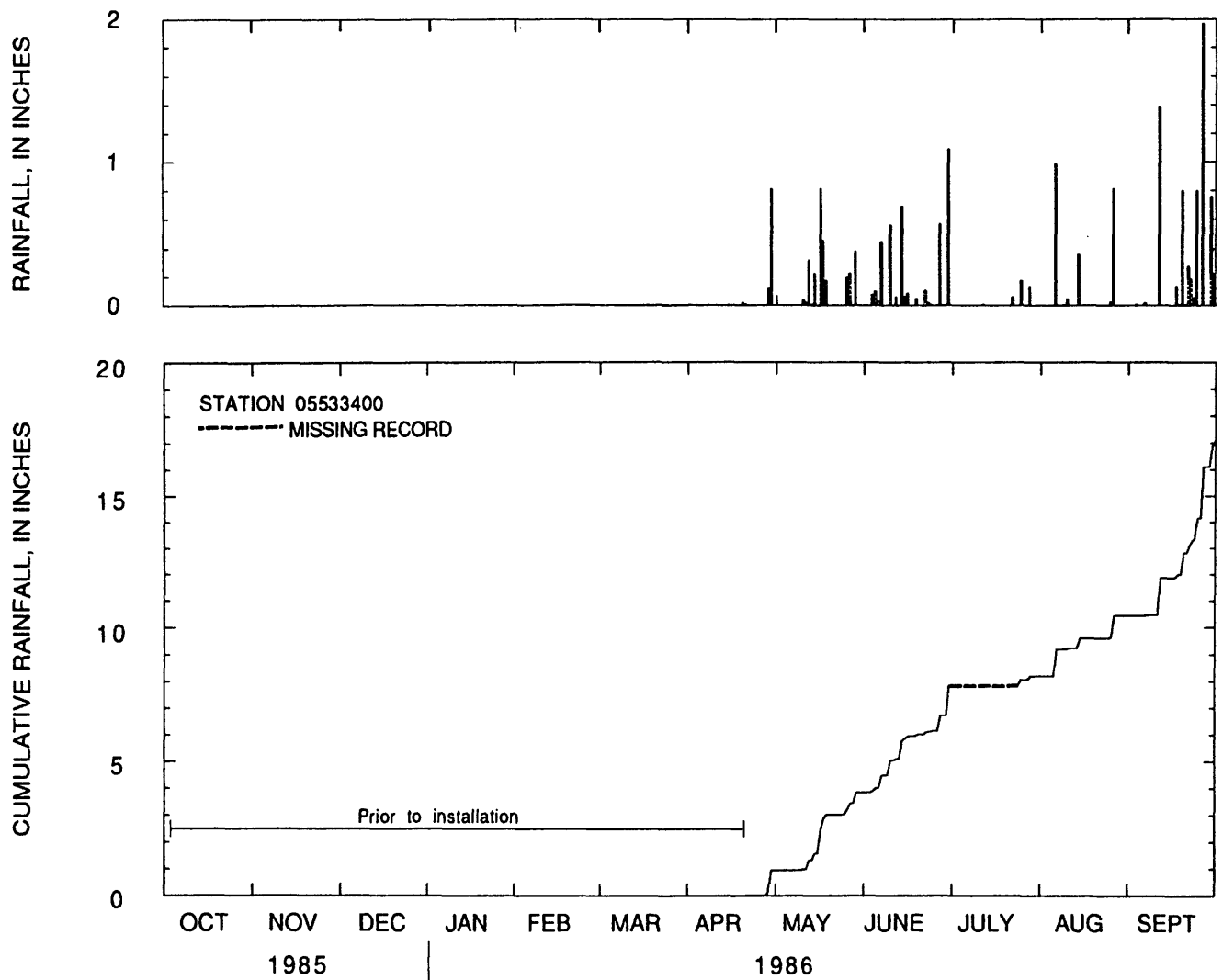
Figure 6.--Daily rainfall totals and cumulative rainfall at Sawmill Creek near Lemont, Illinois, water year 1986.
