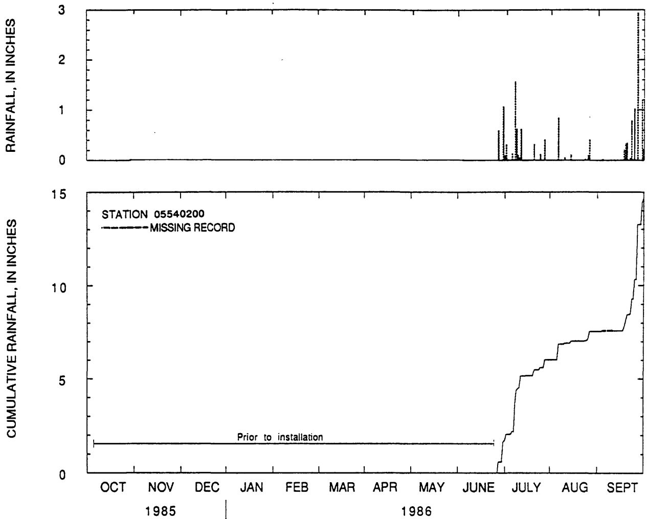
Figure 24.--Daily rainfall totals and cumulative rainfall at St. Joseph Creek at Lisle, Illinois, water year 1986.
