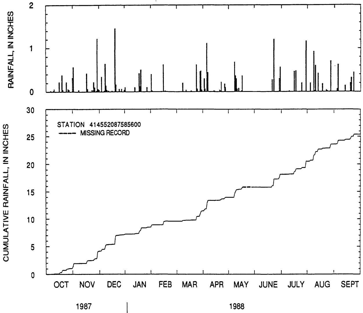
Figure 36.--Daily rainfall totals and cumulative rainfall at Clarendon Hills Cemetery at Darien, Illinois, water year 1988.
