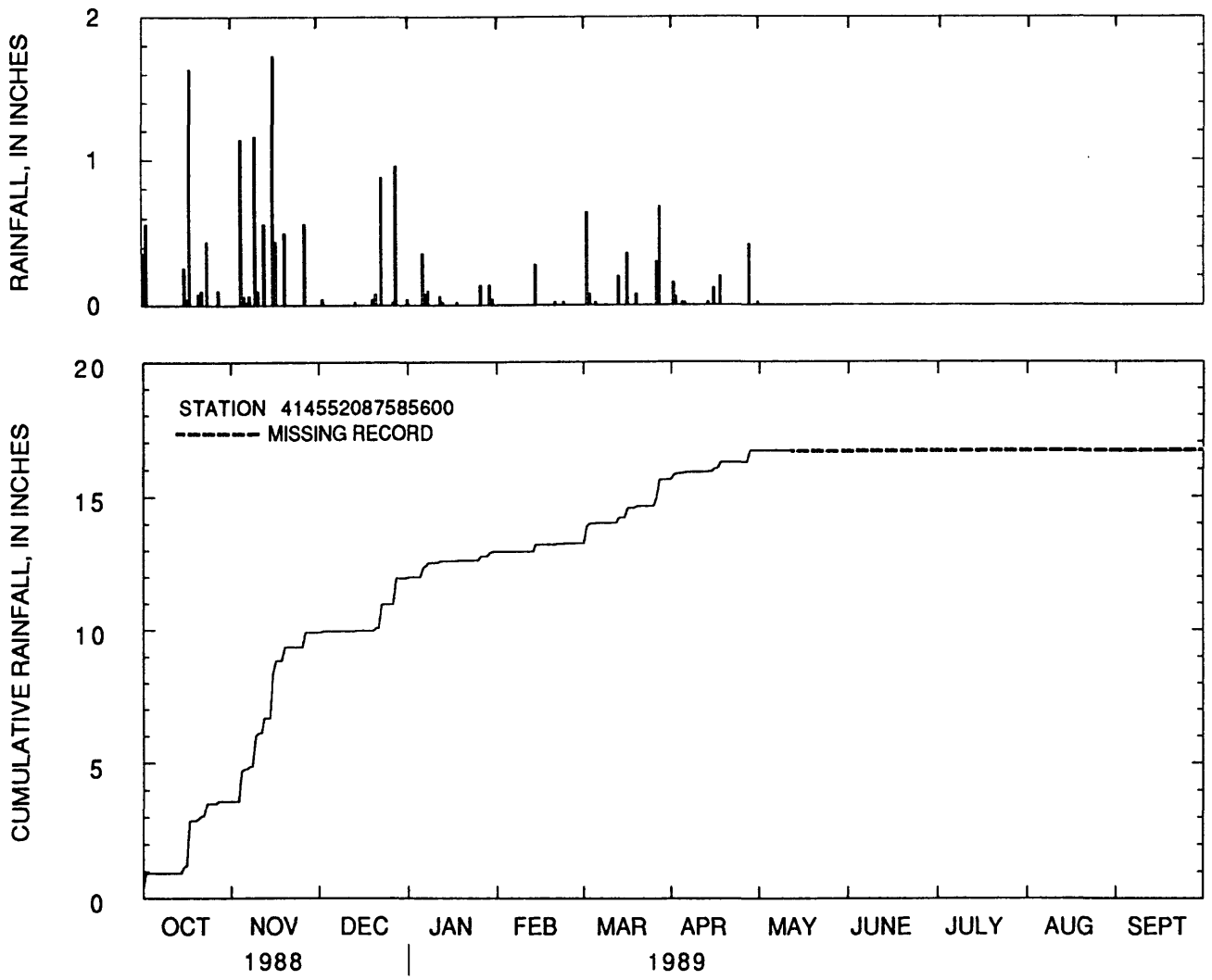
Figure 37.--Daily rainfall totals and cumulative rainfall at Clarendon Hills Cemetery at Darien, Illinois, water year 1989.
