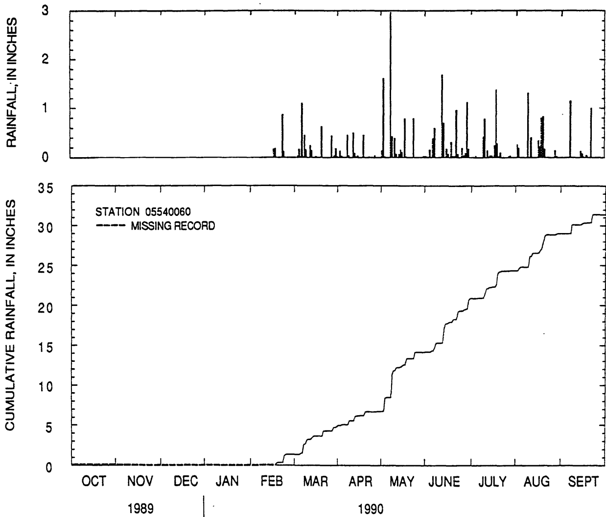
Figure 16.--Daily rainfall totals and cumulative rainfall at Kress Creek at West Chicago, Illinois, water year 1990.
