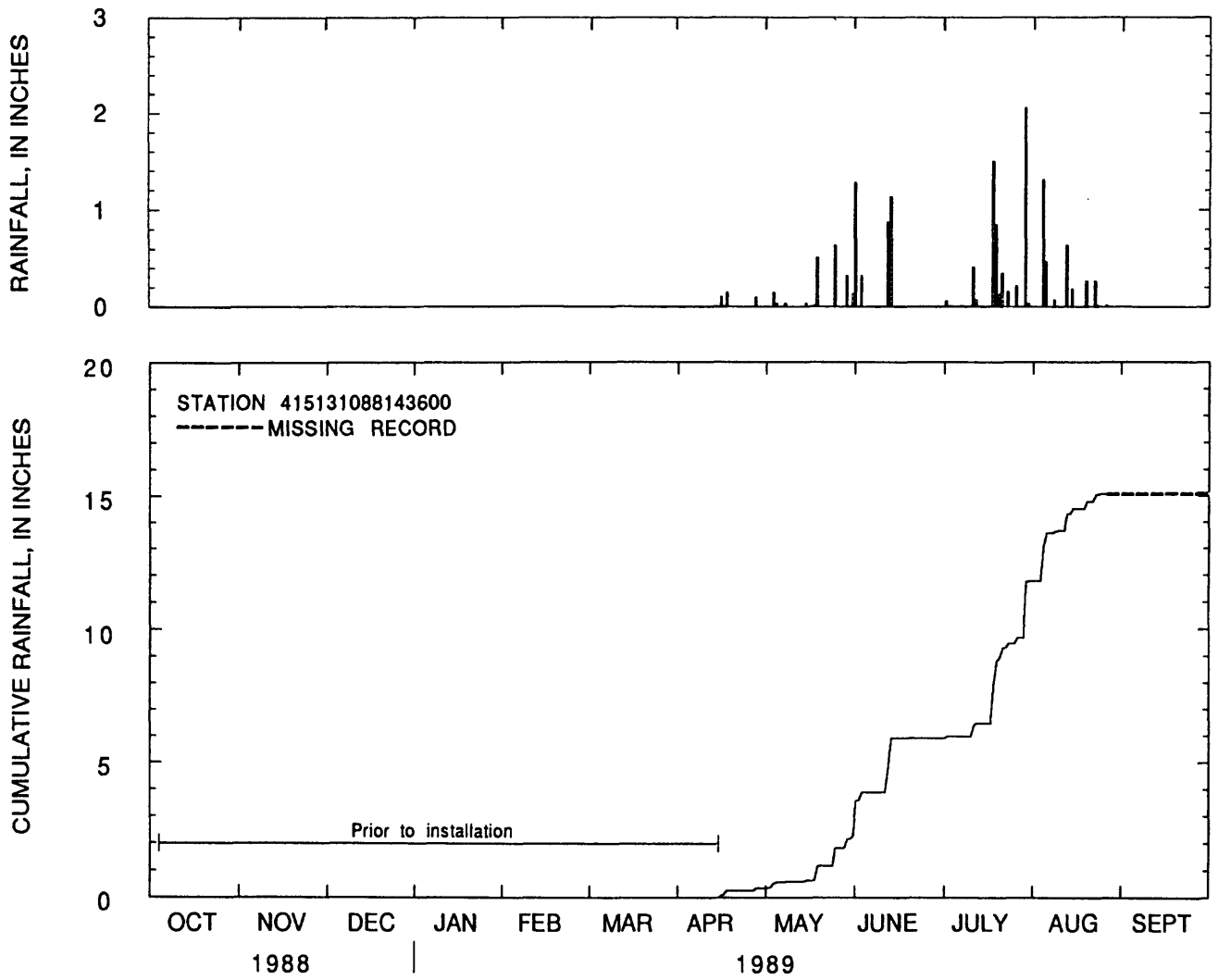
Figure 43.--Daily rainfall totals and cumulative rainfall at National Accelerator Laboratory near West Chicago, Illinois, water year 1989.
