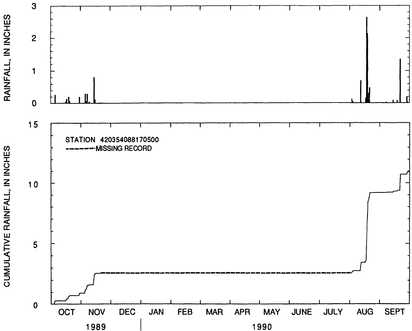
Figure 55.--Daily rainfall totals and cumulative rainfall at Elgin Wastewater Treatment Facility at Elgin, Illinois, water year 1990.
