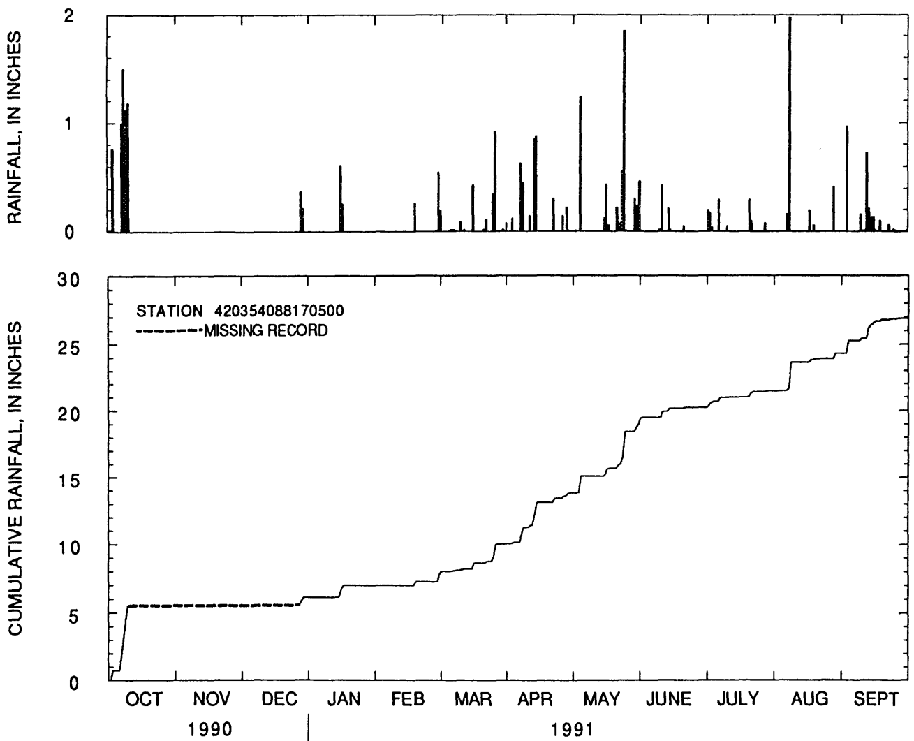
Figure 56.--Daily rainfall totals and cumulative rainfall at Elgin Wastewater Treatment Facility at Elgin, Illinois, water year 1991.
