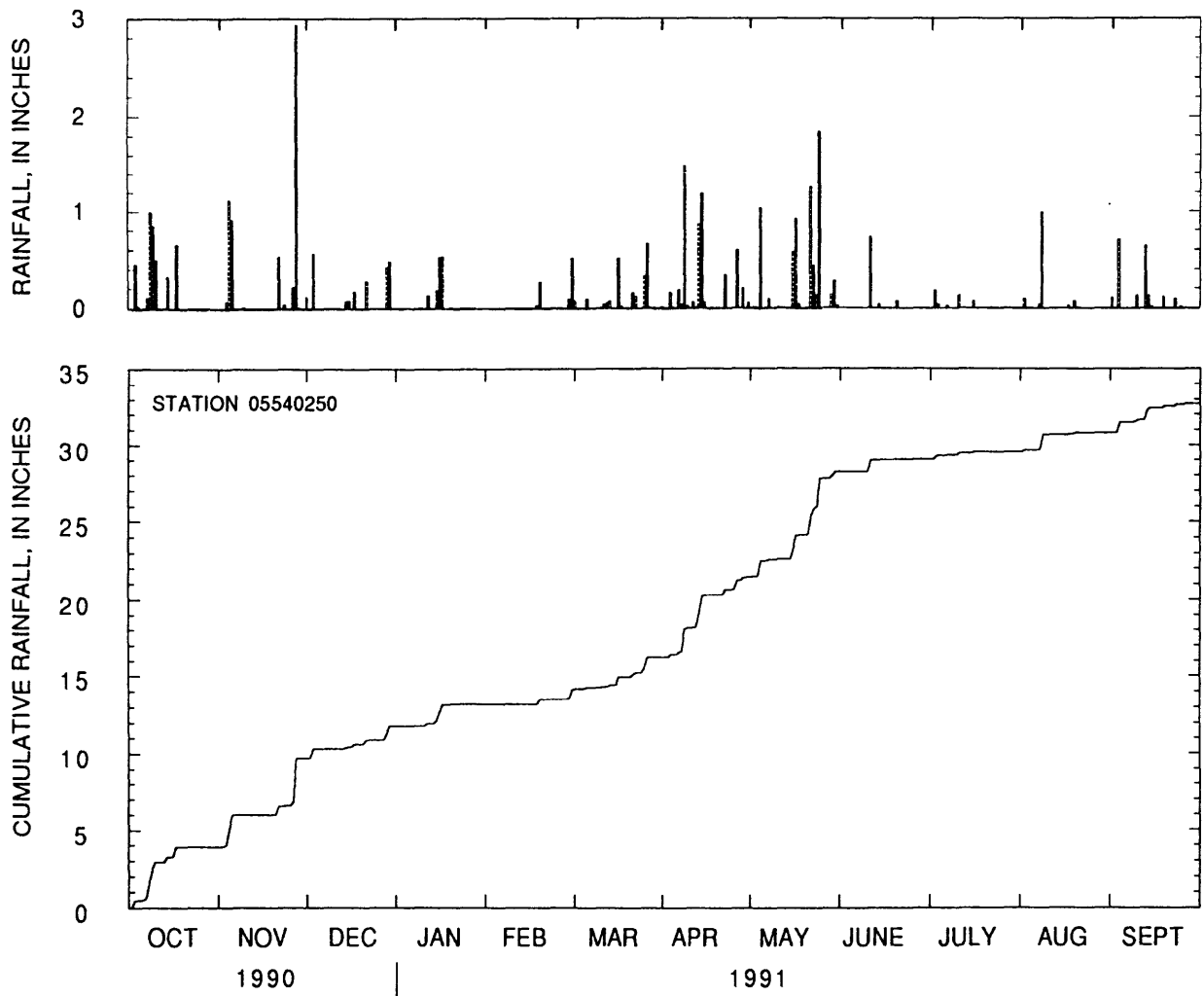
Figure 32.--Daily rainfall totals and cumulative rainfall at East Branch Du Page River at Bolingbrook, Illinois, water year 1991.
