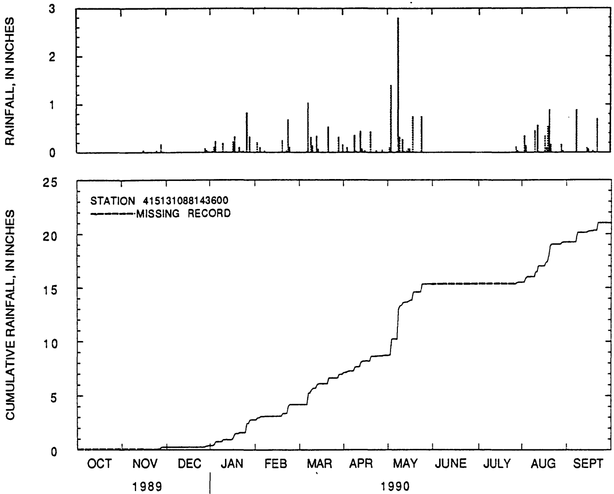
Figure 44.--Daily rainfall totals and cumulative rainfall at National Accelerator Laboratory near West Chicago, Illinois, water year 1990.
