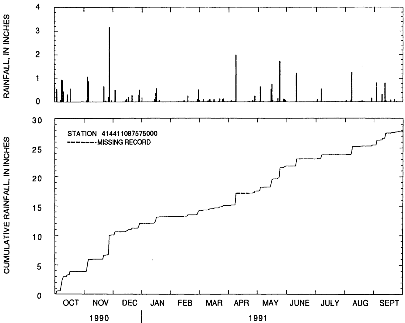
Figure 33.--Daily rainfall totals and cumulative rainfall at Marienbrook Wastewater Treatment Facility at Darien, Illinois, water year 1991.
