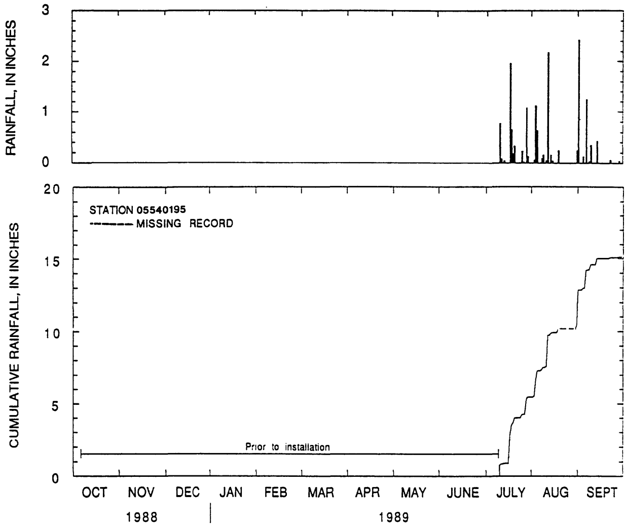
Figure 21.--Daily rainfall totals and cumulative rainfall at St. Joseph Creek at State Highway 34 at Lisle, Illinois, water year 1989.
