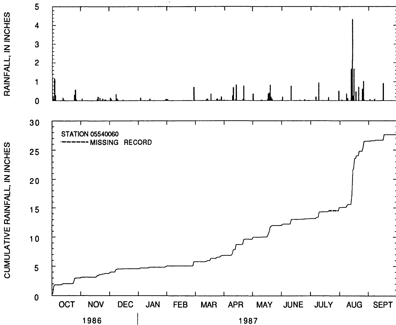
Figure 13.--Daily rainfall totals and cumulative rainfall at Kress Creek at West Chicago, Illinois, water year 1987.
