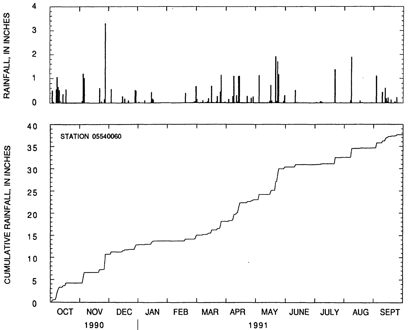
Figure 17.--Daily rainfall totals and cumulative rainfall at Kress Creek at West Chicago, Illinois, water year 1991.
