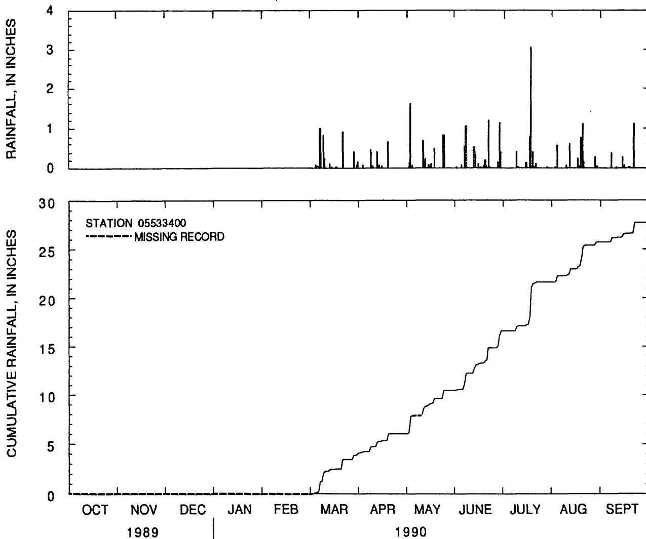
Figure 10.--Daily rainfall totals and cumulative rainfall at Sawmill Creek near Lemont, Illinois, water year 1990.
