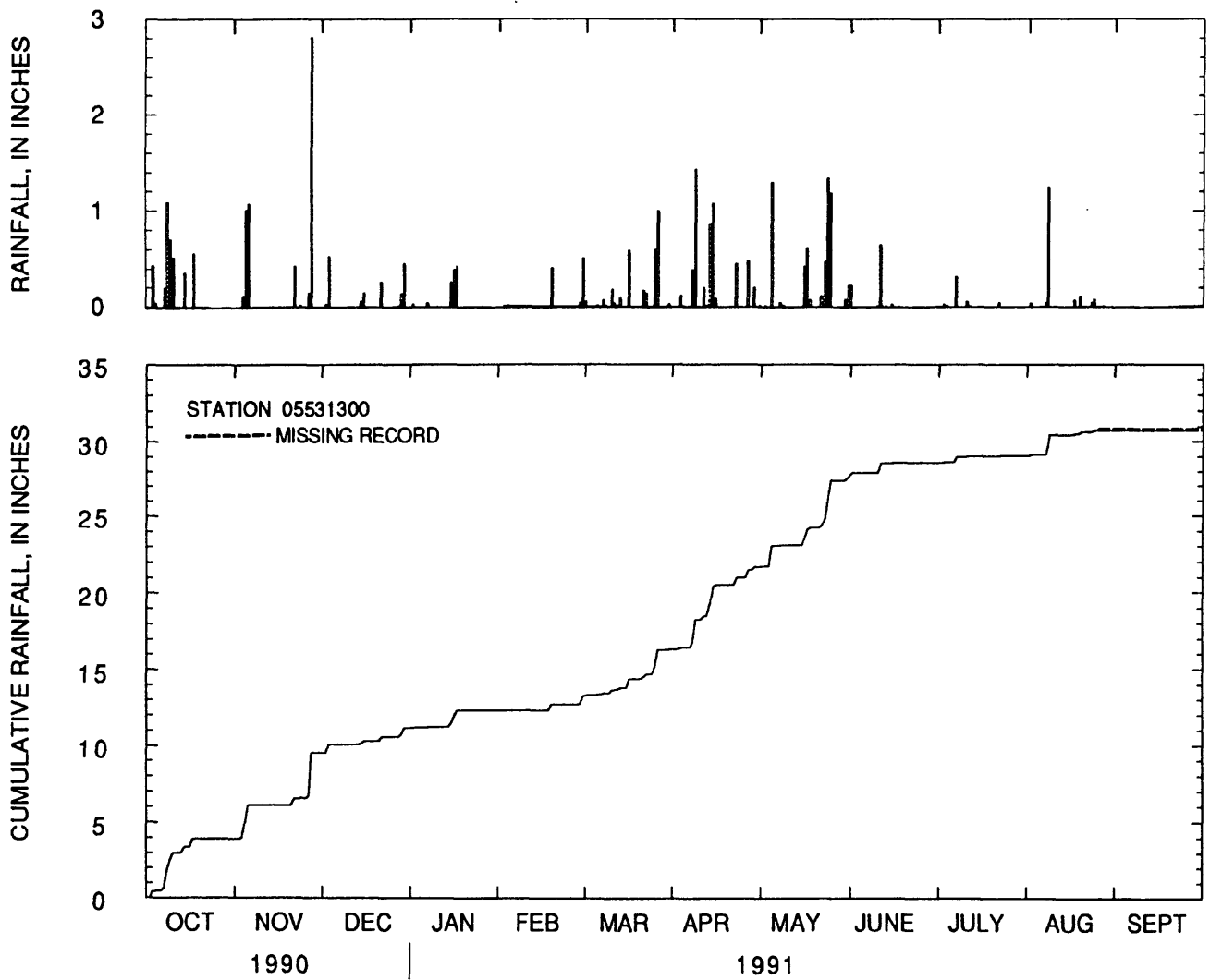
Figure 5.--Daily rainfall totals and cumulative rainfall at Salt Creek at Elmhurst, Illinois, water year 1991.
