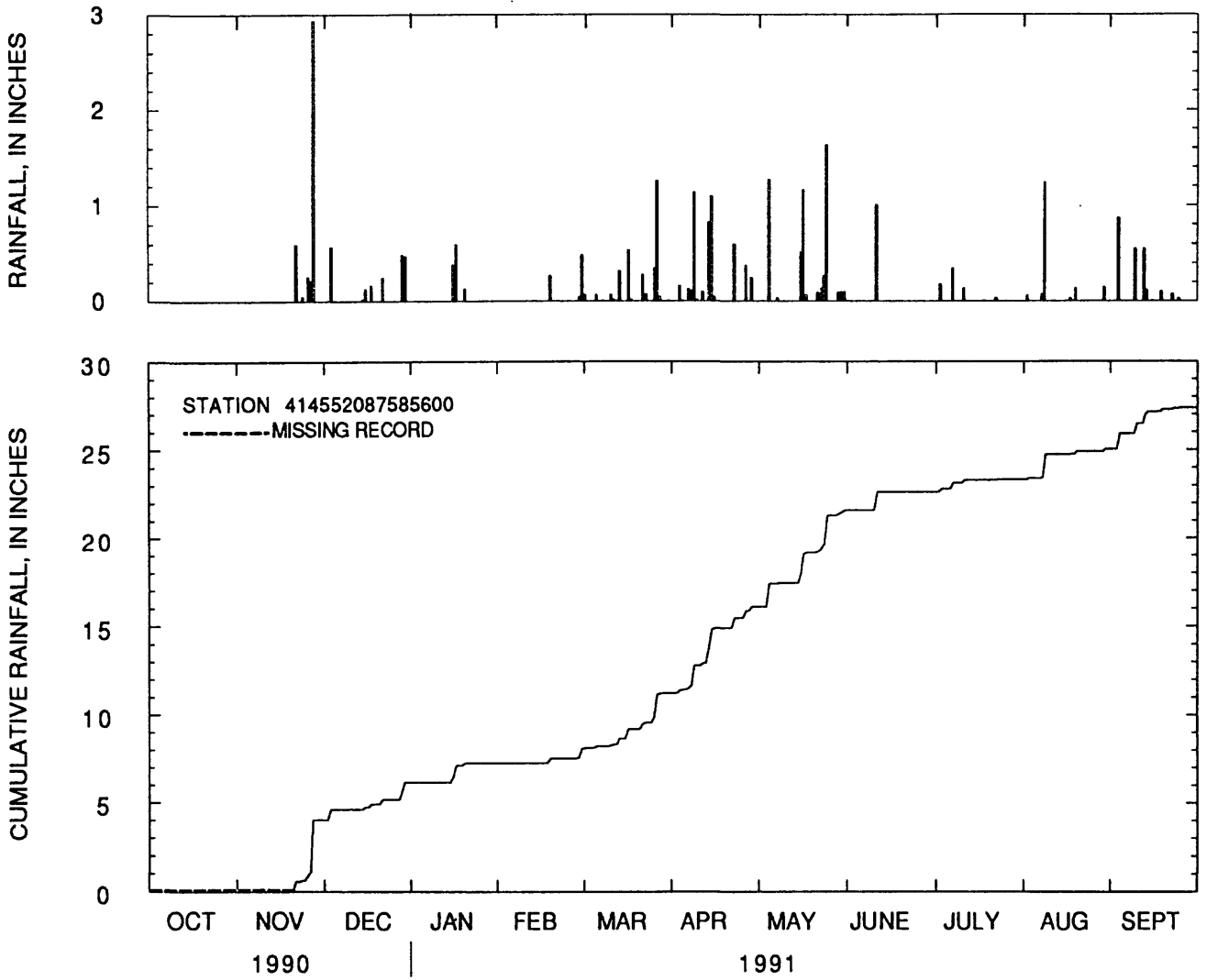
Figure 39.--Daily rainfall totals and cumulative rainfall at Clarendon Hills Cemetery at Darien, Illinois, water year 1991.
