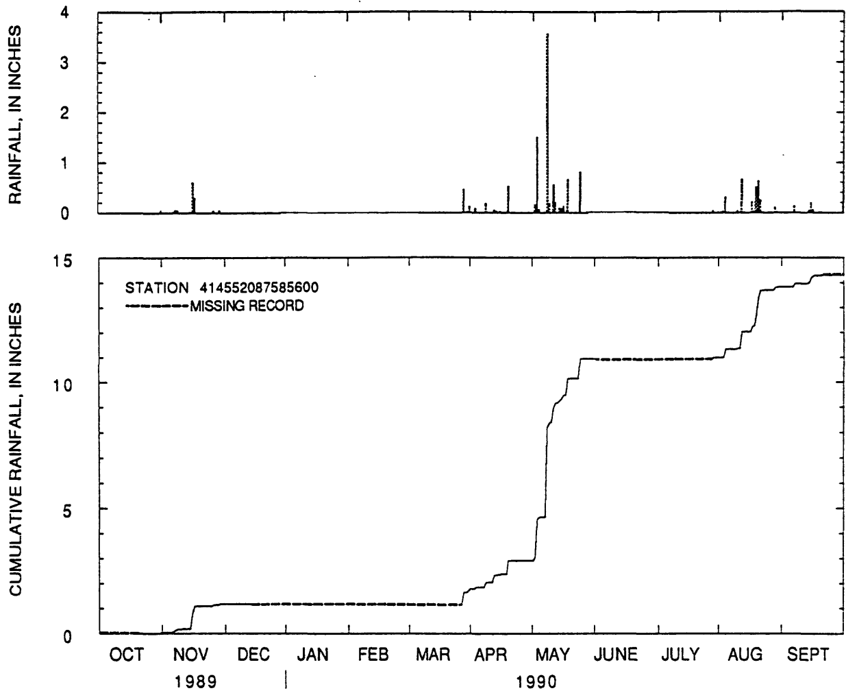
Figure 38.--Daily rainfall totals and cumulative rainfall at Clarendon Hills Cemetery at Darien, Illinois, water year 1990.
