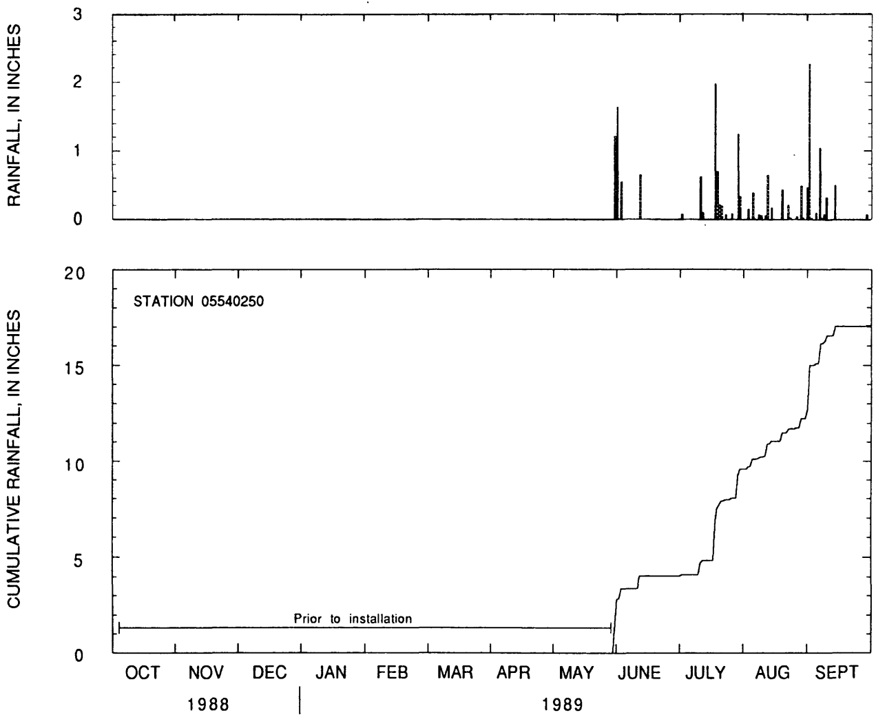
Figure 30.--Daily rainfall totals and cumulative rainfall at East Branch Du Page River at Bolingbrook, Illinois, water year 1989.
