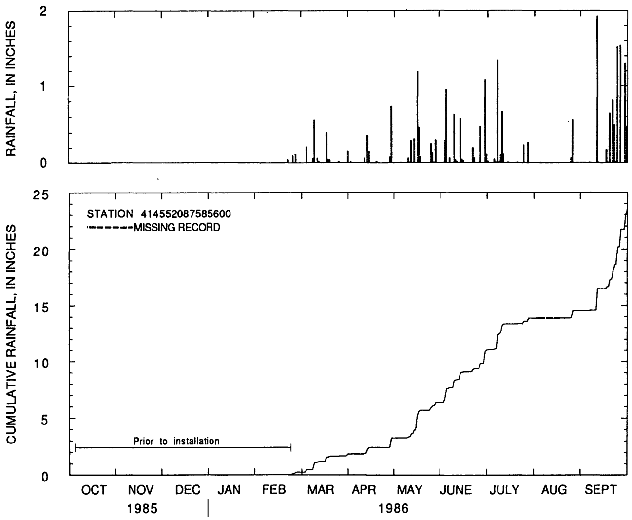
Figure 34.--Daily rainfall totals and cumulative rainfall at Clarendon Hills Cemetery at Darien, Illinois, water year 1986.
