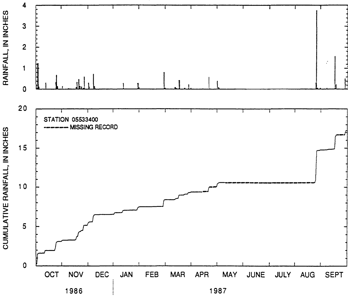
Figure 7.--Daily rainfall totals and cumulative rainfall at Sawmill Creek near Lemont, Illinois, water year 1987.
