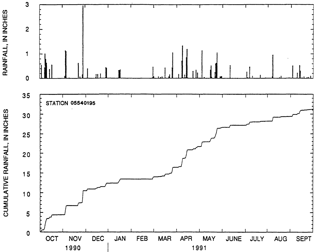
Figure 23.--Daily rainfall totals and cumulative rainfall at St. Joseph Creek at State Highway 34 at Lisle, Illinois, water year 1991.
