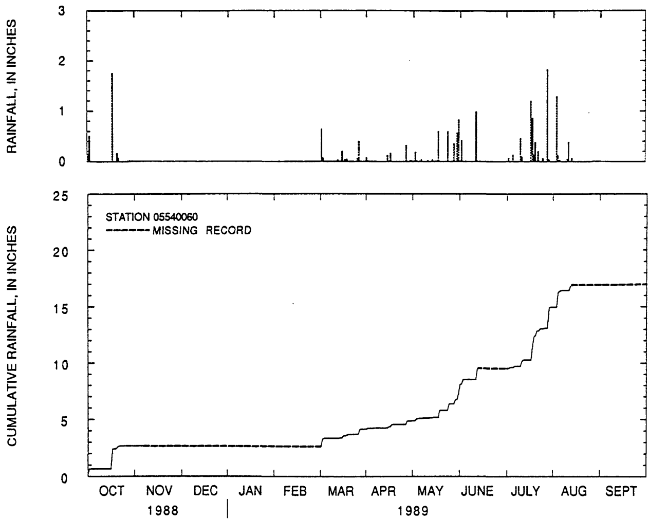
Figure 15.--Daily rainfall totals and cumulative rainfall at Kress Creek at West Chicago, Illinois, water year 1989.
