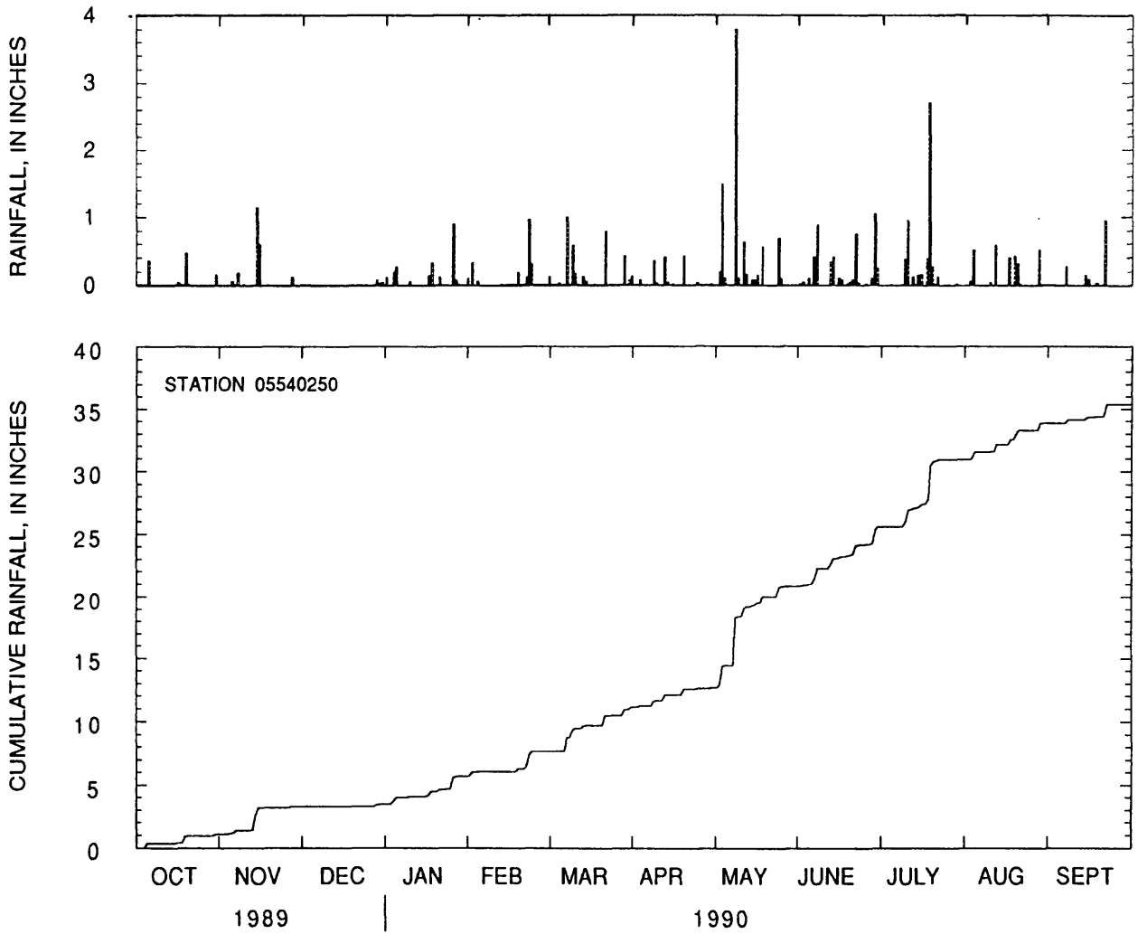
Figure 31.--Daily rainfall totals and cumulative rainfall at East Branch Du Page River at Bolingbrook, Illinois, water year 1990.
