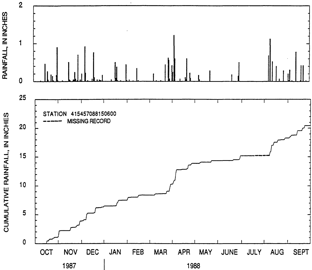
Figure 48.--Daily rainfall totals and cumulative rainfall at Du Page County Airport near St. Charles, Illinois, water year 1988.
