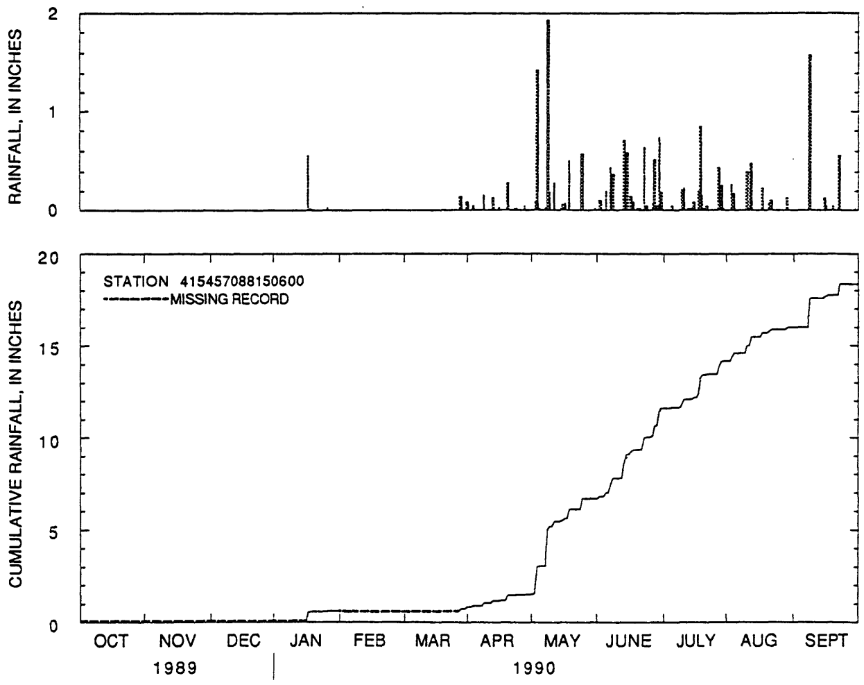
Figure 50.--Daily rainfall totals and cumulative rainfall at Du Page County Airport near St. Charles, Illinois, water year 1990.
