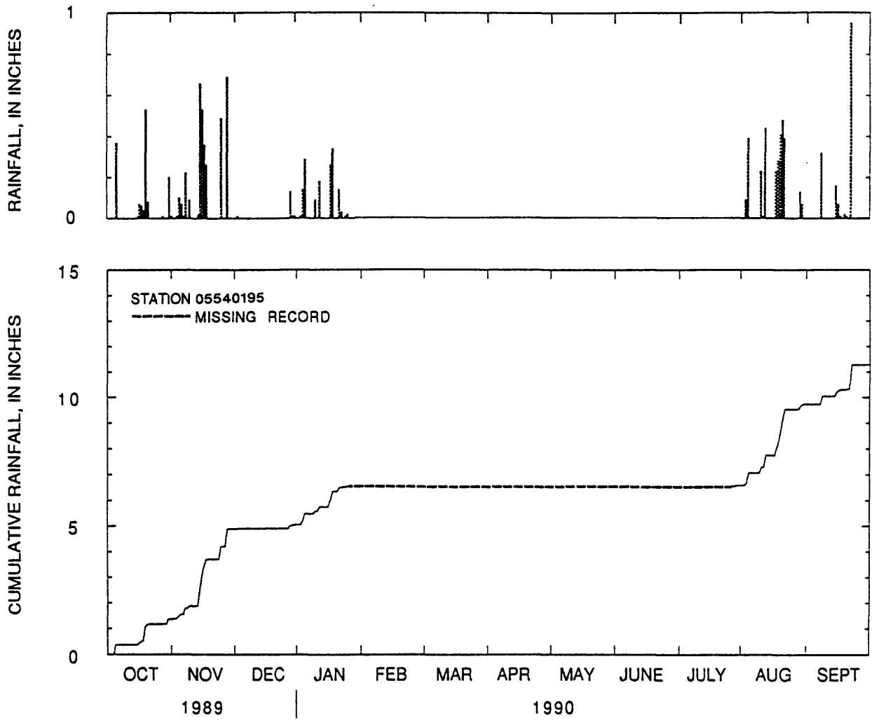
Figure 22.--Daily rainfall totals and cumulative rainfall at St. Joseph Creek at State Highway 34 at Lisle, Illinois, water year 1990.
