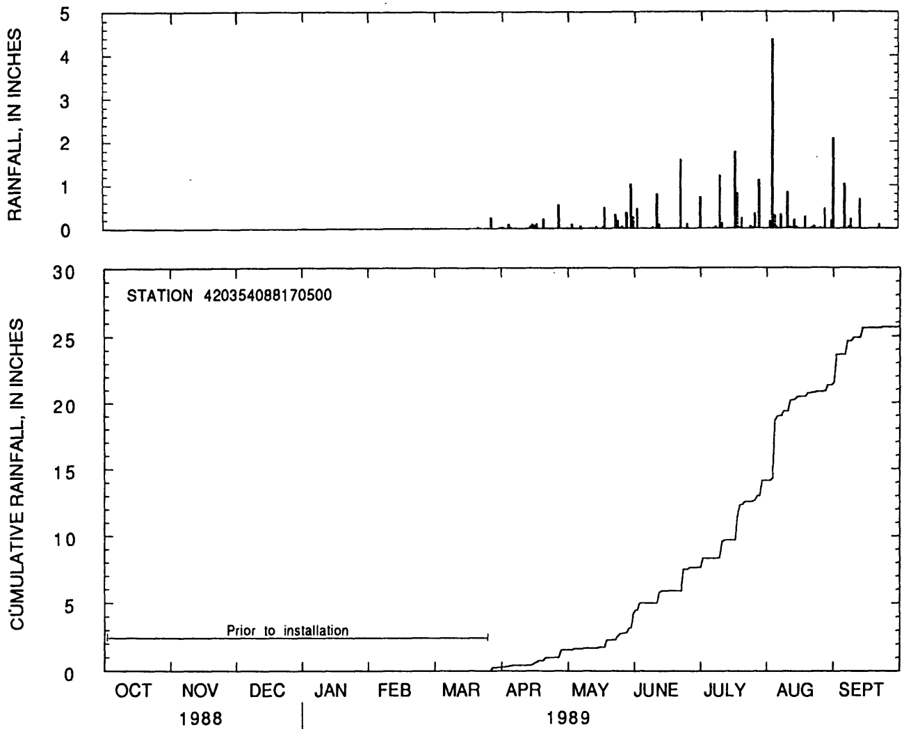
Figure 54.--Daily rainfall totals and cumulative rainfall at Elgin Wastewater Treatment Facility at Elgin, Illinois, water year 1989.
