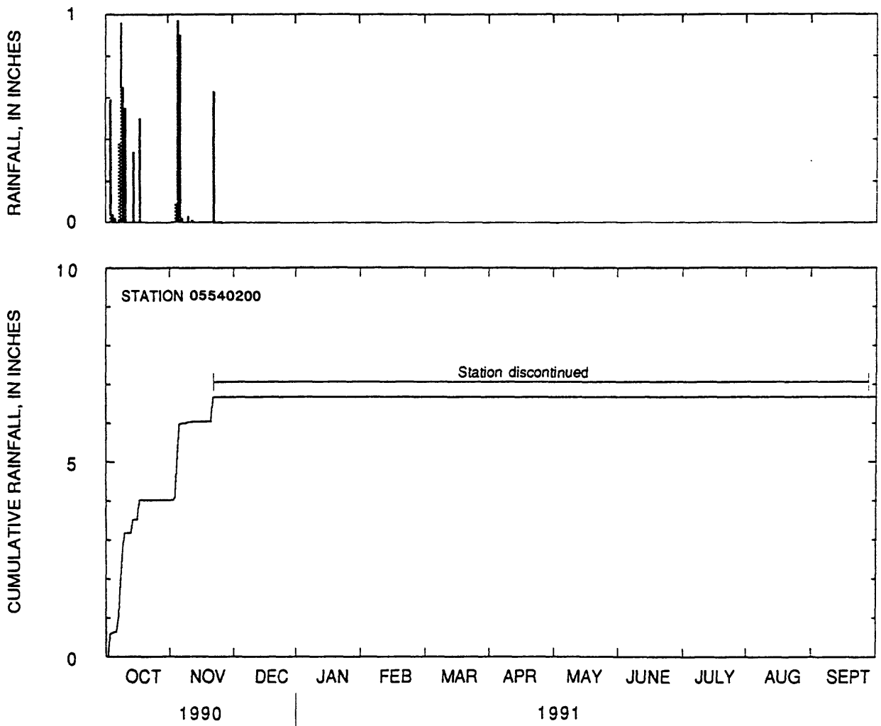
Figure 29.--Daily rainfall totals and cumulative rainfall at St. Joseph Creek at Lisle, Illinois, water year 1991.
