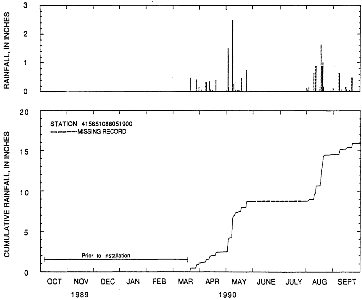
Figure 52.--Daily rainfall totals and cumulative rainfall at Bloomingdale Lift Station at Bloomingdale, Illinois, water year 1990.
