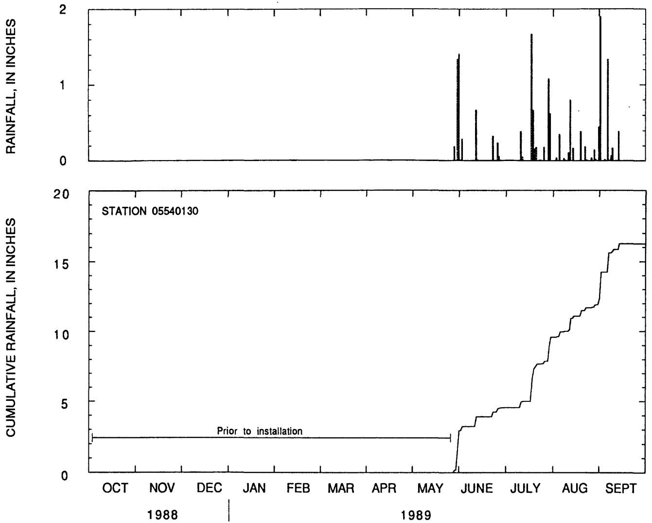
Figure 18.--Daily rainfall totals and cumulative rainfall at West Branch Du Page River near Naperville, Illinois, water year 1989.
