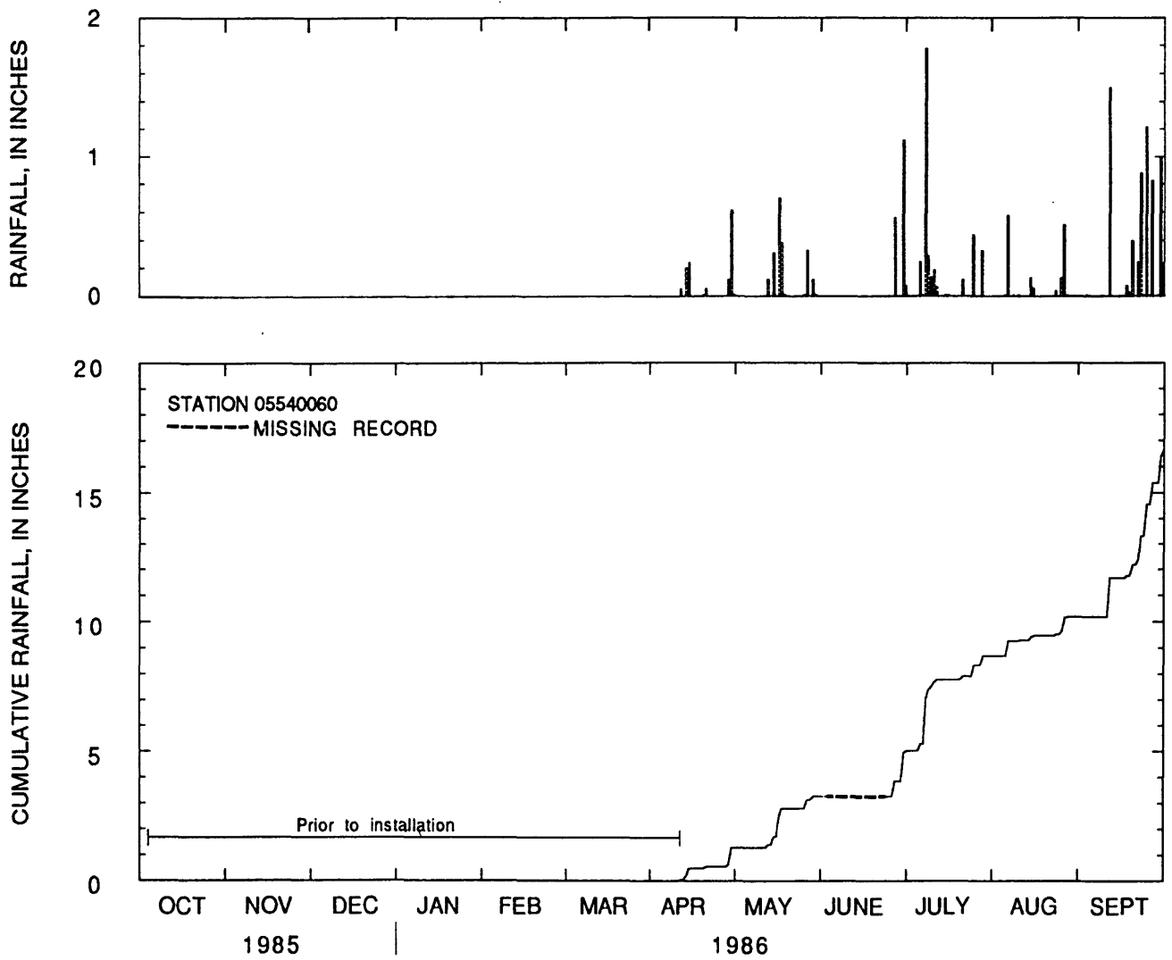
Figure 12.--Daily rainfall totals and cumulative rainfall at Kress Creek at West Chicago, Illinois, water year 1986.
