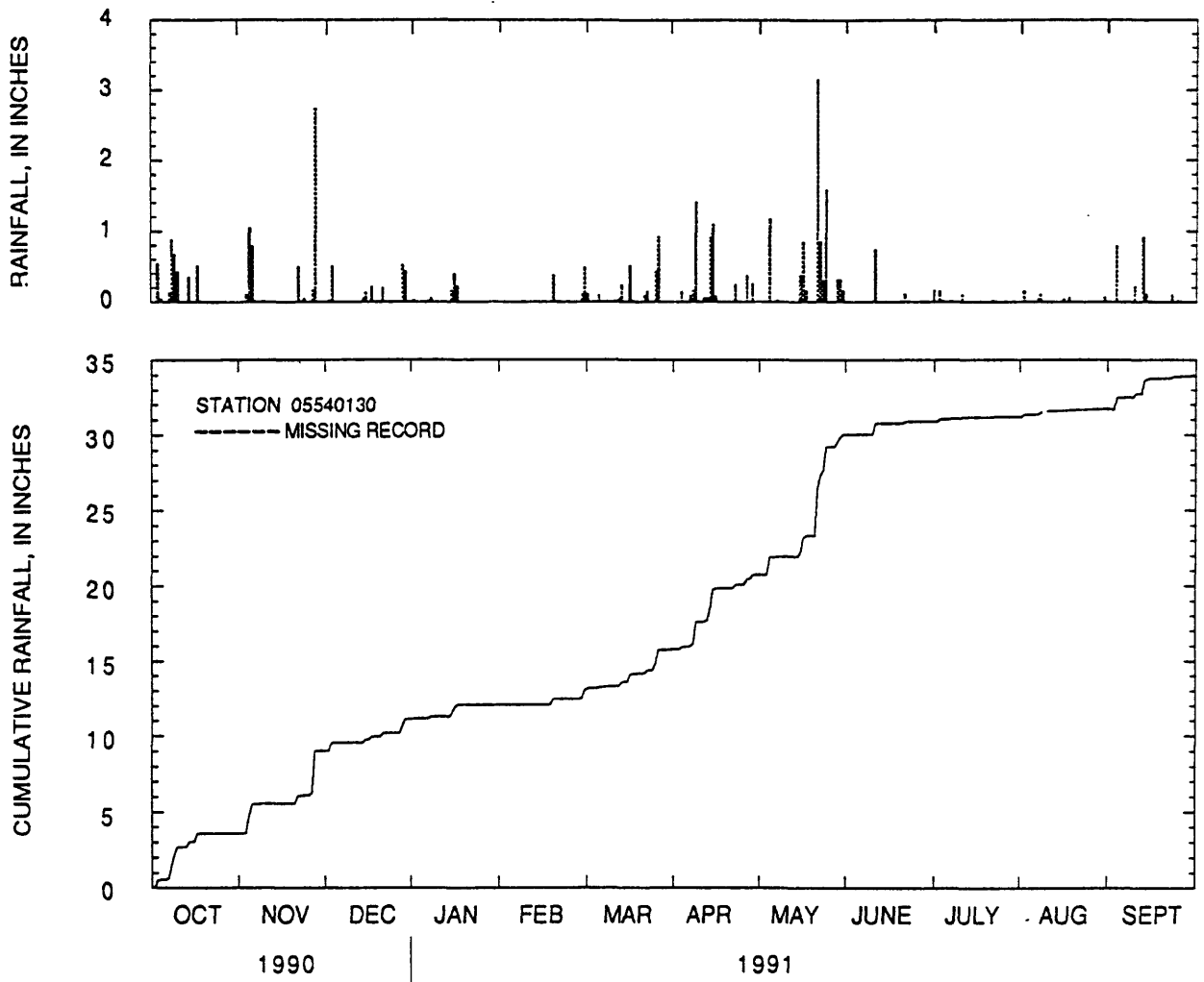
Figure 20.--Daily rainfall totals and cumulative rainfall at West Branch Du Page River near Naperville, Illinois, water year 1991.
