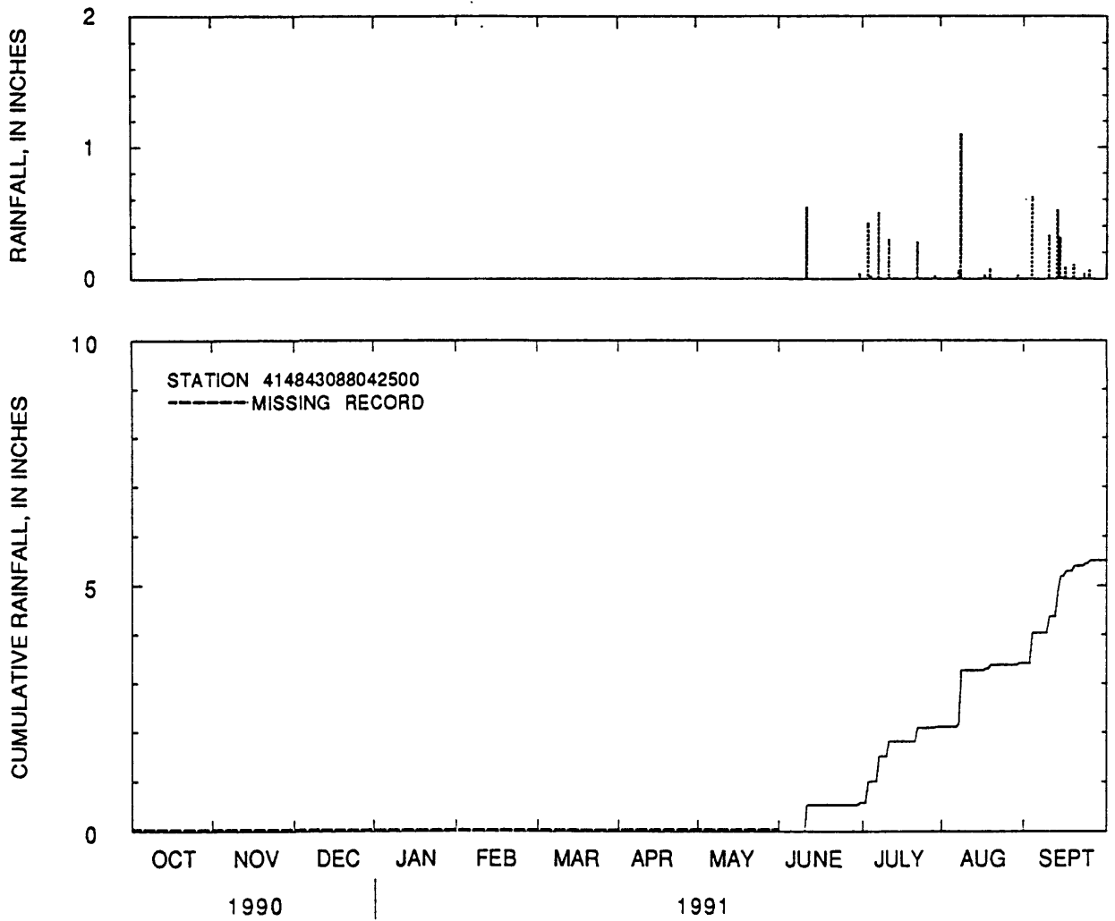
Figure 42.--Daily rainfall totals and cumulative rainfall at Morton Arboretum near Lisle, Illinois, water year 1991.
