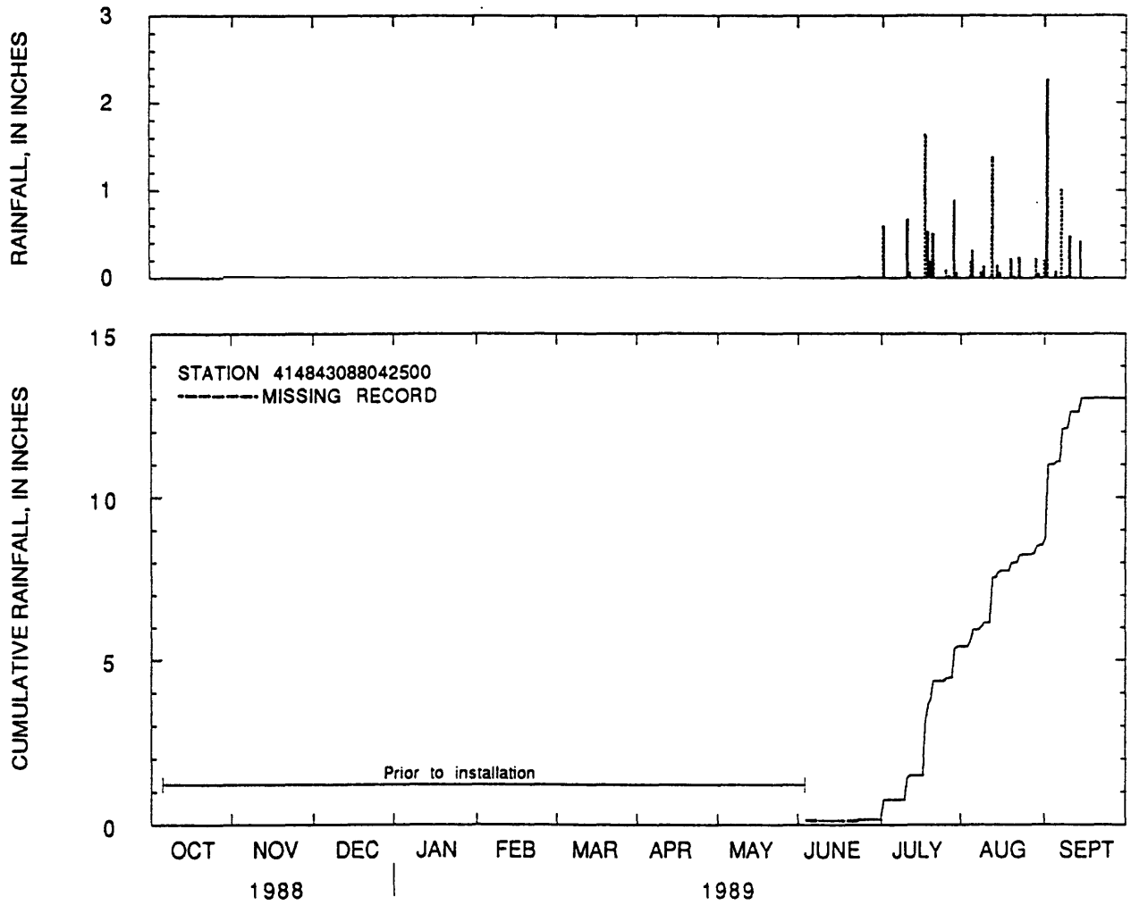
Figure 40.--Daily rainfall totals and cumulative rainfall at Morton Arboretum near Lisle, Illinois, water year 1989.
