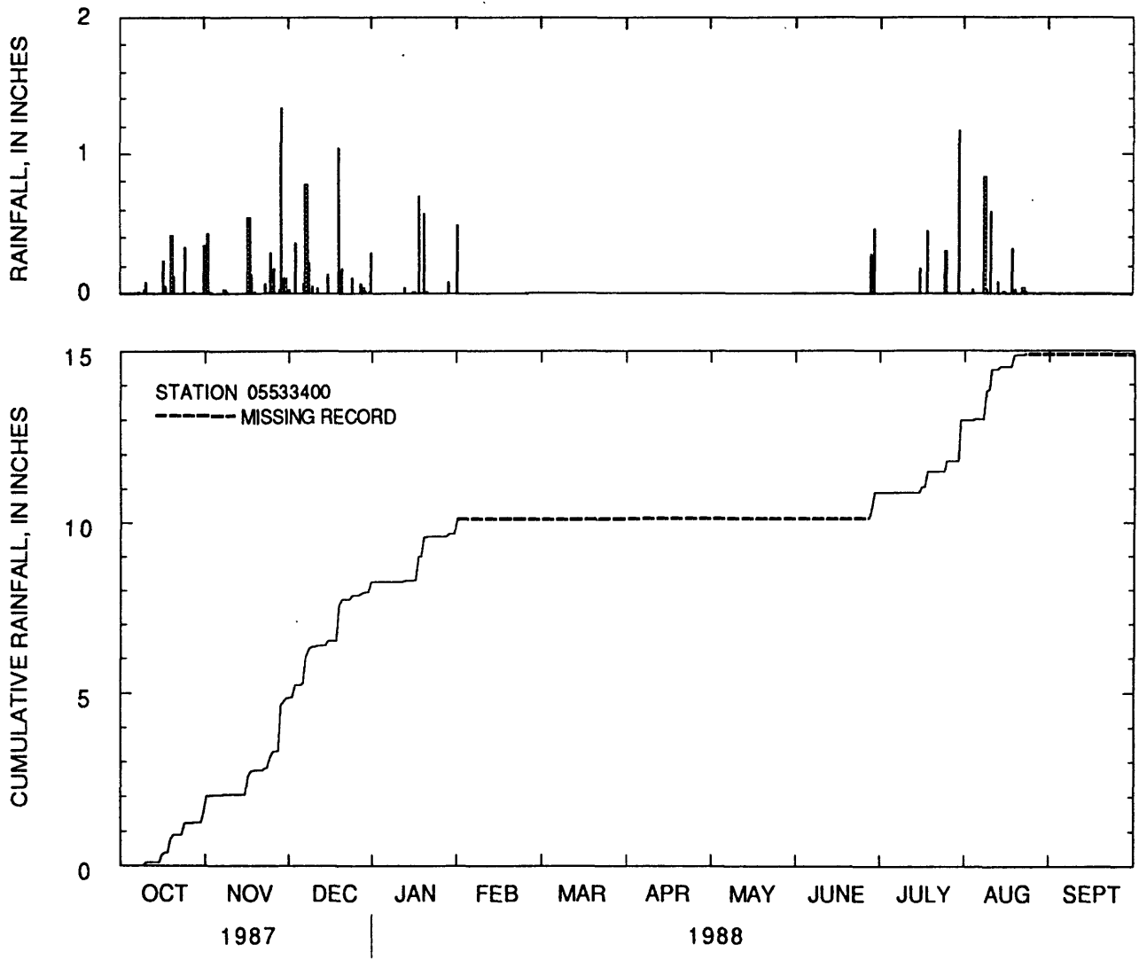
Figure 8.--Daily rainfall totals and cumulative rainfall at Sawmill Creek near Lemont, Illinois, water year 1988.
