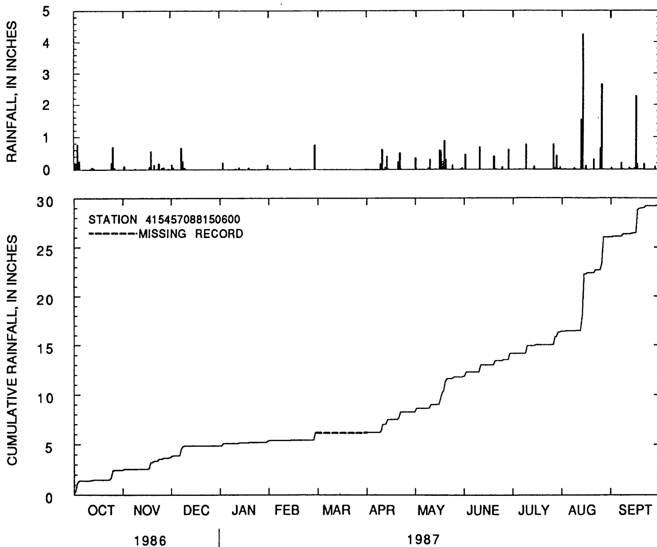
Figure 47.--Daily rainfall totals and cumulative rainfall at Du Page County Airport near St. Charles, Illinois, water year 1987.
