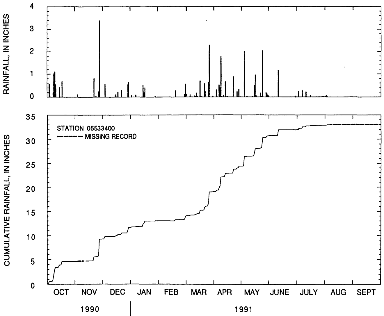
Figure 11.--Daily rainfall totals and cumulative rainfall at Sawmill Creek near Lemont, Illinois, water year 1991.
