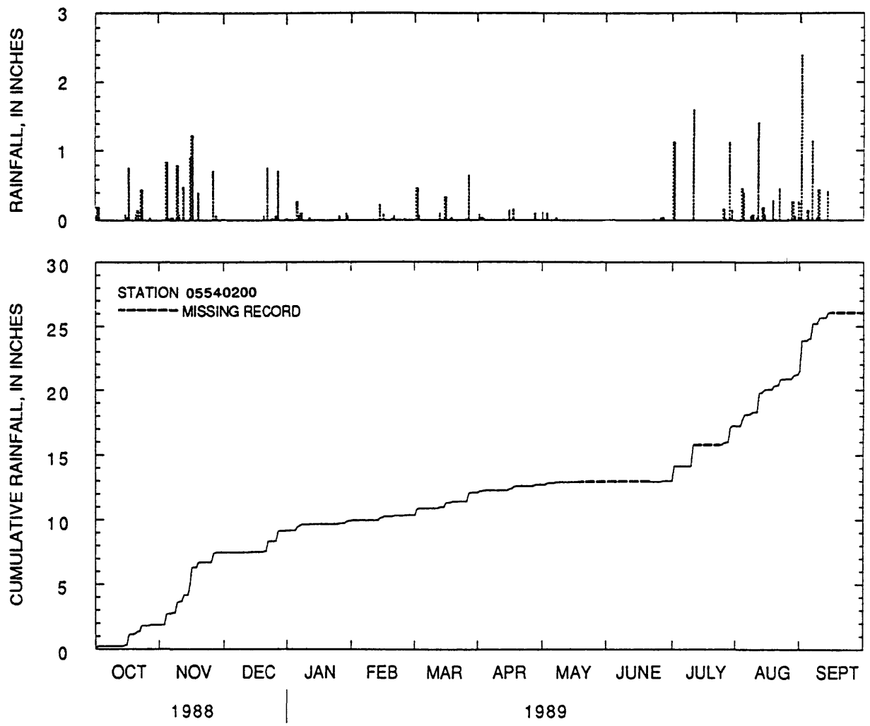
Figure 27.--Daily rainfall totals and cumulative rainfall at St. Joseph Creek at Lisle, Illinois, water year 1989.
