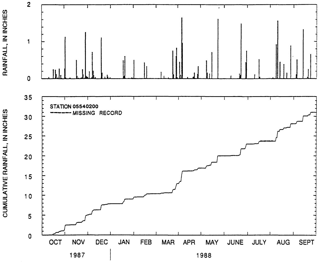
Figure 26.--Daily rainfall totals and cumulative rainfall at St. Joseph Creek at Lisle, Illinois, water year 1988.
