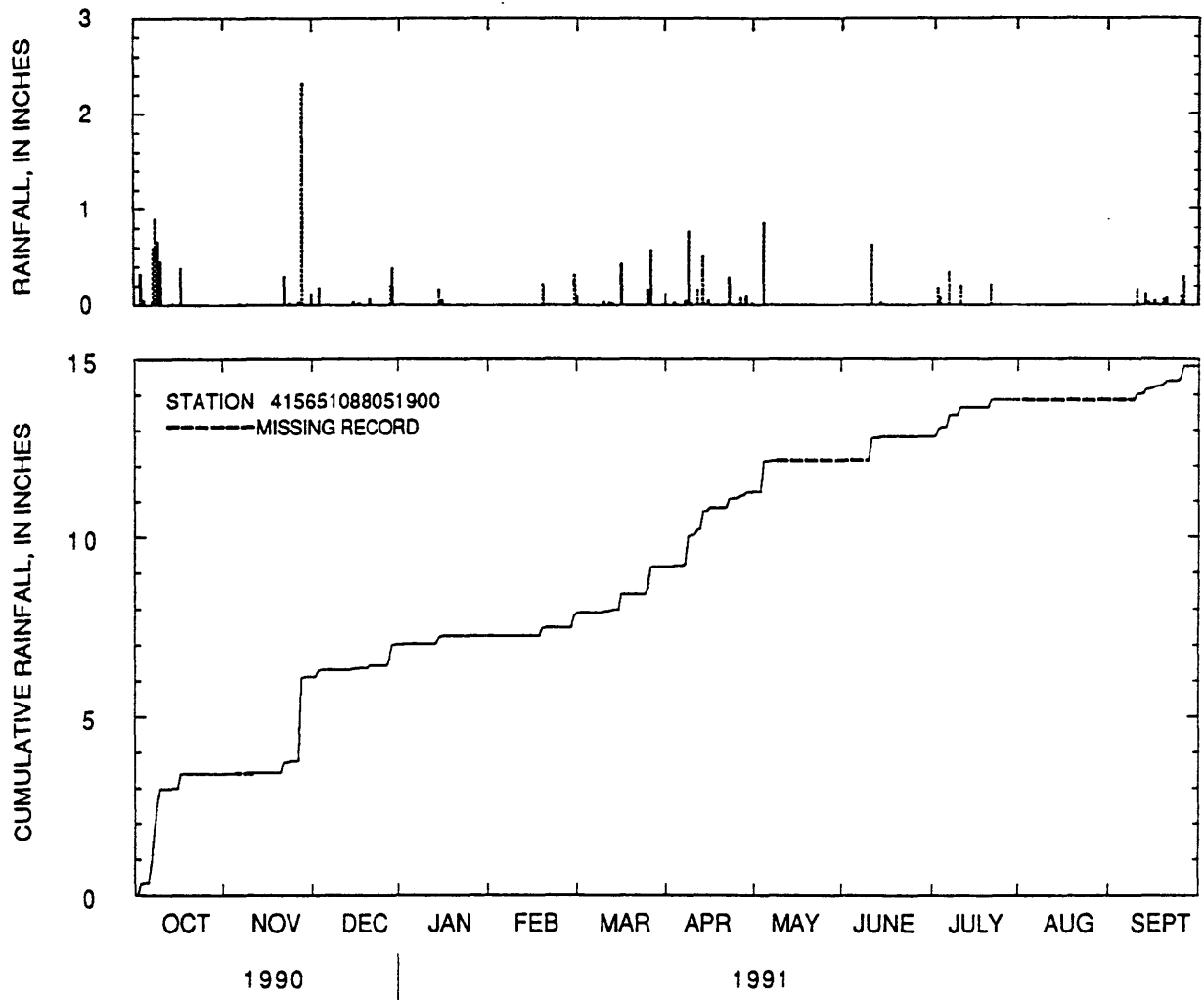
Figure 53.--Daily rainfall totals and cumulative rainfall at Bloomingdale Lift Station at Bloomingdale, Illinois, water year 1991.
