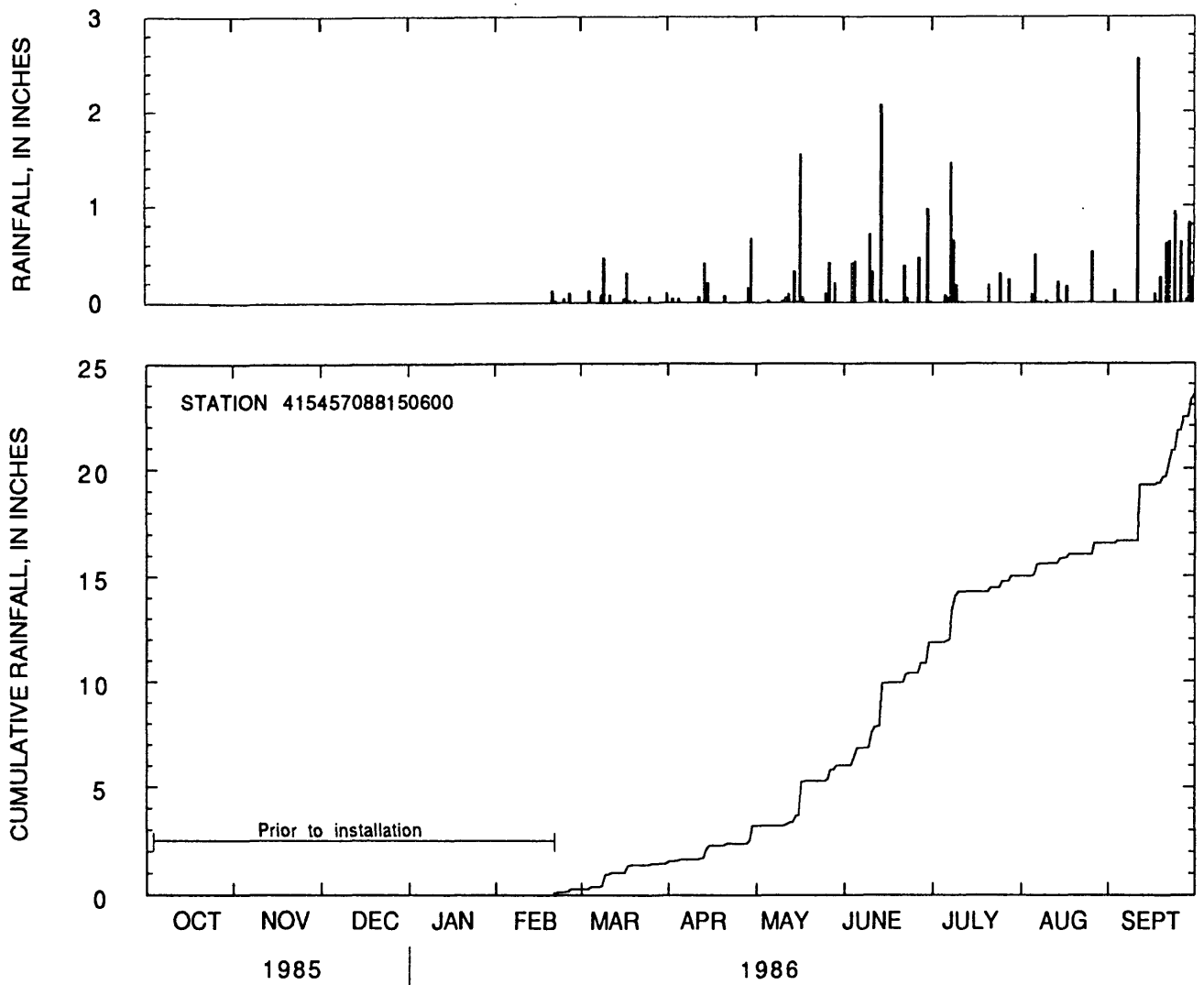
Figure 46.--Daily rainfall totals and cumulative rainfall at Du Page County Airport near St. Charles, Illinois, water year 1986.
