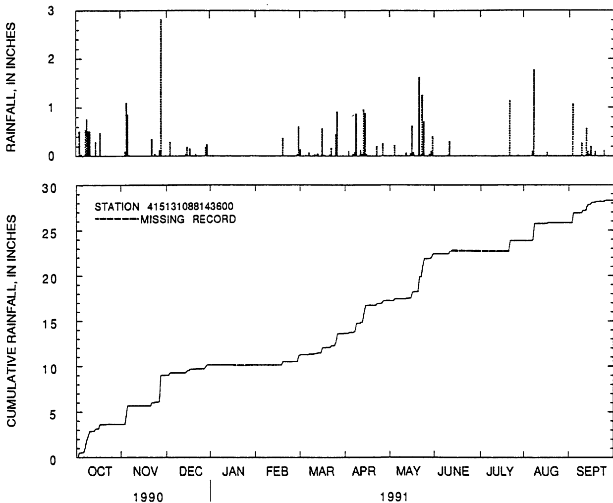
Figure 45.--Daily rainfall totals and cumulative rainfall at National Accelerator Laboratory near West Chicago, Illinois, water year 1991.
