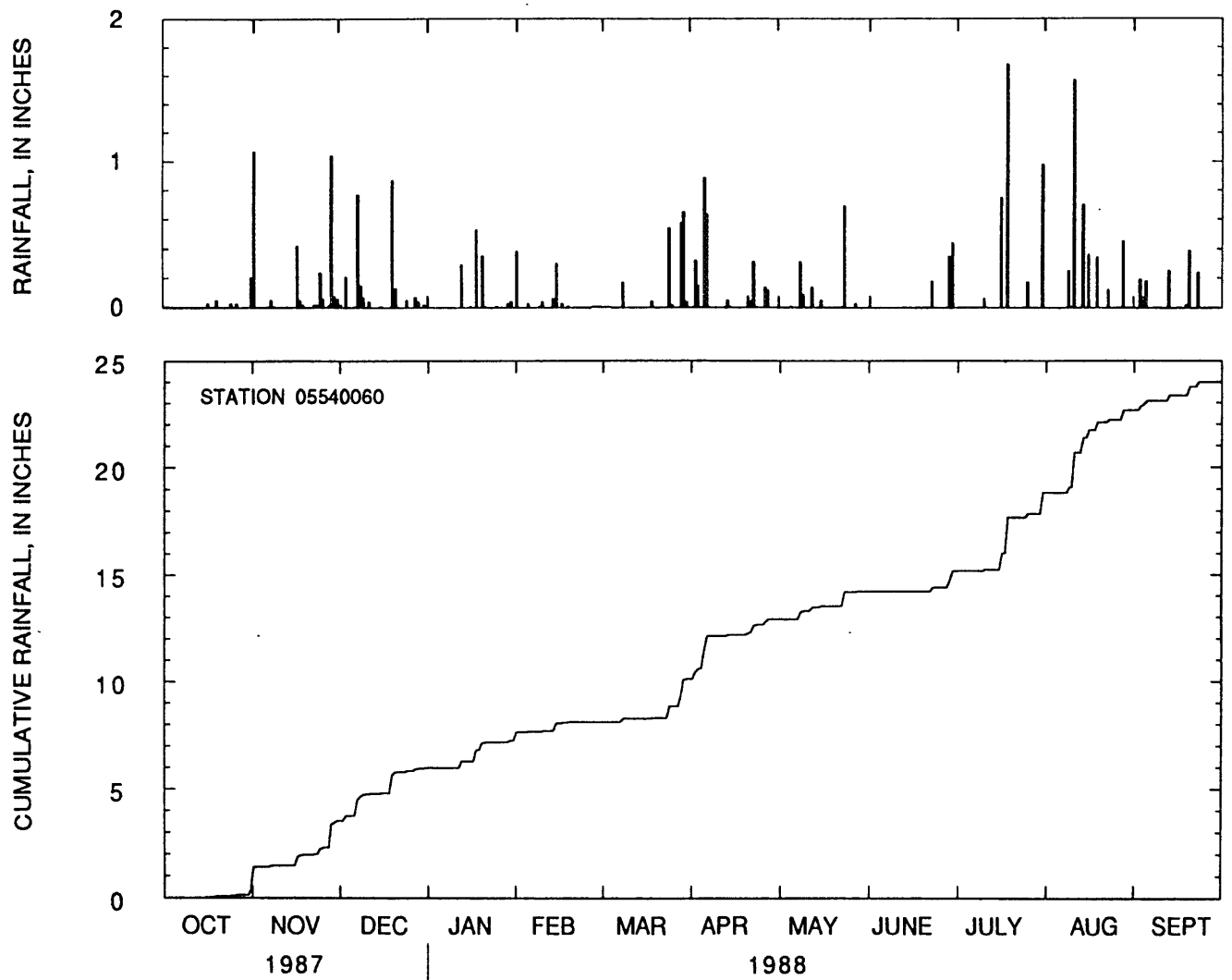
Figure 14.--Daily rainfall totals and cumulative rainfall at Kress Creek at West Chicago, Illinois, water year 1988.
