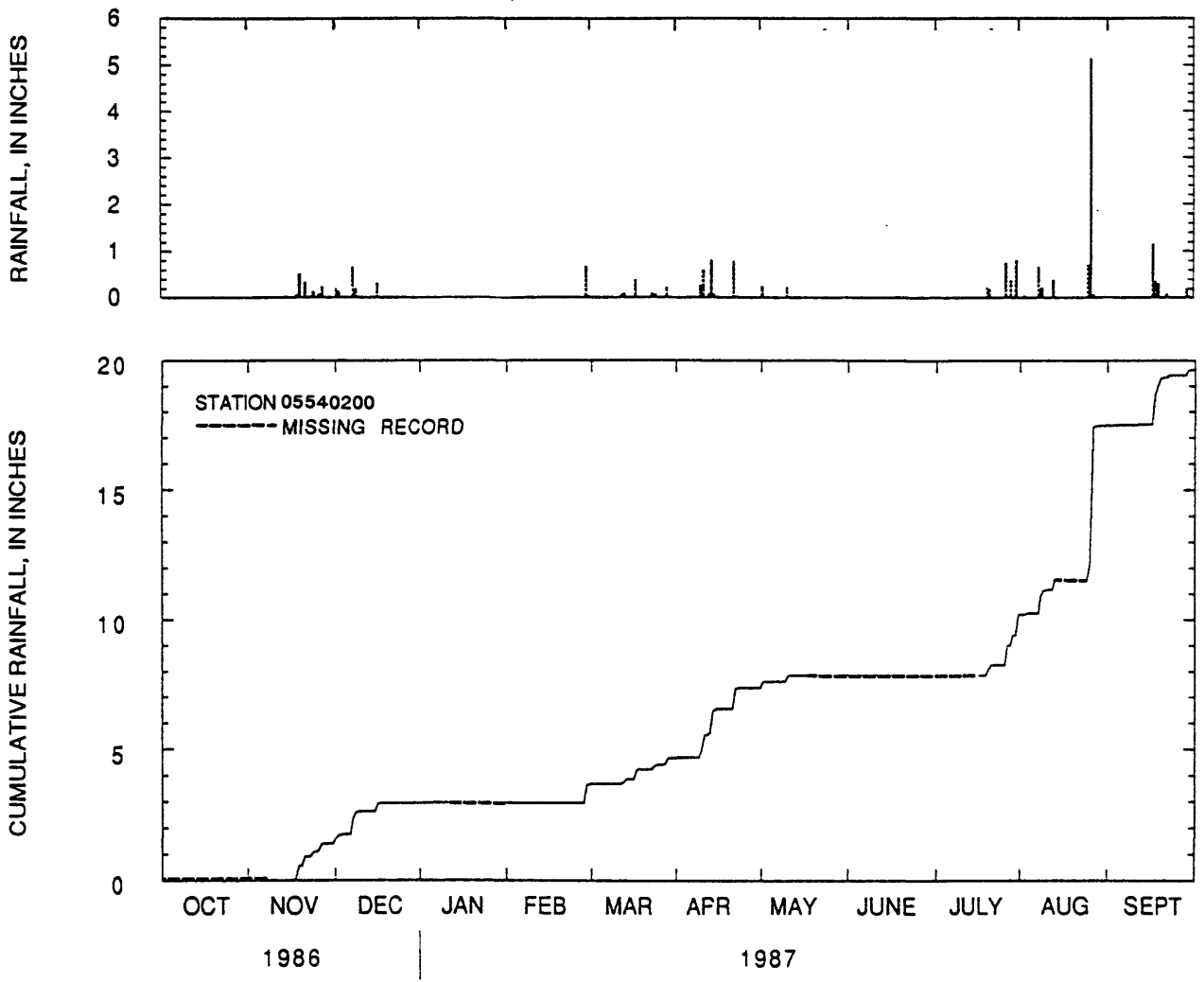
Figure 25.--Daily rainfall totals and cumulative rainfall at St. Joseph Creek at Lisle, Illinois, water year 1987.
