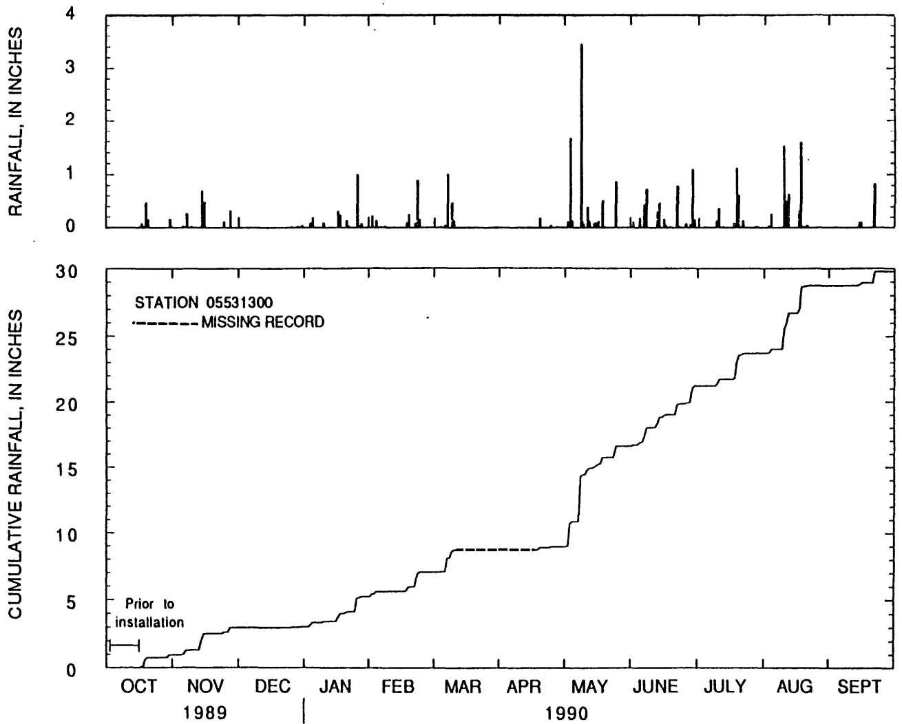
Figure 4.--Daily rainfall totals and cumulative rainfall at Salt Creek at Elmhurst, Illinois, water year 1990.
